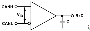
Figure 23. Receiver Voltage Measurements
