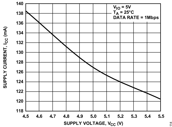
Figure 19. Supply Current, I_{CC} vs. Supply Voltage V_{CC}
