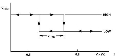
Figure 3. Receiver Input Hysteresis
