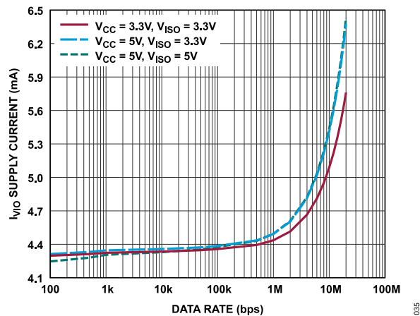
Figure 35. V_{IO} Supply Current vs. Data Rate, T_A = 25^\circ\text{C} , (ADM2895E-1), 54Ω termination, Logarithmic Scale
