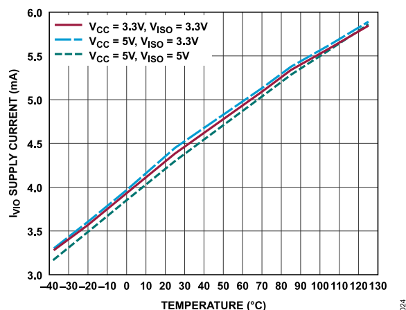
Figure 24. V_{IO} Supply Current vs. Temperature at 250kbps (ADM2895E), Unterminated Bus
