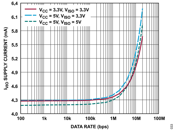
Figure 33. V_{IO} Supply Current vs. Data Rate, T_A = 25^\circ\text{C} , (ADM2895E-1), Unterminated Bus, Logarithmic Scale
