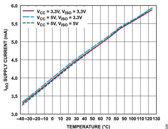
Figure 26. V_{IO} Supply Current vs. Temperature at 250kbps (ADM2895E), 54\Omega Termination
