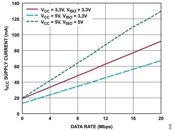
Figure 18. V_{CC} Supply Current vs. Frequency, T_A = 25^\circ\text{C} , (ADM2895E-1), Underterminated Bus, Linear Scale
