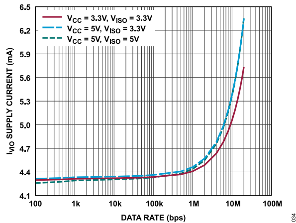
Figure 34. V_{IO} Supply Current vs. Data Rate, T_A = 25^\circ\text{C} , (ADM2895E-1), 120Ω Termination, Logarithmic Scale
