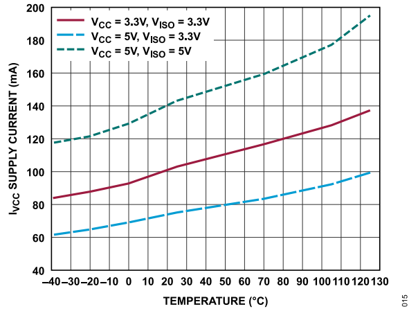
Figure 15. V_{CC} Supply Current vs. Temperature at 20Mbps (ADM2895E-1), Underterminated Bus
