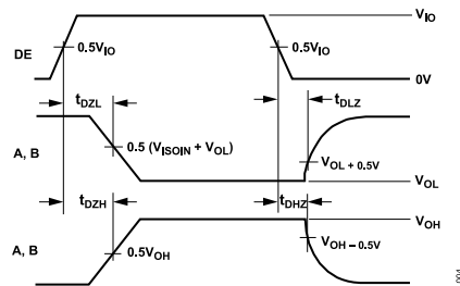
Figure 4. Driver Enable or Disable Timing
