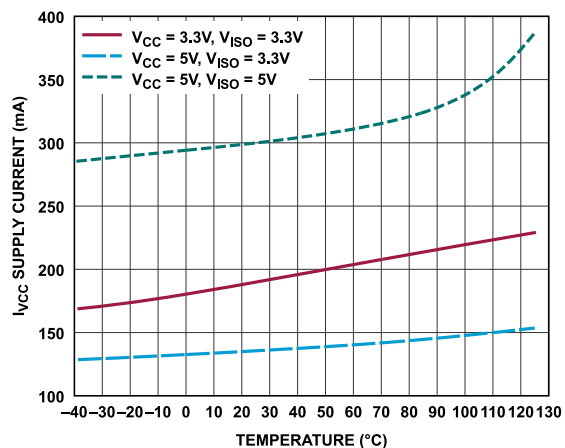
Figure 17. V_{CC} Supply Current vs. Temperature at 20Mbps (ADM2895E-1), 54Ω Termination
