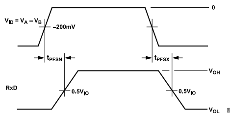
Figure 6. Fail-Safe Entry or Exit Delay Timing
