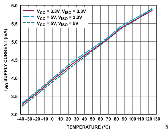
Figure 25. V_{IO} Supply Current vs. Temperature at 250kbps (ADM2895E), 120\Omega Termination
