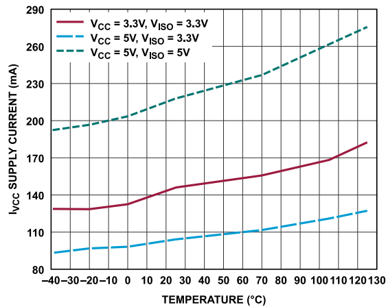
Figure 16. V_{CC} Supply Current vs. Temperature at 20Mbps (ADM2895E-1), 120Ω Termination
