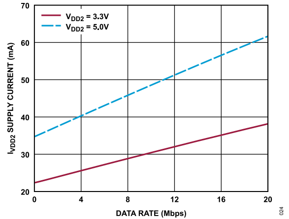
Figure 24. V_{DD2} Supply Current vs. Data Rate, T_A = 25^\circ\text{C} (ADM2495E-1), 120\Omega Termination, Linear Scale
