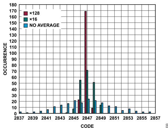
Figure 33. ADC Code Histogram ( V_{SENSE} = 10 mV, 200 Measurements)
