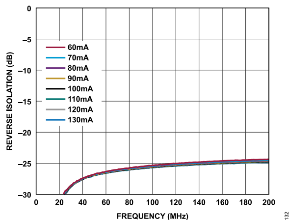
Figure 32. Reverse Isolation vs. Frequency for Various I_{DQ} Values, 10MHz to 200MHz, V_{DD} = 5\text{V}
