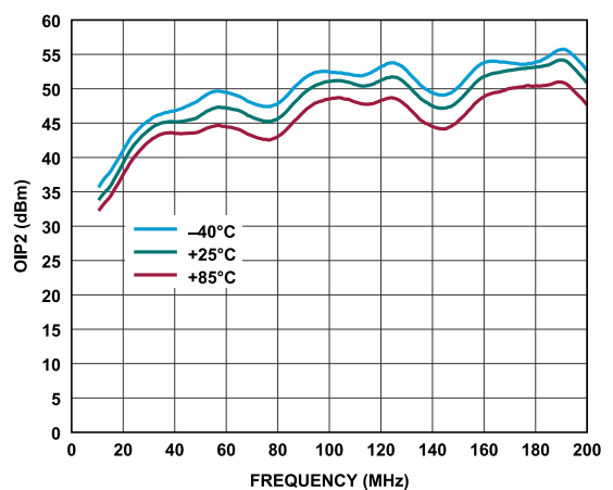
Figure 73. OIP2 vs. Frequency for Various Temperatures, 10MHz to 200MHz, V_{DD} = 5\text{V} , I_{DQ} = 110\text{mA}
