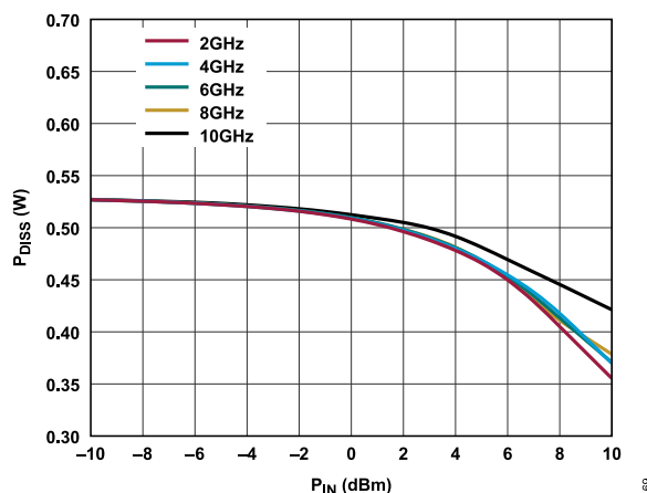
Figure 69. P_{DISS} vs. P_{IN} at T_{CASE} = 85^{\circ}C , V_{DD} = 5V
