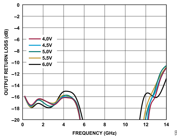
Figure 33. Output Return Loss vs. Frequency for Various Supply Voltages, 200MHz to 14GHz, I_{DQ} = 110\text{mA}
