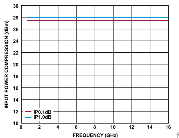
Figure 96. Input Power Compression vs. Frequency for Various Compressions, 1GHz to 16GHz, Mode = Internal, External Bypass A, and External Bypass B
