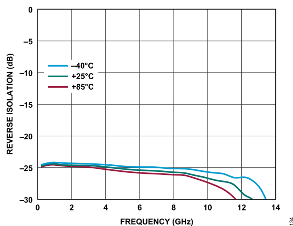
Figure 34. Reverse Isolation vs. Frequency for Various Temperatures, 200MHz to 14GHz, V_{DD} = 5\text{V} , I_{DQ} = 110\text{mA}
