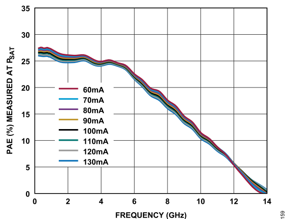
Figure 59. PAE Measured at P_{SAT} vs. Frequency for Various I_{DQ} Values, 200MHz to 14GHz, V_{DD} = 5V
