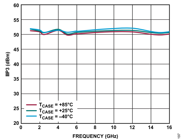
Figure 97. IIP3 vs. Frequency for Various Temperatures, 1GHz to 16GHz, Mode = Internal Bypass, External Bypass A, and External Bypass B
