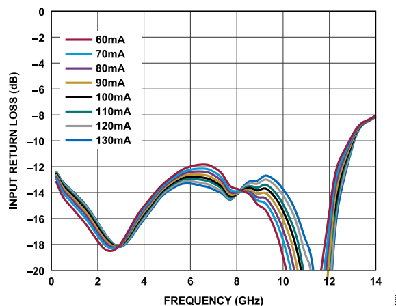
Figure 23. Input Return Loss vs. Frequency for Various I_{DQ} Values, 200MHz to 14GHz, V_{DD} = 5V
