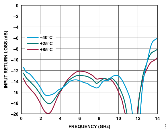
Figure 22. Input Return Loss vs. Frequency for Various Temperatures, 200MHz to 14GHz, V_{DD} = 5V , I_{DQ} = 110mA
