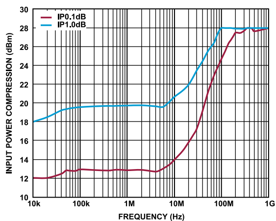
Figure 93. Input Power Compression vs. Frequency for Various Compressions, 10kHz to 1GHz, Mode = Internal Bypass, External Bypass A, and External Bypass B
