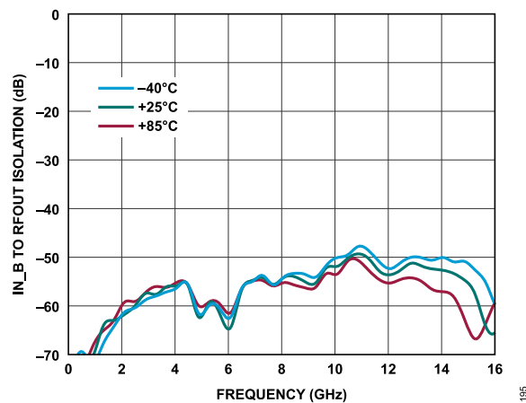
Figure 95. IN_B to RFOUT Isolation vs. Frequency for Various Temperatures, 10MHz to 16GHz
