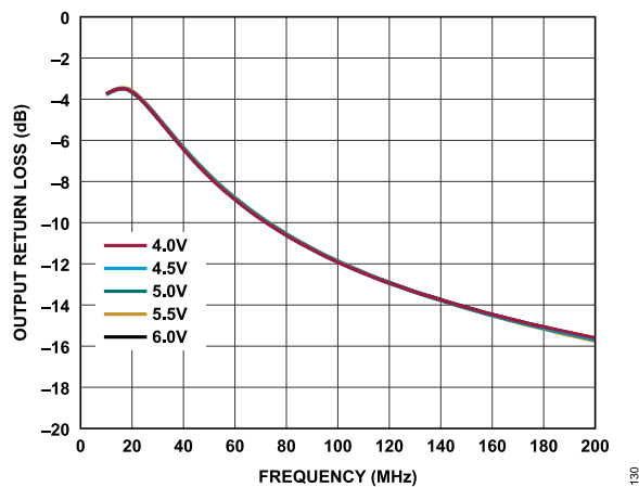
Figure 30. Output Return Loss vs. Frequency for Various Supply Voltages, 10MHz to 200MHz, I_{DQ} = 110\text{mA}
