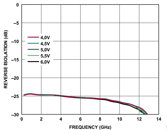
Figure 39. Reverse Isolation vs. Frequency for Various Supply Voltages, 200MHz to 14GHz, I_{DQ} = 110\text{mA}
