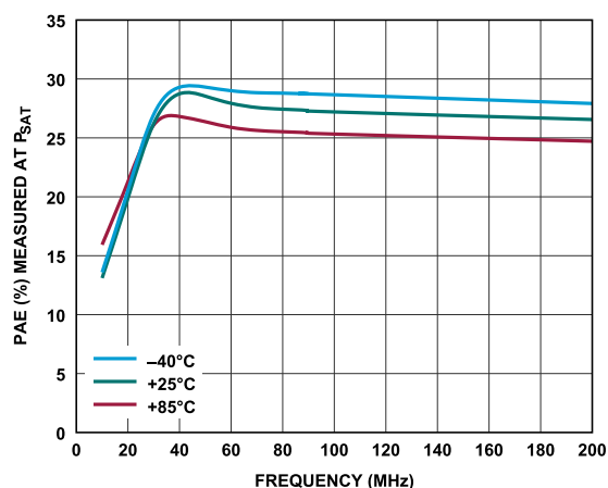
Figure 55. Power Added Efficiency (PAE) Measured at P_{SAT} vs. Frequency for Various Temperatures, 10MHz to 200MHz, V_{DD} = 5V , I_{DQ} = 110mA
