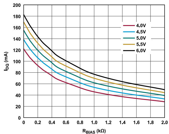
Figure 80. I_{DQ} vs. Bias Resistor Signal ( R_{BIAS} ) for Various Supply Voltages, 0Ω to 2.0kΩ
