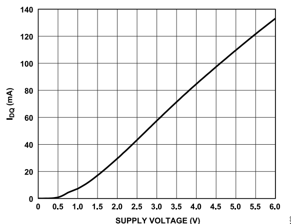
Figure 82. I_{DQ} vs. Supply Voltage, R_{BIAS} = 280\Omega
