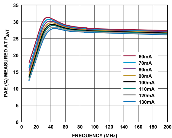
Figure 56. PAE Measured at P_{SAT} vs. Frequency for Various I_{DQ} Values, 10MHz to 200MHz, V_{DD} = 5V
