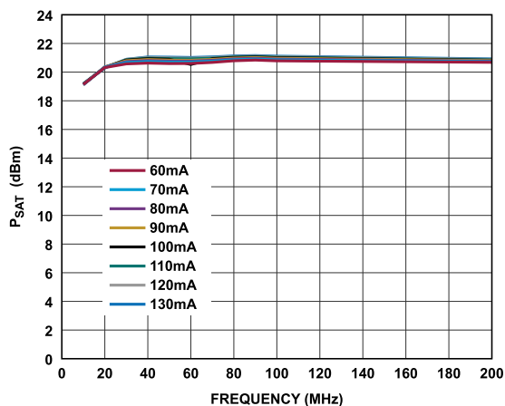
Figure 50. P_{SAT} vs. Frequency for Various I_{DQ} Values, 10MHz to 200MHz, V_{DD} = 5\text{V}
