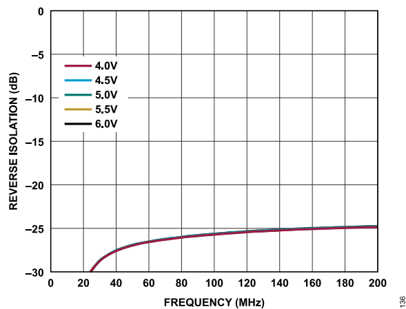
Figure 36. Reverse Isolation vs. Frequency for Various Supply Voltages, 10MHz to 200MHz, I_{DQ} = 110\text{mA}
