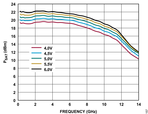
Figure 57. P_{SAT} vs. Frequency for Various Supply Voltages, 200MHz to 14GHz, I_{DQ} = 110mA
