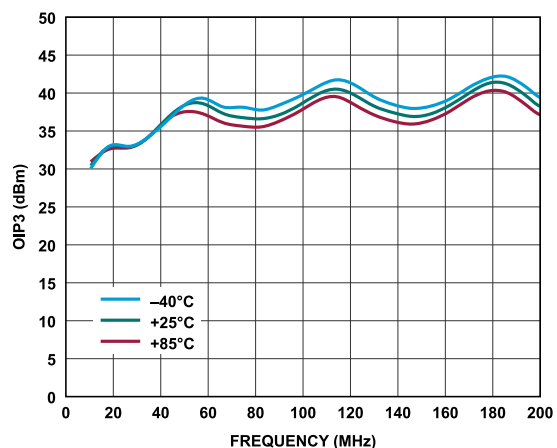
Figure 67. OIP3 vs. Frequency for Various Temperatures, 10MHz to 200MHz, V_{DD} = 5V , I_{DQ} = 110mA
