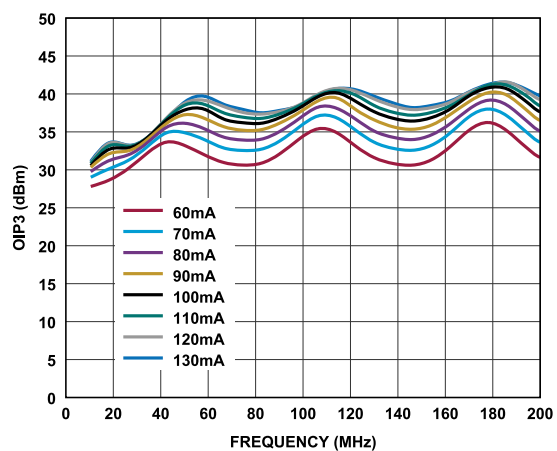
Figure 68. OIP3 vs. Frequency for Various I_{DQ} Values, 10MHz to 200MHz, V_{DD} = 5V
