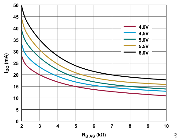
Figure 83. I_{DQ} vs. R_{BIAS} for Various Supply Voltages, 2kΩ to 10kΩ
