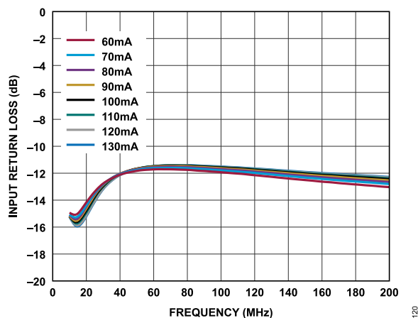
Figure 20. Input Return Loss vs. Frequency for Various I_{DQ} Values, 10MHz to 200MHz, V_{DD} = 5V
