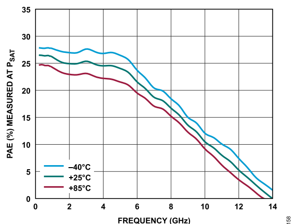
Figure 58. PAE Measured at P_{SAT} vs. Frequency for Various Temperatures, 200MHz to 14GHz, V_{DD} = 5V , I_{DQ} = 110mA
