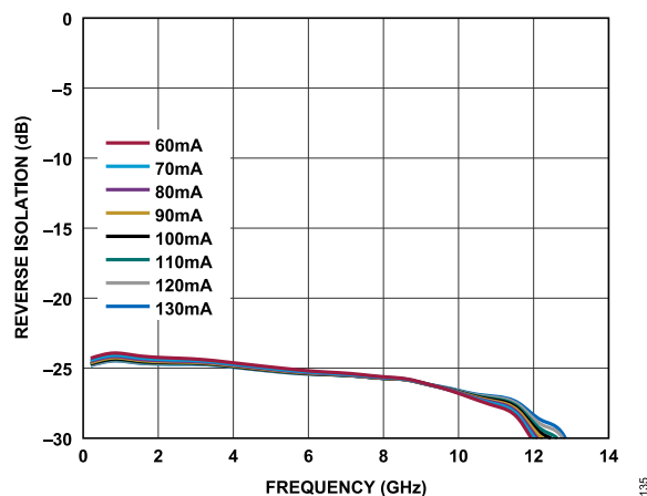
Figure 35. Reverse Isolation vs. Frequency for Various I_{DQ} Values, 200MHz to 14GHz, V_{DD} = 5\text{V}
