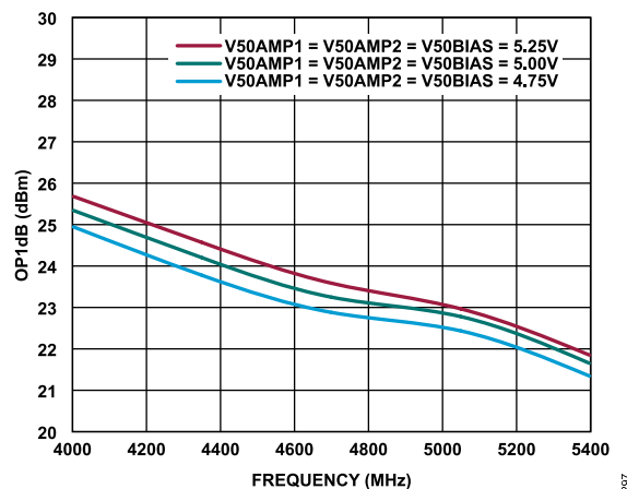
Figure 97. OP1dB vs. Frequency for Various Supplies
