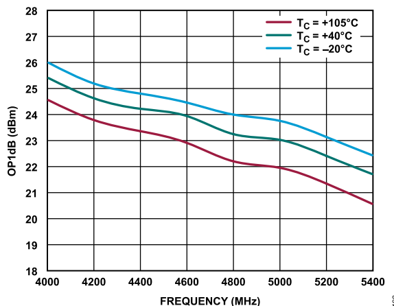
Figure 98. OP1dB vs. Frequency for Various Temperatures
