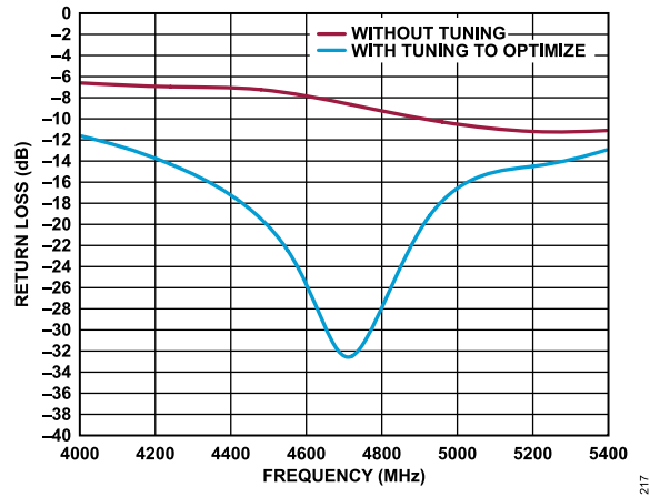
Figure 117. Return Loss of Differential RF Input S11 at 100 \Omega Match; 0.6 pF in Shunt and 0.8 nH Series on Each Input
