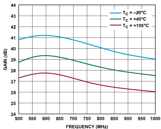
Figure 14. Gain vs. Frequency for Various Temperatures
