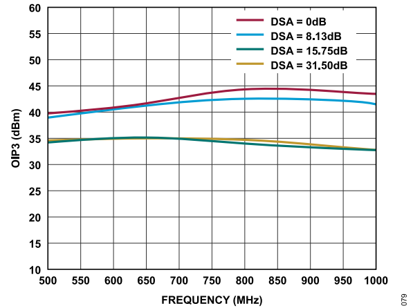
Figure 21. OIP3 vs. Frequency at Various DSA Values
