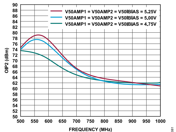
Figure 23. OIP2 vs. Frequency for Various Supplies
