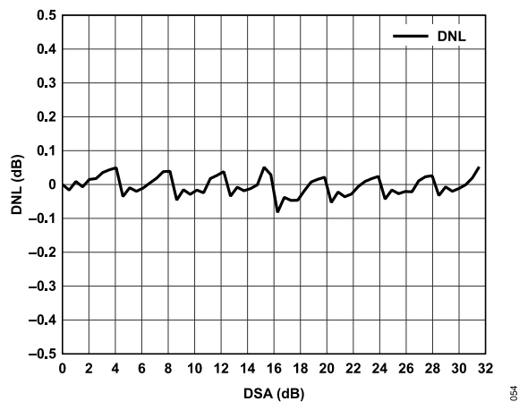
Figure 60. DSA Gain Step Error; Frequency = 2100 MHz
