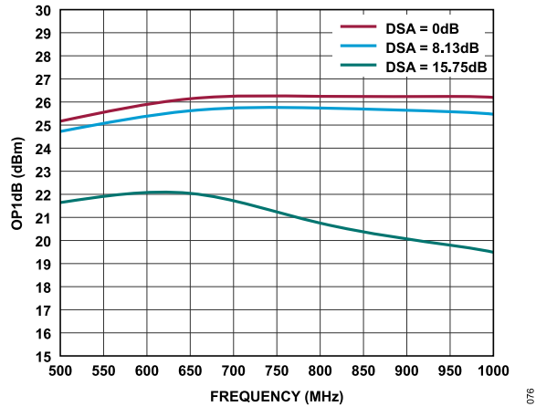
Figure 18. OP1dB vs. Frequency at Various DSA Values
