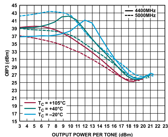
Figure 103. OIP3 vs. Output Power Per Tone for Various Temperatures at 4400 MHz and 5000 MHz
