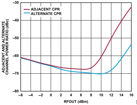
Figure 118. Adjacent and Alternate Channel Power Ratio vs. Output Power (RFOUT) by P_{IN} at 4700 MHz, LTE Test Model 1.1 (TM1.1) 5 MHz, DSA = 0 dB
