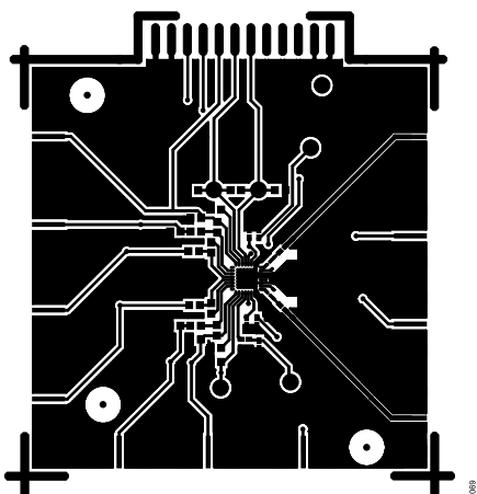
Figure 73. Top Side Layout
