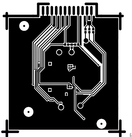
Figure 75. Bottom Side Layout
