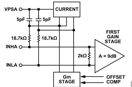
Figure 52. Single-Channel Input Interface
