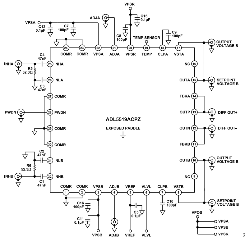
Figure 53. Basic Connections for Operation in Measurement Mode
