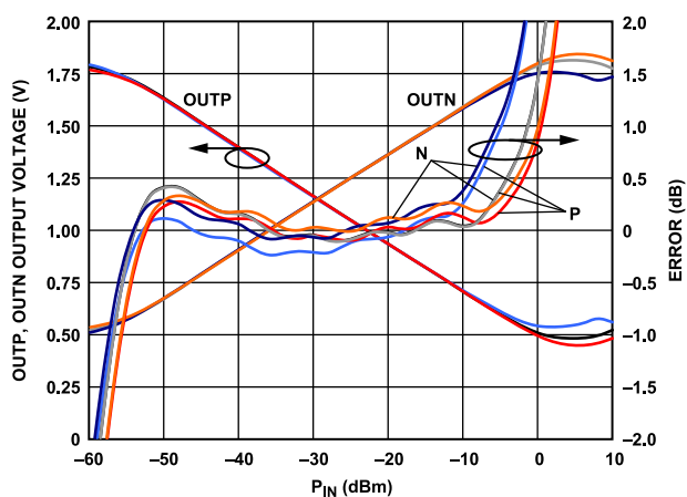
Figure 31. OUTP, OUTN Gain Error and Voltage vs. Input Amplitude at 5.8 GHz, Typical Device, ADJA, ADJB = 0.58 V, 0.7 V, Sine Wave, Single-Ended Drive, P_{INB} = -30 dBm, Channel A Swept
