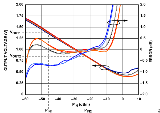
Figure 61. Dynamic Range Extension by Choosing Calibration Points That Are Close to the End of the Linear Range, 2.14 GHz
