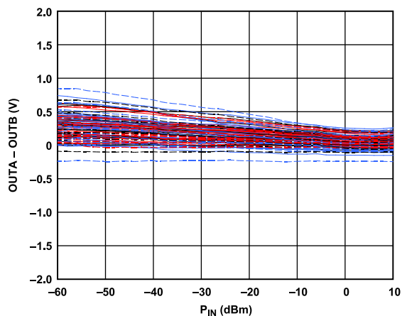
Figure 5. Distribution of [OUTA - OUTB] Voltage Difference over Temperature for 45 Devices from a Nominal Lot, Frequency = 100 MHz, ADJA, ADJB = 0.65 V, 0.7 V, Sine Wave, Single-Ended Drive
