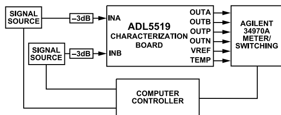
Figure 59. General Characterization Configuration
