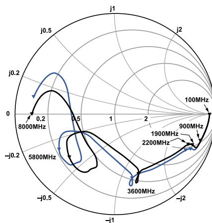
Figure 38. Single-Ended Input Impedance (S11) vs. Frequency; Z_0 = 50 \Omega
