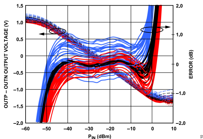
Figure 37. Distribution of [OUTP - OUTN] Gain Error and Voltage vs. Input Amplitude over Temperature, After Ambient Normalization for 45 Devices from a Nominal Lot, Frequency = 8 GHz, ADJA, ADJB = 0.72 V, 0.82 V, Sine Wave, Single-Ended Drive, P_{INH} = -30 dBm, Channel A Swept
