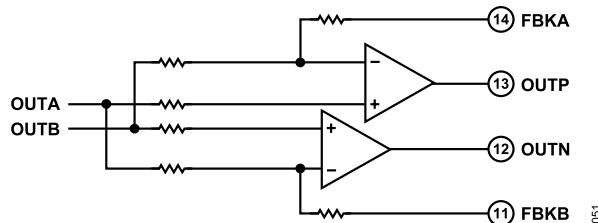
Figure 58. Op Amp Connections (All Resistors Are 1 kΩ ± 20%)
