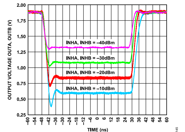
Figure 45. Output Response to RF Burst Input for Various RF Input Levels, Carrier Frequency = 900 MHz, CLPA = Open
