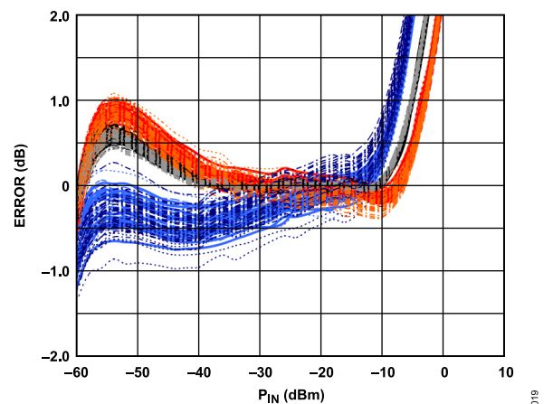
Figure 19. Distribution of OUTA, OUTB Error over Temperature After Ambient Normalization vs. Input Amplitude for at Least 45 Devices from a Nominal Lot
