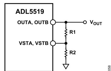
Figure 64. External Network to Raise Slope
