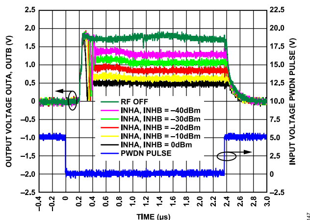
Figure 47. Output Response Using Power-Down Mode for Various RF Input Levels, Carrier Frequency = 900 MHz, CLPA = Open
