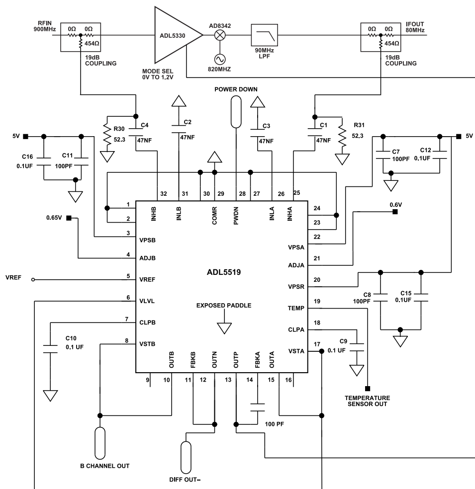
Figure 69. Gain-Stable Receiver Circuit
