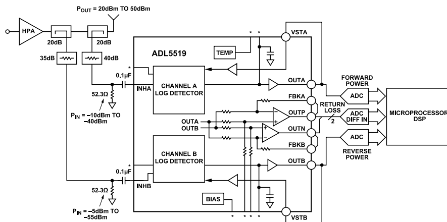
Figure 70. ADL5519 VSWR Level Planning
