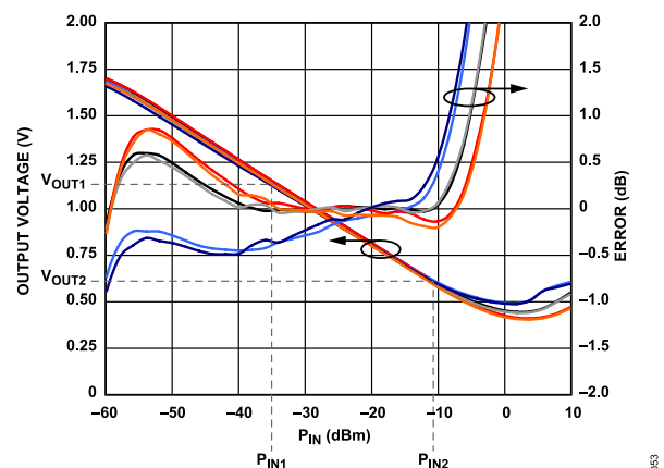
Figure 60. Transfer Function at 2.2 GHz with Calibration Points
