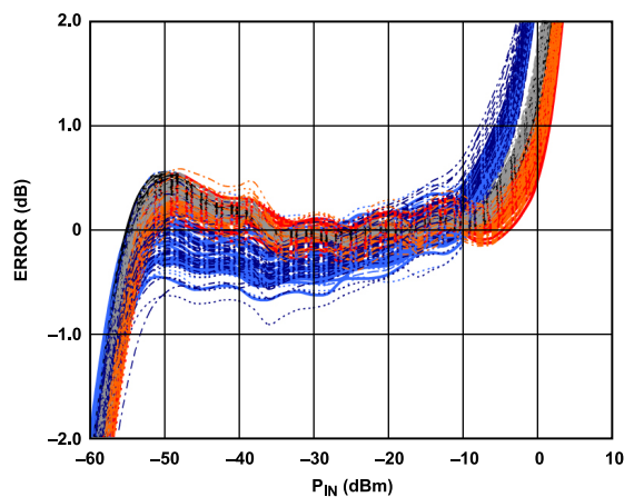
Figure 29. Distribution of OUTA, OUTB Error over Temperature After Ambient Normalization vs. Input Amplitude for at Least 15 Devices from Multiple Lots,
