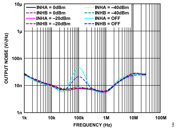
Figure 44. Noise Spectral Density of OUTA, OUTB; CLPA, CLPB = 0.1 μF, Frequency = 2140 MHz
