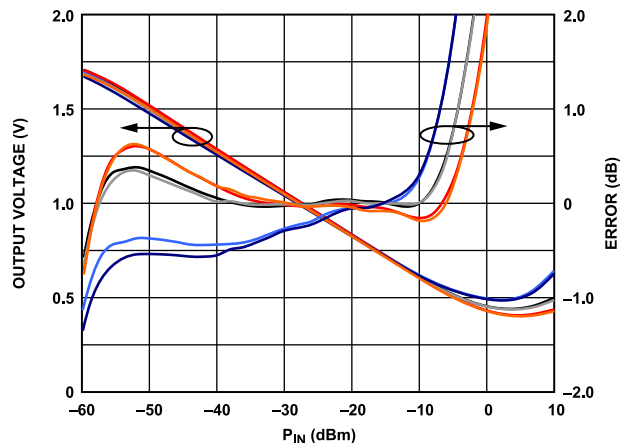
Figure 13. OUTA, OUTB Voltage and Log Conformance vs. Input Amplitude at 1.9 GHz, Typical Device, ADJA, ADJB = 0.5 V, 0.55 V, Sine Wave, Single-Ended Drive
