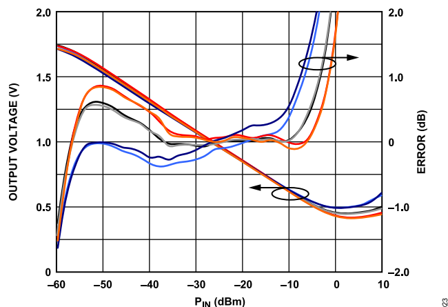
Figure 23. OUTA, OUTB Voltage and Log Conformance vs. Input Amplitude at 3.6 GHz, Typical Device, ADJA, ADJB = 0.35 V, 0.42 V, Sine Wave, Single-Ended Drive
