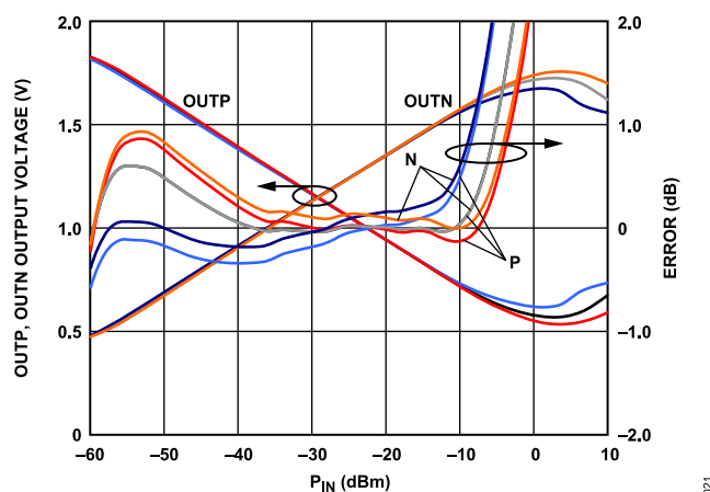
Figure 21. OUTP, OUTN Gain Error and Voltage vs. Input Amplitude at 2.2 GHz, Typical Device, ADJA, ADJB = 0.48 V, 0.6 V, Sine Wave, Single-Ended Drive, P_{INHB} = -30 dBm, Channel A Swept
