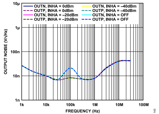
Figure 43. Noise Spectral Density of OUTP, OUTN; CLPA, CLPB = 0.1 μF, Frequency = 2140 MHz
