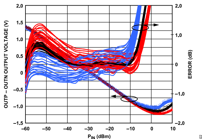
Figure 22. Distribution of [OUTP - OUTN] Gain Error and Voltage vs. Input Amplitude over Temperature, After Ambient Normalization for 45 Devices from a Nominal Lot, Frequency = 2.2 GHz, ADJA, ADJB = 0.48 V, 0.6 V, Sine Wave, Single-Ended Drive, P_{INHB} = -30 dBm, Channel A Swept
