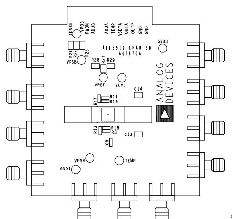
Figure 76. Bottom Side Silkscreen
