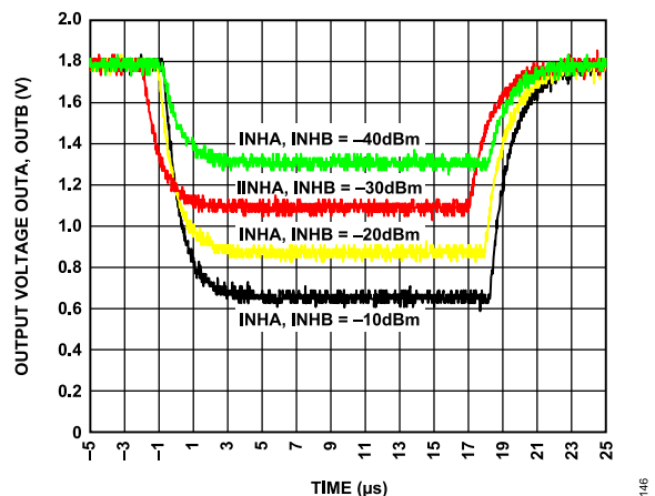
Figure 46. Output Response to RF Burst Input for Various RF Input Levels, Carrier Frequency = 900 MHz, CLPA = 0.1 \mu F
