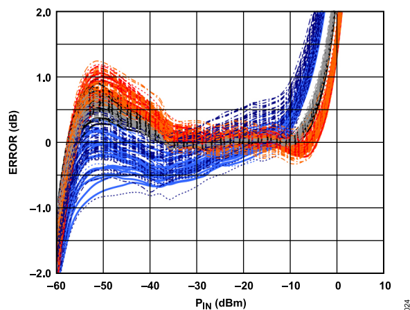
Figure 24. Distribution of OUTA, OUTB Error over Temperature After Ambient Normalization vs. Input Amplitude for 45 Devices from a Nominal Lot, Frequency = 2.2 GHz, ADJA, ADJB = 0.48 V, 0.6 V, Sine Wave, Single-Ended Drive
