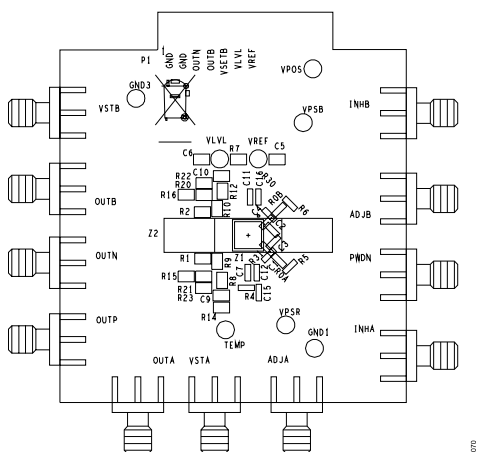
Figure 74. Top Side Silkscreen
