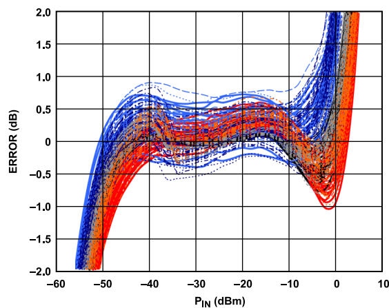
Figure 34. Distribution of OUTA, OUTB Error over Temperature After Ambient Normalization vs. Input Amplitude for 45 Devices from a Nominal Lot, Frequency = 5.8 GHz, ADJA, ADJB = 0.58 V, 0.7 V, Sine Wave, Single-Ended Drive, P_{INB} = -30 dBm, Channel A Swept
