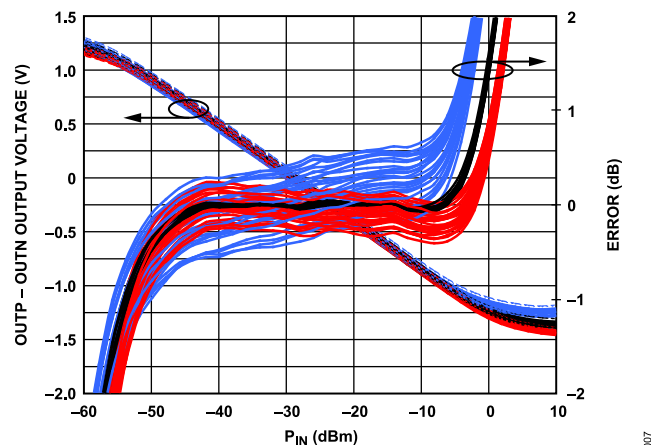
Figure 7. Distribution of [OUTP - OUTN] Gain Error and Voltage vs. Input Amplitude over Temperature, After Ambient Normalization for 45 Devices from a Nominal Lot, Frequency = 100 MHz, ADJA, ADJB = 0.65 V, 0.7 V, Sine Wave, Single-Ended Drive, P_{INH} = -30\text{ dBm} , Channel A Swept
