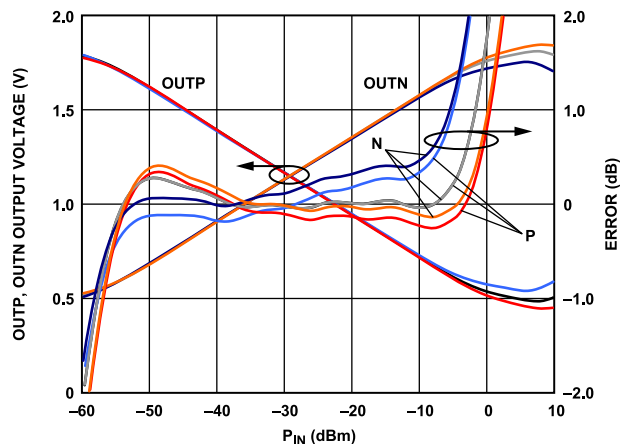
Figure 11. OUTP, OUTN Gain Error and Voltage vs. Input Amplitude at 900 MHz, Typical Device, ADJA, ADJB = 0.6 V, 0.65 V, Sine Wave, Single-Ended Drive; P_{INH} = -30 dBm, Channel A Swept
