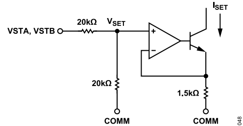
Figure 55. VSTA, VSTB Interface Simplified Schematic
