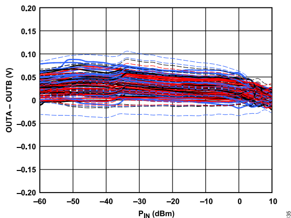
Figure 35. Distribution of [OUTA - OUTB] Voltage Difference over Temperature for 45 Devices from a Nominal Lot, Frequency = 8 GHz, ADJA, ADJB = 0.72 V, 0.82 V, Sine Wave, Single-Ended Drive
