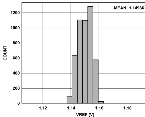
Figure 39. Distribution of VREF Pin Voltage for 4000 Devices
