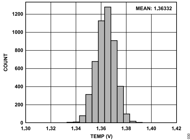
Figure 40. Distribution of TEMP Pin Voltage for 4000 Devices
