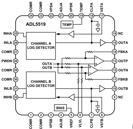
Figure 50. Block Diagram
