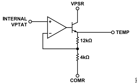
Figure 54. TEMP Interface Simplified Schematic
