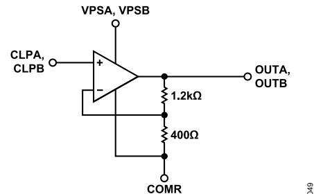
Figure 56. OUTA, OUTB Interface Simplified Schematic
