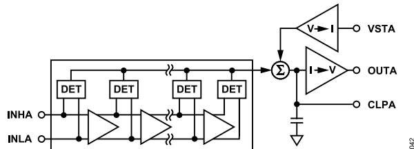
Figure 51. Single Channel Block Diagram
