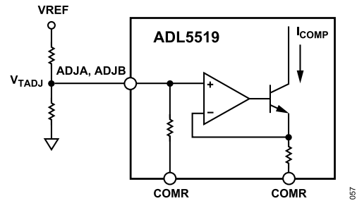
Figure 63. ADJA, ADJB Interface Simplified Schematic
