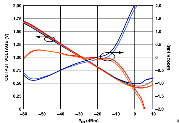
Figure 62. Error vs. Temperature with Respect to Output Voltage at 25°C, 2.14 GHz (Removes Transfer Function Nonlinearities at 25°C)
