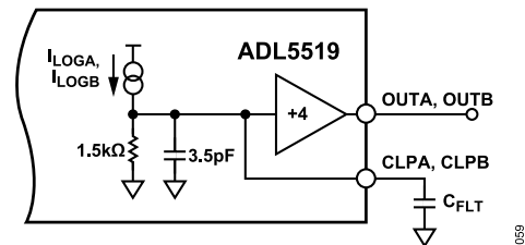
Figure 65. Lowering the Post Demodulation Bandwidth
