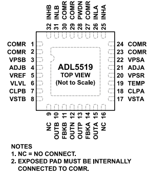
Figure 2. Pin Configuration
