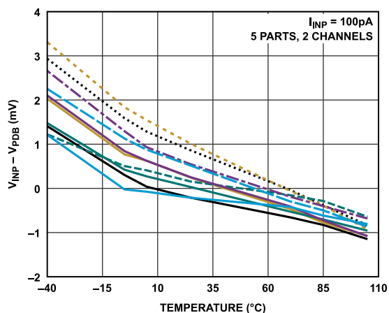
Figure 29. V_{INP} - V_{PDB} vs. Temperature at I_{INP} = 100 pA
