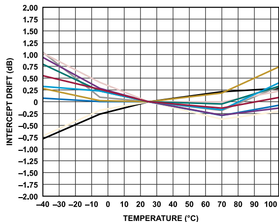
Figure 11. Intercept Drift vs. Temperature Over 10 Samples
