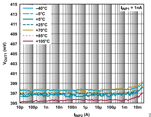
Figure 12. V_{OUT1} vs. I_{INP2} for I_{INP1} = 1 nA
