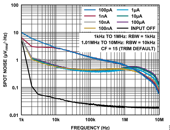
Figure 26. Spot Noise Spectral Density for V_{OUT} vs. I_{INP} at CF = 15
