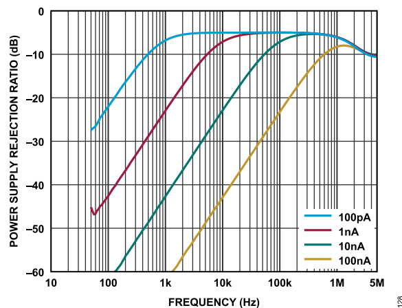
Figure 27. PSRR for Various I_{INP} values
