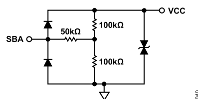
Figure 50. Simplified SBA Interface
