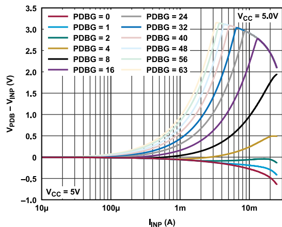
Figure 16. V_{PDB} - V_{INP} vs. I_{INP} for Various PDBG Register Values, with PDBG_Fix = 0 at V_{CC} = 5.0 V
