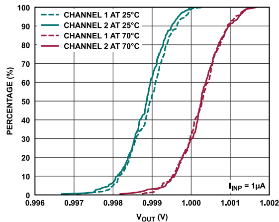
Figure 35. Output Voltage Distribution at I_{INP} = 1 \text{ μA}
