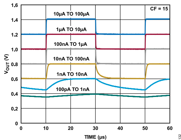
Figure 31. Pulse Response for I_{INP} in Decade Steps for CF = 15
