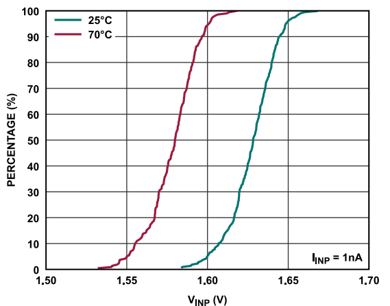
Figure 33. Input Voltage Distribution at I_{INP} = 1 nA
