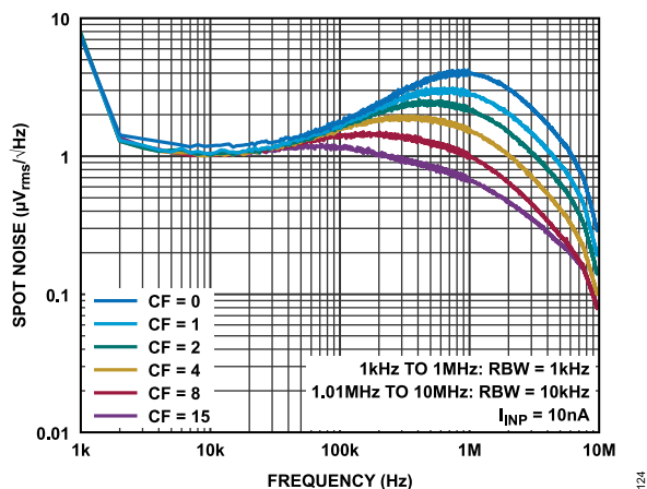
Figure 23. Spot Noise Spectral Density at V_{OUT} for I_{INP} = 10 \text{ nA} at Various CF register values
