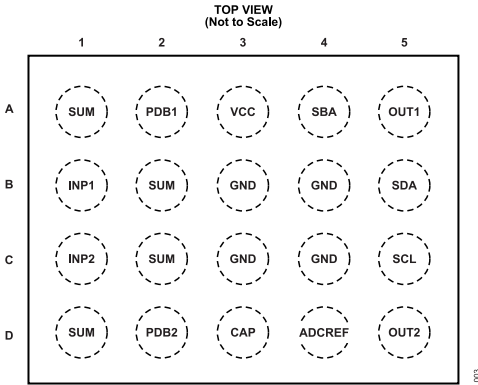
Figure 3. Pin Configuration
