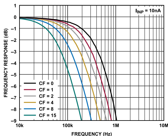
Figure 18. Small Signal AC Response from I_{INP} to V_{OUT} for I_{INP} = 10 nA at Various CF Register Values
