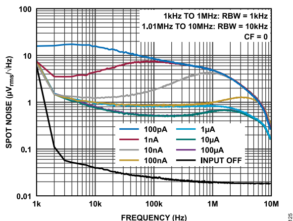
Figure 24. Spot Noise Spectral Density for V_{OUT} vs. I_{INP} at CF = 0
