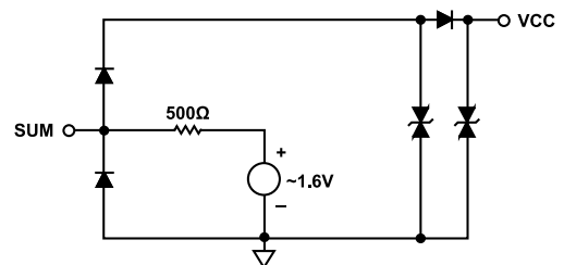
Figure 46. Simplified SUM Interface
