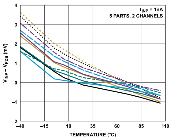
Figure 32. Offset Voltage vs. Temperature at I_{INP} = 1 nA
