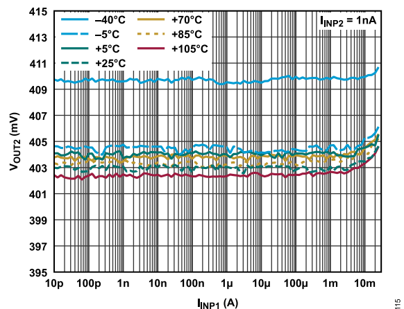
Figure 15. V_{OUT2} vs. I_{INP1} for I_{INP2} = 1 nA
