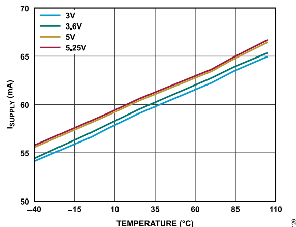
Figure 25. I_{SUPPLY} vs. Temperature for I_{INP1}, I_{INP2} = 10 \text{ nA}
