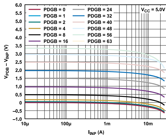
Figure 19. V_{PDB} - V_{INP} vs. I_{INP} for Various PDBG Register Values with PDBG_Fix = 1 at V_{CC} = 5.0 V
