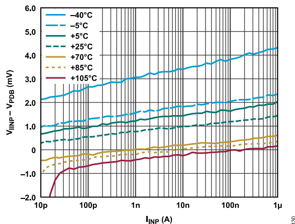
Figure 13. Offset Voltage ( V_{INP} - V_{PDB} ) vs. I_{INP} at Different Temperatures
