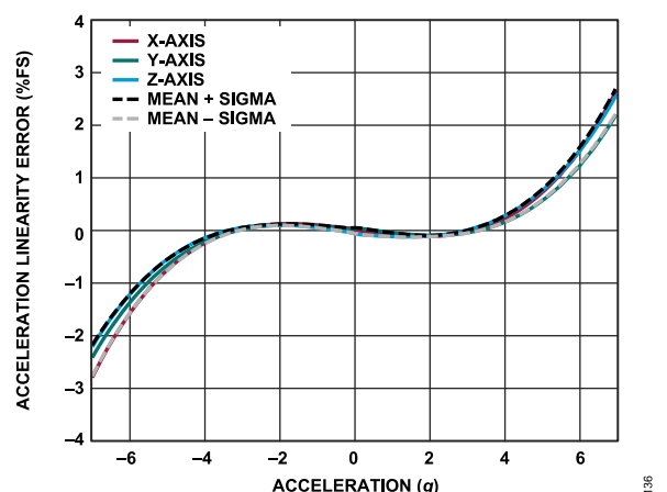
Figure 36. Accelerometer Linearity Error, ADIS16575
