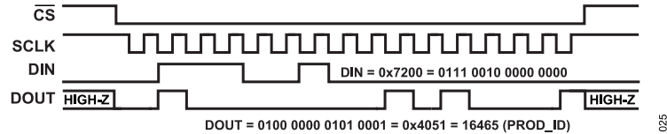
Figure 54. SPI Signal Pattern, Repeating Read of the PROD_ID Register
