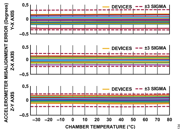
Figure 34. Accelerometer Misalignment Error vs. Chamber Temperature, ADIS16576
