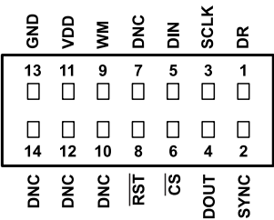
ADIS16575/ADIS16576/ADIS16577 TOP VIEW (Not to Scale)
