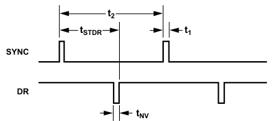
Figure 4. Input Clock Timing Diagram, External Sync Mode, Register MSC_CTRL, Bits[4:2] = 101 (Binary)
