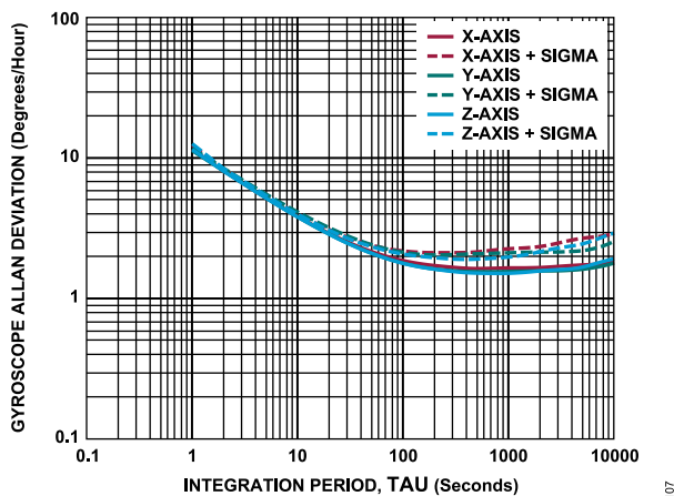
Figure 7. Gyroscope Allan Deviation, T_C = 25^\circ\text{C} , ADIS16575-2, ADIS16576-2, and ADIS16577-2
