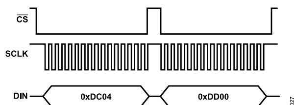
Figure 58. SPI Sequence for Writing 0x0004 to FILT_CTRL
