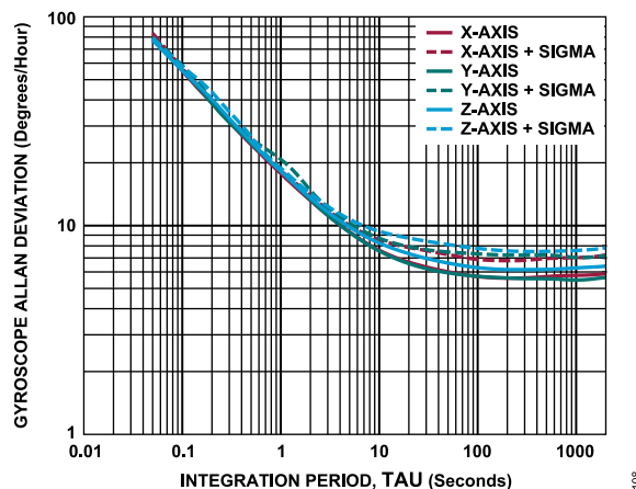
Figure 8. Gyroscope Allan Deviation, T_C = 25^\circ\text{C} , ADIS16576-3 and ADIS16577-3
