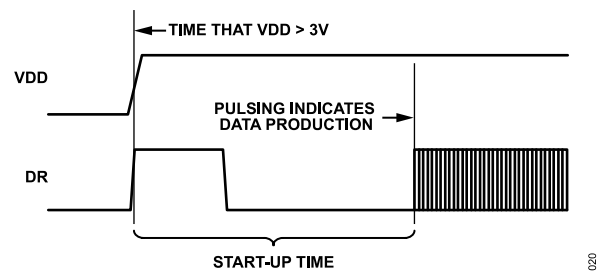
Figure 49. Data Ready Response During Startup
