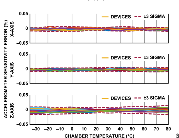
Figure 29. Accelerometer Sensitivity Error vs. Chamber Temperature, ADIS16577
