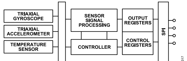
Figure 46. Basic Operation of the ADIS16575/ADIS16576/ADIS16577
