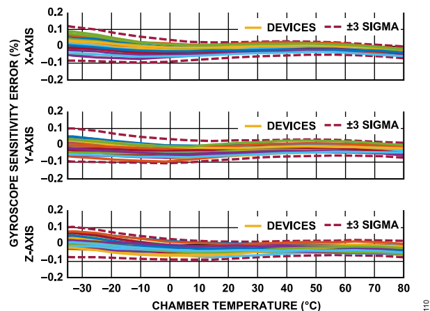
Figure 10. Gyroscope Sensitivity Error vs. Chamber Temperature, ADIS16576-3 and ADIS16577-3
