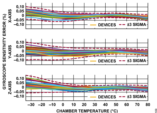
Figure 9. Gyroscope Sensitivity Error vs. Chamber Temperature, ADIS16575-2, ADIS16576-2, and ADIS16577-2
