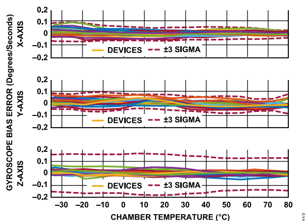
Figure 12. Gyroscope Bias Error vs. Chamber Temperature, ADIS16576-3 and ADIS16577-3
