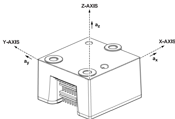
Figure 62. Accelerometer Axis and Polarity Assignments
