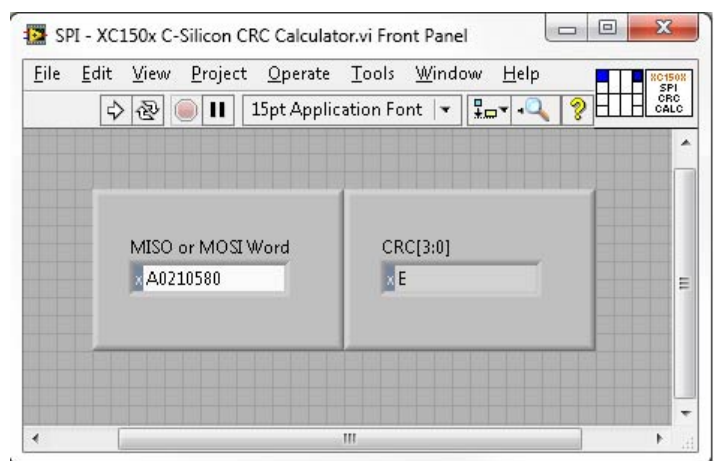
Figure 42. LabVIEW CRC Calculation Example (Front Panel)
