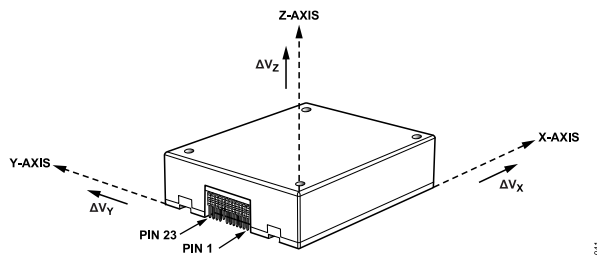
Figure 47. Delta Velocity Axis and Polarity Assignments
