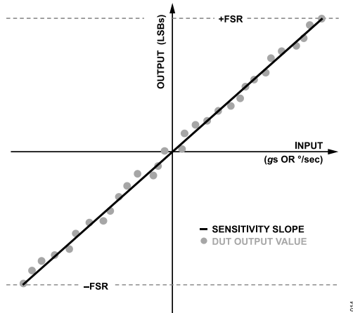
Figure 20. Nominal Sensitivity Slope
