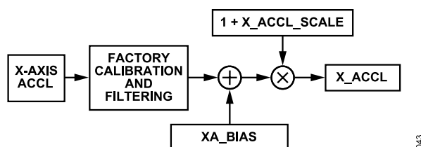
Figure 49. User Bias and Scale Adjustment Registers in Accelerometer Signal Path
