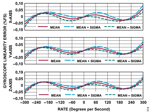
Figure 14. Gyroscope Linearity Error vs. Rate
