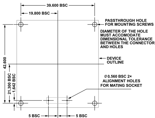
Figure 53. Suggested PCB Layout Pattern, Connector Down
