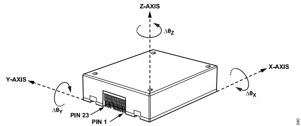
Figure 46. Delta Angle Axis and Polarity Assignments
