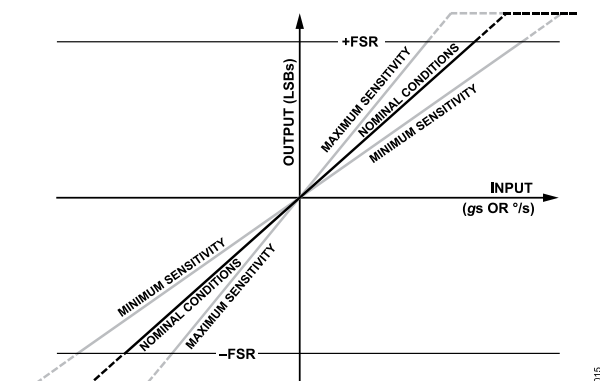
Figure 21. Sensitivity and Scale Factor Transfer Function
