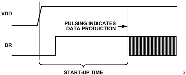
Figure 34. Data Ready Response During Startup
