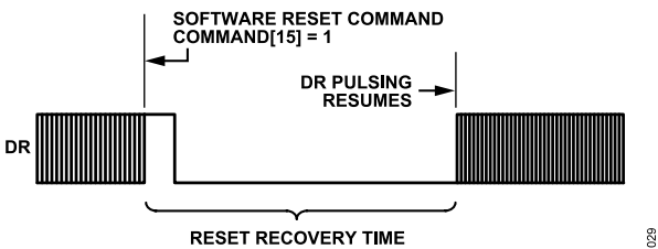
Figure 35. Data Ready Response During Reset (Register COMMAND, Bit 15 = 1) Recovery
