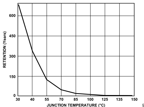
Figure 51. Flash Memory Retention
