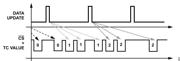
Figure 39. TC—Fast \overline{CS} Rate
