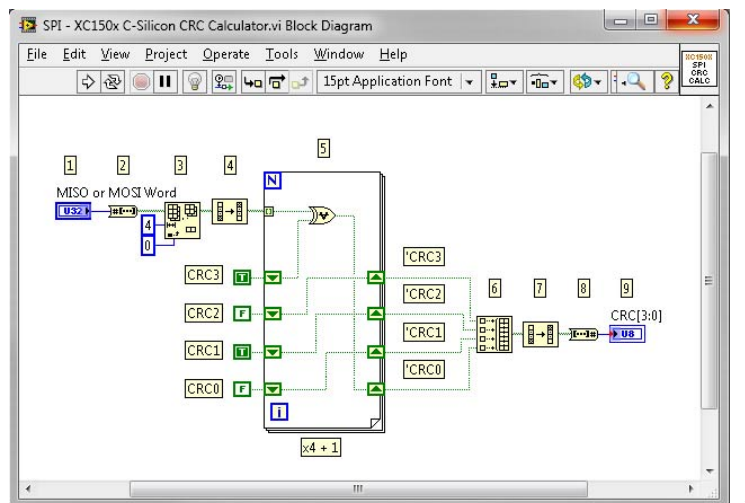
Figure 41. LabVIEW CRC Calculation (Block Diagram)
