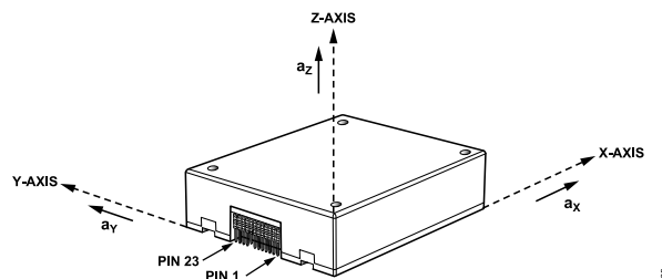
Figure 45. Accelerometer Axis and Polarity Assignments
