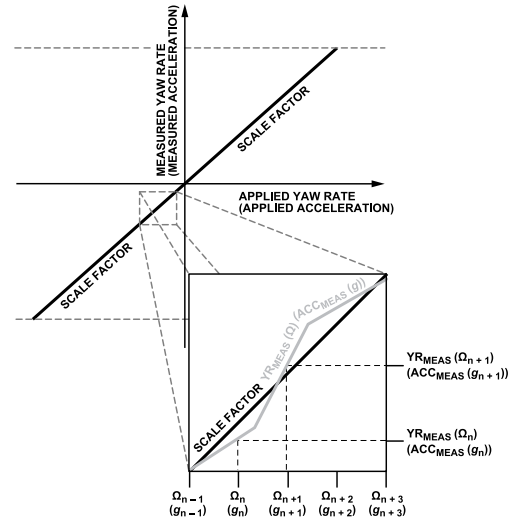
Figure 23. Microlinearity Characteristic
