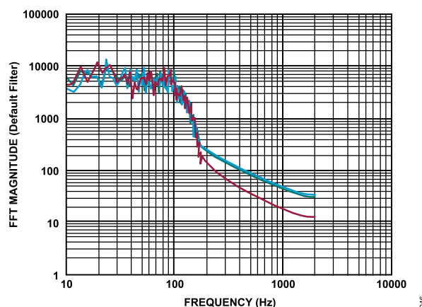
Figure 52. FIR Frequency Response Curve—Default 100 Hz Filter
