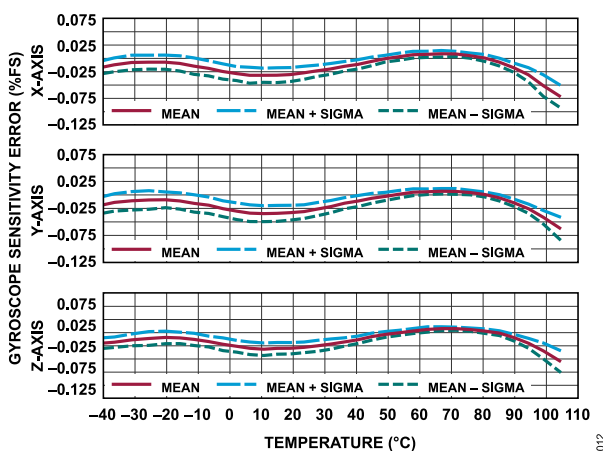
Figure 10. Gyroscope Sensitivity Error vs. Temperature
