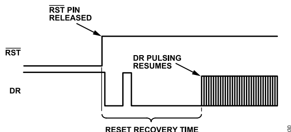
Figure 36. Data Ready Response During Reset ( \overline{RST} = 0 ) Recovery
