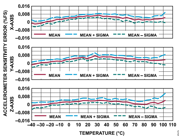
Figure 13. Accelerometer Sensitivity Error vs. Temperature
