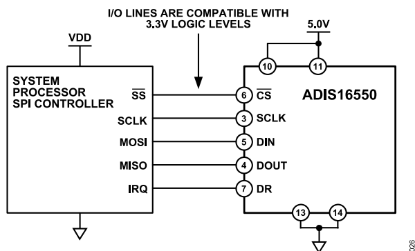
Figure 32. Electrical Connection Diagram
