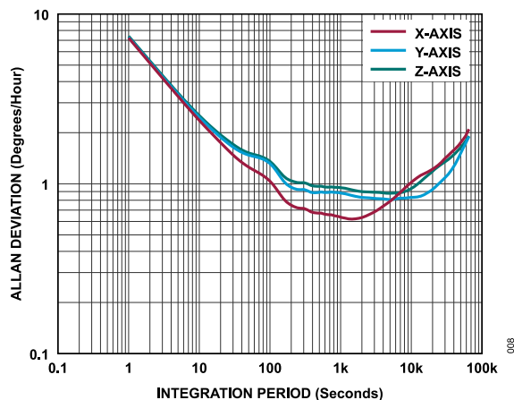
Figure 8. Gyroscope Allan Deviation
