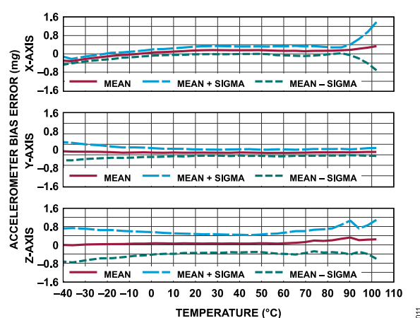
Figure 12. Accelerometer Bias Error vs. Temperature
