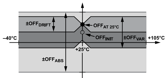
Figure 18. Bias Error over Temperature, OFF_{INIT} \neq OFF_{AT\_25^\circ C} (Change OFF_{AT\_25^\circ C} to OFF_{AT\_25^\circ C} )
