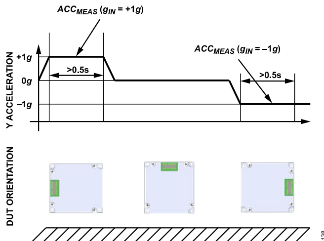
Figure 16. Acceleration Sensitivity Measurement Process
