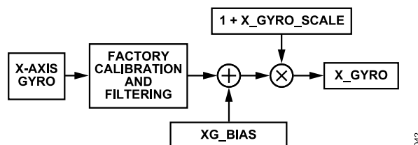
Figure 48. User Bias and Scale Adjustment Registers in Gyroscope Signal Path
