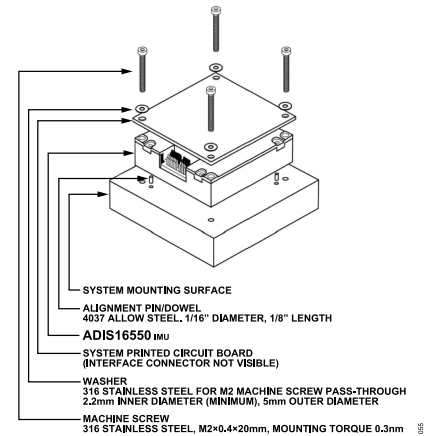
Figure 55. Mechanical Integration Design Example
