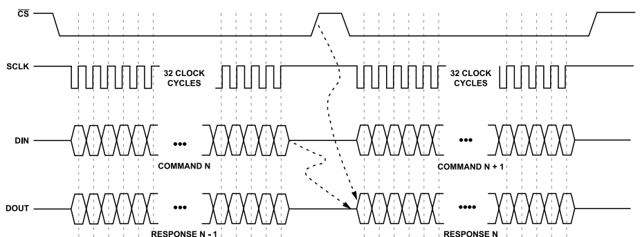
Figure 38. SPI Command and Response Format
