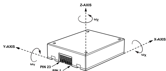
Figure 44. Gyroscope Axis and Polarity Assignments
