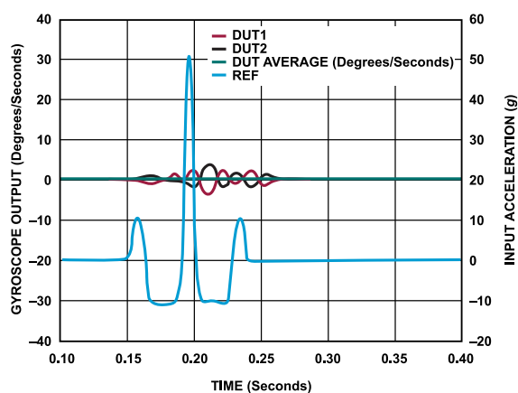
Figure 24. Sensitivity to Linear Acceleration
