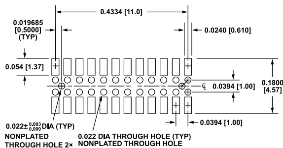
Figure 54. Suggested Layout and Mechanical Design when Using Samtec CLM-112-02-G-D-A for the Mating Connector
