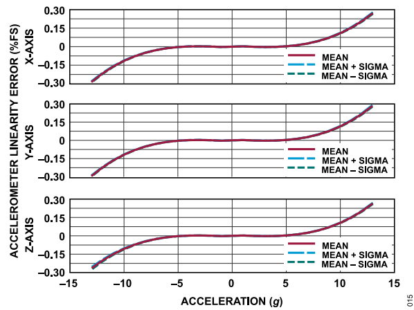
Figure 15. Accelerometer Linearity Error vs. Acceleration
