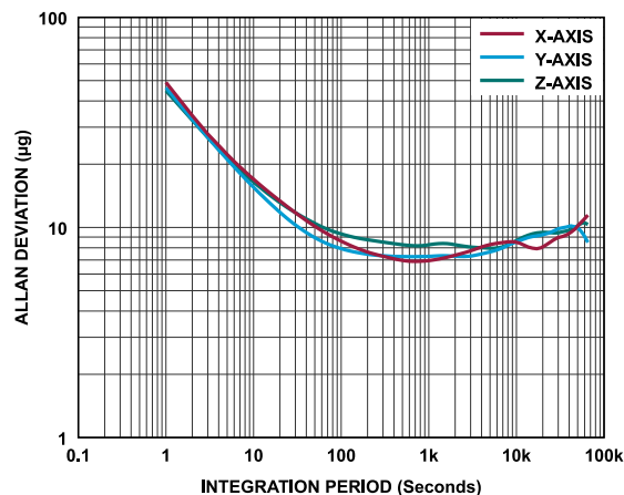
Figure 11. Accelerometer Allan Deviation
