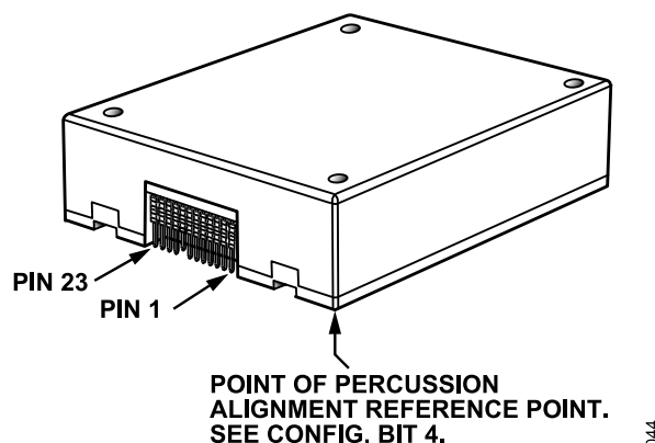
Figure 50. Point of Percussion Reference Point
