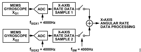
Figure 26. Gyroscope Data Sampling
