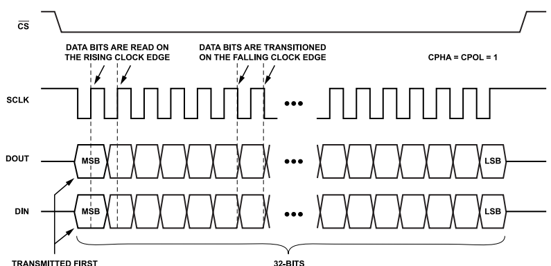
Figure 37. SPI Communication Structure
