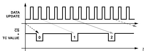
Figure 40. TC—Slow \overline{CS} Rate
