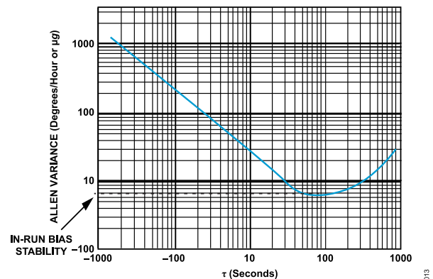
Figure 19. Example Allan Variance Plot
