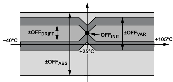
Figure 17. Bias Error over Temperature, OFF_{INIT} = OFF_{AT\_25^\circ C}
