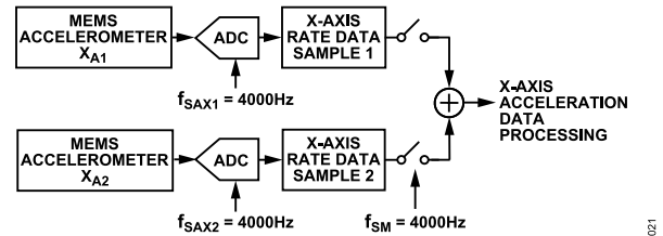
Figure 27. Accelerometer Data Sampling
