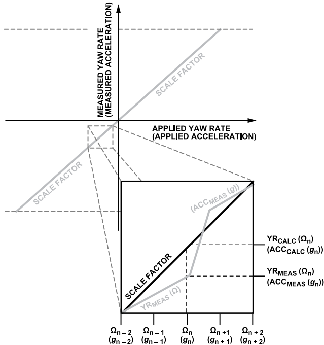
Figure 22. Nonlinearity Characteristic
