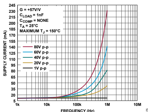
Figure 75. Supply Current and Amplitude vs. Frequency Square Wave, with Heatsink and Airflow, C_{LOAD} = 1nF , C_{COMP} = None
