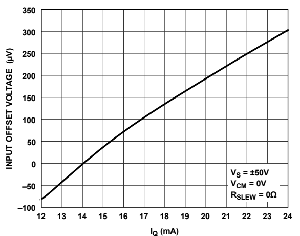
Figure 60. Input Offset Voltage vs. I_Q
