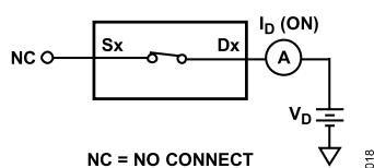
Figure 16. On Leakage
