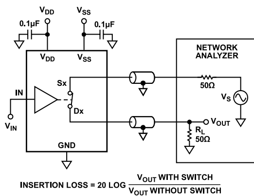
Figure 21. Bandwidth
