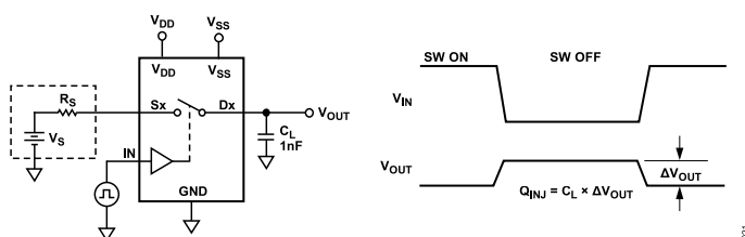
Figure 18. Charge Injection
