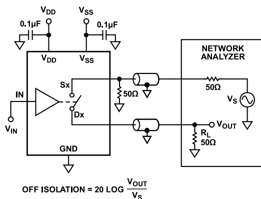
Figure 19. Off Isolation
