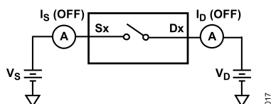
Figure 15. Off Leakage
