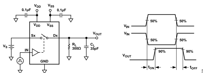
Figure 17. Switching Times ( t_{ON} , t_{OFF} )
