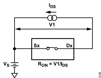
Figure 14. On Resistance
