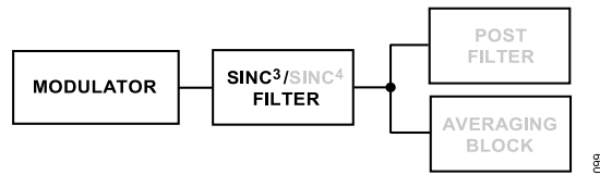
Figure 89. Sinc³ Filter
