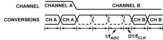
Figure 90. Sinc³ Channel Change
