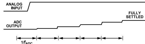
Figure 83. Asynchronous Step Change in the Analog Input
