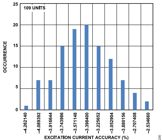
Figure 30. IOUTx Current Initial Accuracy Histogram (500 µA)
