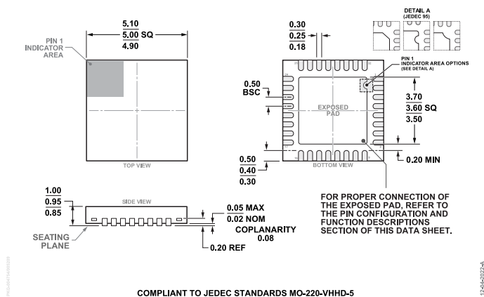
Figure 129. 32-Lead Lead Frame Chip Scale Package [LFCSP] 5 mm × 5 mm Body and 0.95 mm Package Height (CP-32-30) Dimensions shown in millimeters
