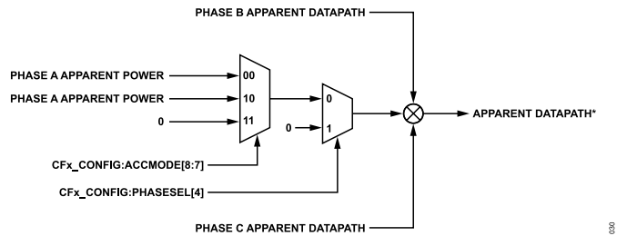
Figure 57. Apparent Datapath
