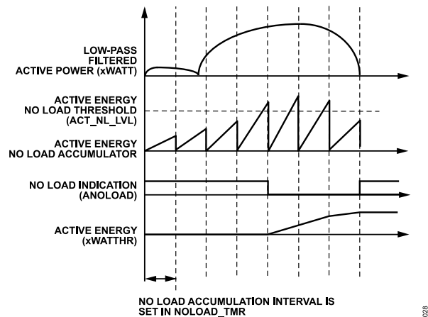
Figure 55. No Load Behavior
