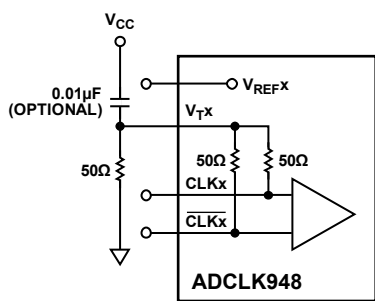
Figure 20. DC-Coupled LVPECL Input Termination
