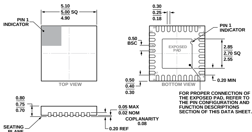
Figure 24. 32-Lead Lead Frame Chip Scale Package [LFCSP] 5 mm × 5 mm Body and 0.75 mm Package Height (CP-32-21)
