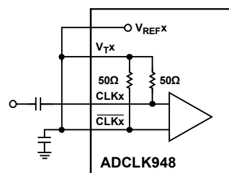
Figure 21. AC-Coupled Input Termination, Such as LVDS and LVPECL
