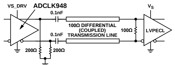
Figure 17. AC-Coupled, LVPECL with Parallel Transmission Line
