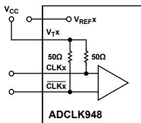
Figure 19. DC-Coupled CML Input Termination
