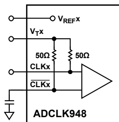
Figure 23. DC-Coupled 3.3 V CMOS Input Termination
