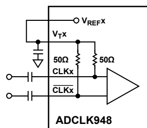
Figure 21. AC-Coupled Input Termination, Such as LVDS and LVPECL
