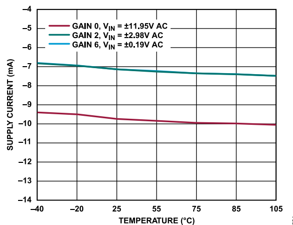
Figure 84. VSS_PGA Supply Current vs. Temperature at Various Gain Modes, AC Input
