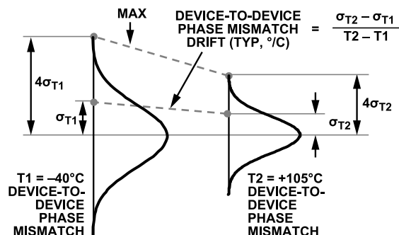
Figure 91. Device-to-Device Phase Mismatch Drift Calculation
