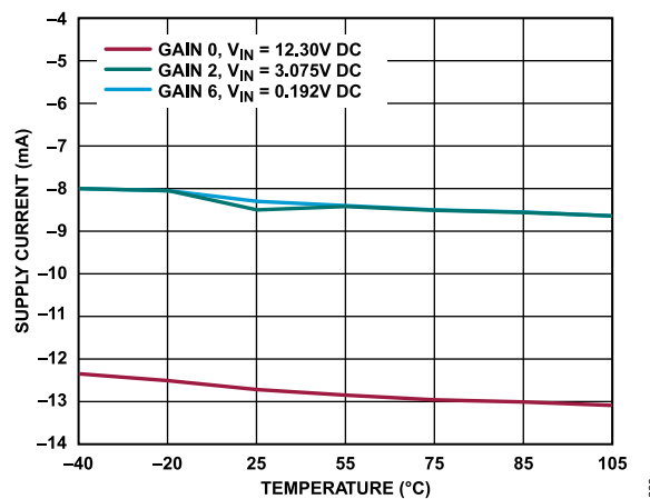
Figure 83. VSS_PGA Supply Current vs. Temperature at Various Gain Modes, DC Input
