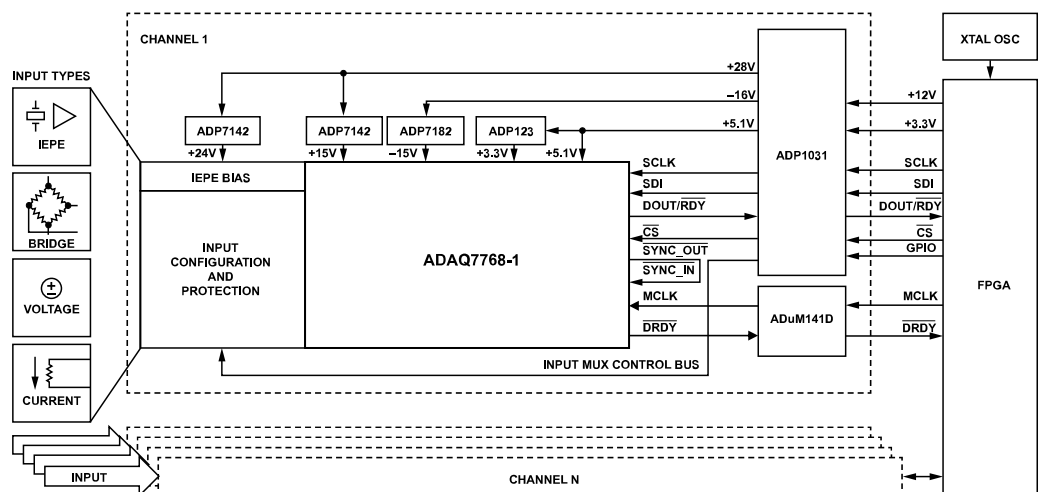
Figure 145. Typical Applications Diagram of a Per Channel Isolated DAQ System
