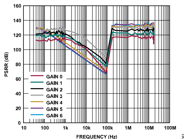
Figure 79. VSS_PGA AC PSRR Across All Gain Modes, Using the Internal Supply Decoupling Capacitor Only
