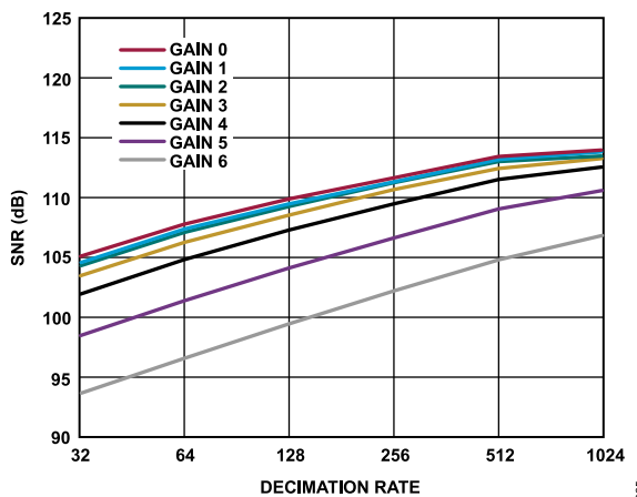
Figure 61. SNR vs. Decimation Rate Across All Gain Modes, Wideband Low Ripple Filter, -0.5 dBFS, 1 kHz
