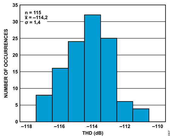
Figure 53. THD Distribution, AFE_GAIN = 20.8 V/V (Gain 6 Mode)
