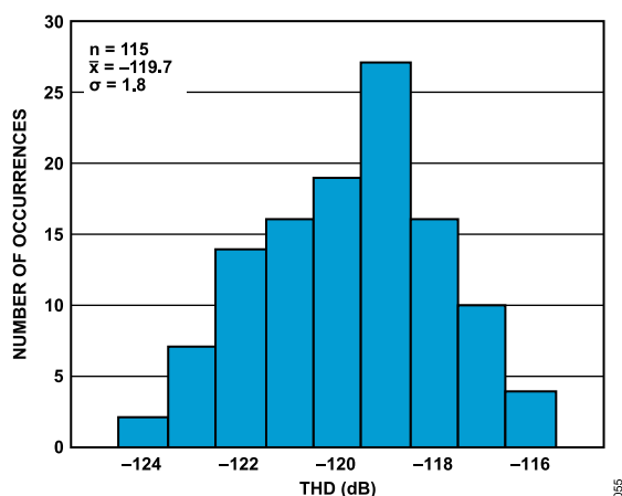
Figure 51. THD Distribution, AFE_GAIN = 0.325 V/V (Gain 0 Mode)
