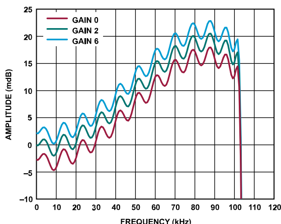
Figure 114. Wideband Low Ripple FIR Filter Passband Ripple, Normalized to Gain 2 Mode
