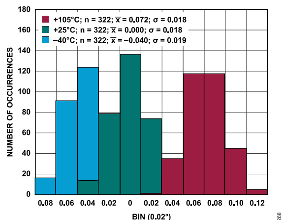
Figure 68. Device-to-Device Phase Angle Mismatch, 20 kHz, AFE_GAIN = 0.325 V/V (Gain 0 Mode), Normalized to the Mean Value at 25°C
