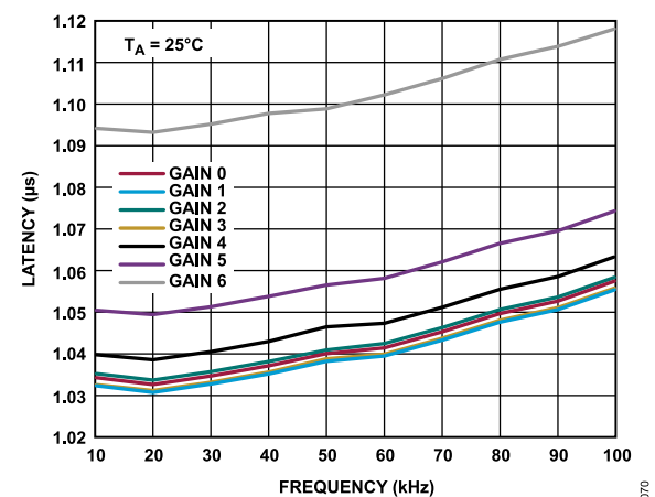
Figure 66. Analog Front-End (AFE) Latency vs. Passband Frequency Across All Gain Modes at 25°C
