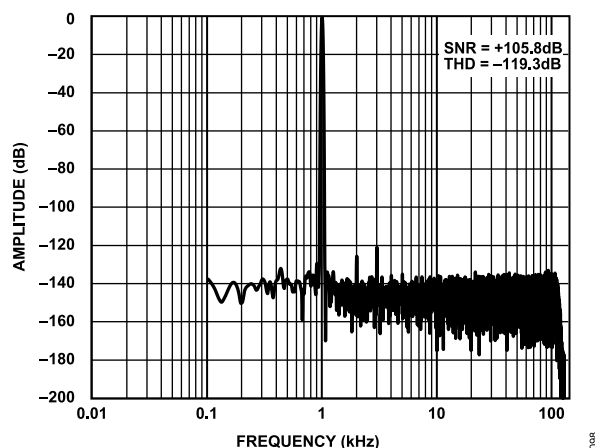
Figure 95. Fully Differential Input, -0.5 dBFS, 1 kHz Sine, V_{CM} = 0 V, ODR = 256 kSPS, V_{REF} = 4.096 V, AFE_GAIN = 0.325 V/V (Gain 0 Mode)
