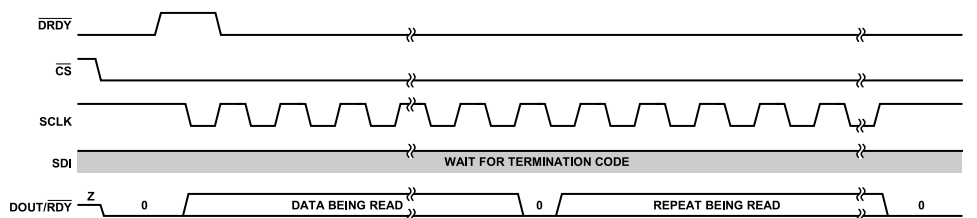
Figure 138. Continuous ADC Read Data Format with \overline{\text{RDY}} Function Disabled
