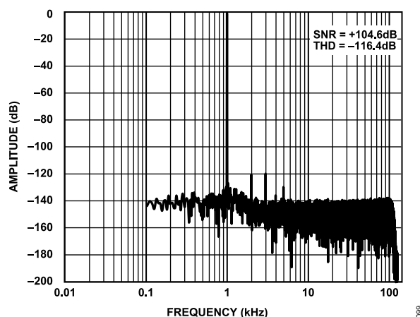
Figure 96. Fully Differential Input, -0.5 dBFS, 1 kHz Sine, V_{CM} = 0 V, ODR = 256 kSPS, V_{REF} = 4.096 V, AFE_GAIN = 1.3 V/V (Gain 2 Mode)
