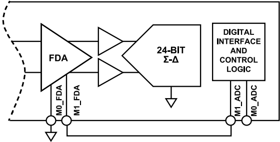
Figure 103. FDA Low-Power Mode Connection
