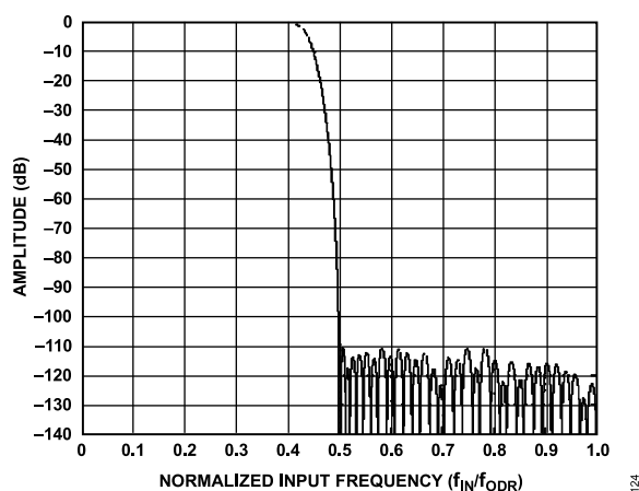
Figure 113. Low Ripple FIR Filter Frequency Response
