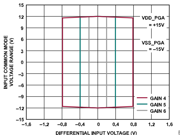
Figure 99. Input Range Diamond Plot for Various Gains
