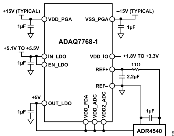
Figure 107. ADAQ7768-1 Power Supply Connection Using Internal LDO
