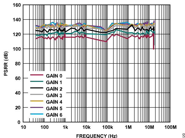
Figure 109. LDO AC PSRR, Using the 0.1 \mu\text{F} Internal Decoupling Capacitors of VDD2_PGA, VDD_FDA, VDD_ADC, VDD2_ADC, and Recommended 1 \mu\text{F} External Decoupling Capacitor at OUT_LDO
