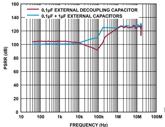
Figure 112. VDD_IO AC PSRR Using External 0.1 \mu\text{F} and Additional 1 \mu\text{F} Supply Decoupling Capacitor
