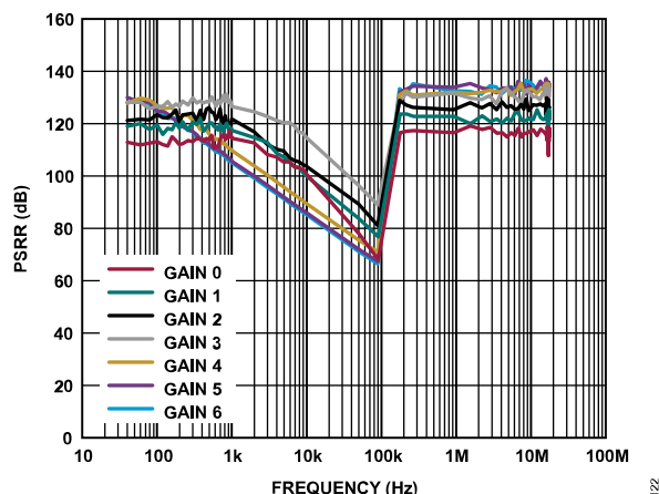
Figure 111. VSS_PGA AC PSRR vs. All Gains, Using the Internal 0.1 \mu\text{F} Supply Decoupling Capacitor Only
