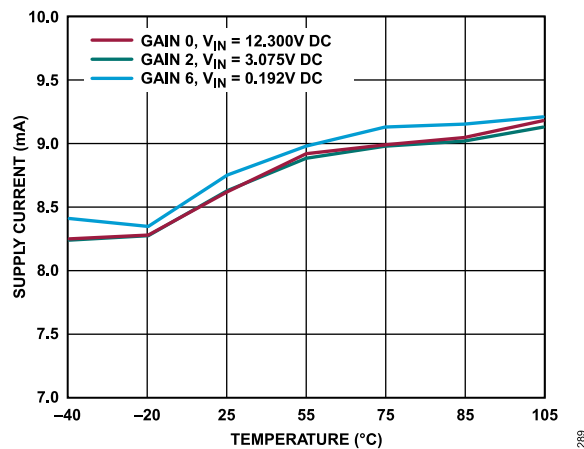
Figure 89. VDD_IO Supply Current vs. Temperature at Various Gain Modes, DC Input
