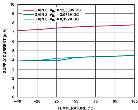
Figure 81. VDD_PGA Supply Current vs. Temperature at Various Gain Modes, DC Input
