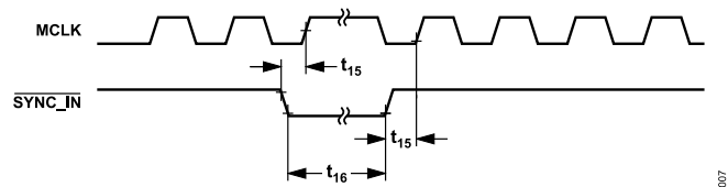
Figure 7. Synchronous \overline{SYNC\_IN} Pulse
