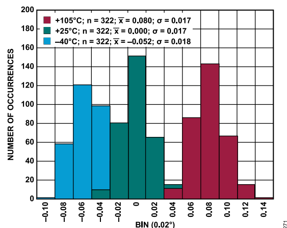
Figure 71. Device-to-Device Phase Angle Mismatch, 20 kHz, AFE_GAIN = 2.6 V/V (Gain 3 Mode), Normalized to the Mean Value at 25°C
