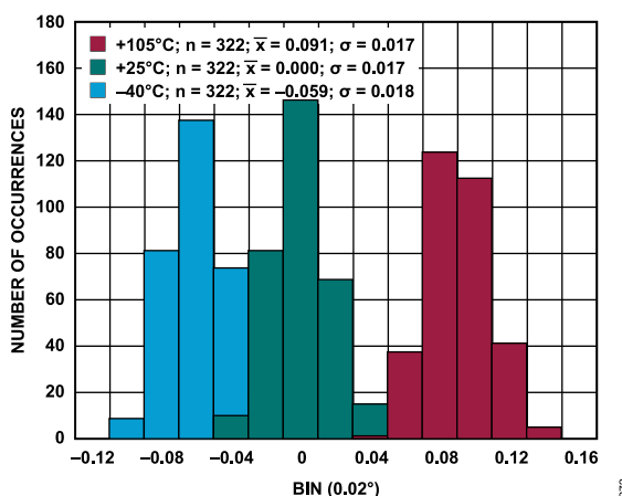
Figure 72. Device-to-Device Phase Angle Mismatch, 20 kHz, AFE_GAIN = 5.2 V/V (Gain 4 Mode), Normalized to the Mean Value at 25°C
