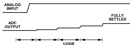
Figure 119. Sinc5 Filter Step Response
