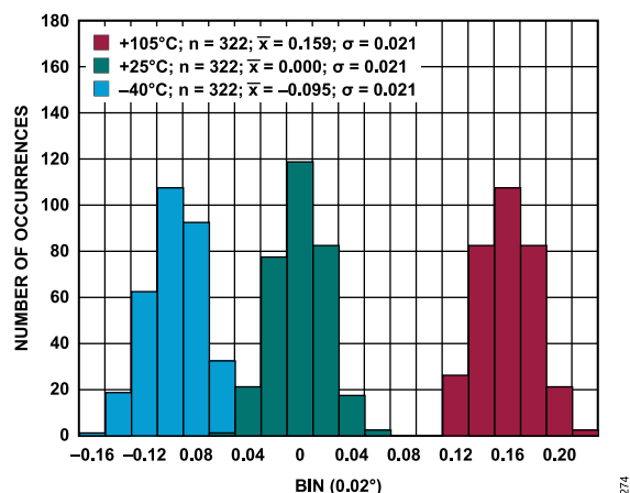
Figure 74. Device-to-Device Phase Angle Mismatch, 20 kHz, AFE_GAIN = 20.8 V/V (Gain 6 Mode), Normalized to the Mean Value at 25°C
