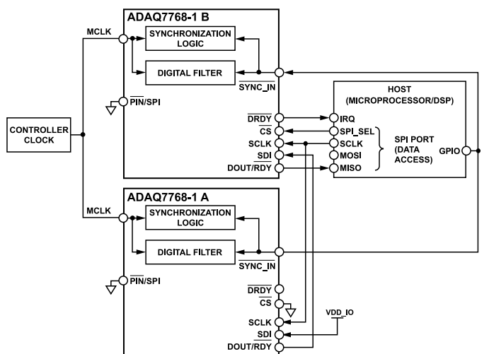
Figure 124. Daisy-Chaining Multiple ADAQ7768-1 Devices
