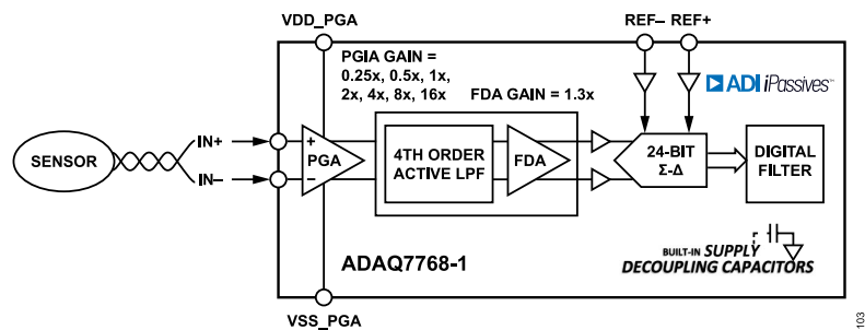
Figure 100. ADAQ7768-1 Top Level Core Signal Chain
