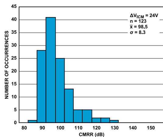
Figure 19. DC CMRR Distribution, V_{ICM} Full Range of \pm 12 V = \Delta V_{ICM} of 24 V, AFE_GAIN = 1.3 V/V (Gain 2 Mode)
