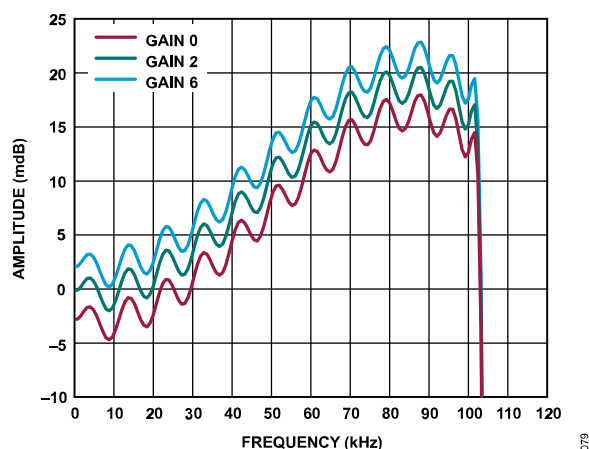
Figure 75. Wideband Low Ripple FIR Filter Pass-Band Ripple, ODR = 256 kSPS, Normalized to AFE_GAIN = 1.3 V/V (Gain 2 Mode)
