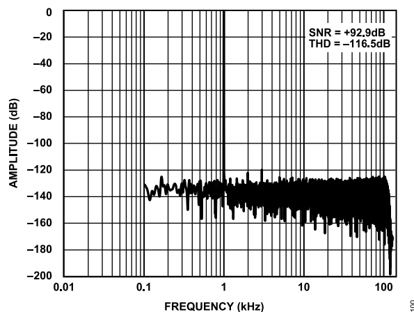
Figure 97. Fully Differential Input, -0.5 dBFS, 1 kHz Sine, V_{CM} = 0 V, ODR = 256 kSPS, V_{REF} = 4.096 V, AFE_GAIN = 20.8 V/V (Gain 6 Mode)
