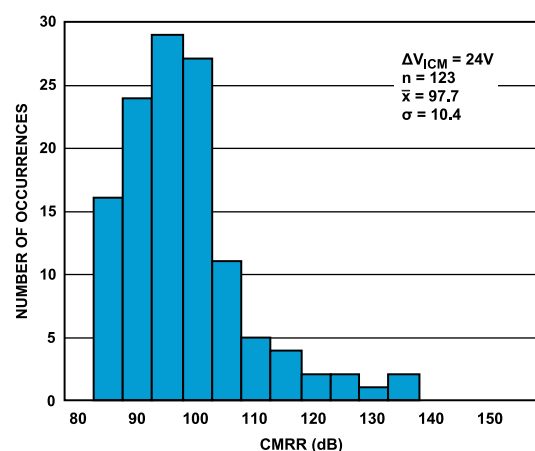
Figure 18. DC CMRR Distribution, V_{ICM} Full Range of \pm 12 V = \Delta V_{ICM} of 24 V, AFE_GAIN = 0.65 V/V (Gain 1 Mode)
