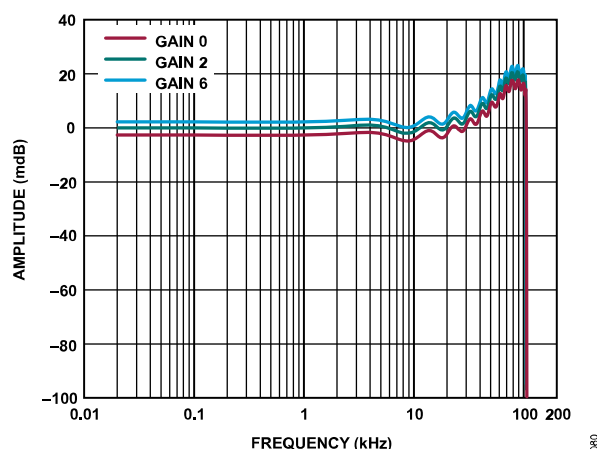
Figure 76. Magnitude Flatness Response, Wideband Low Ripple FIR Filter, ODR = 256 kSPS, Normalized to AFE_GAIN = 1.3 V/V (Gain 2 Mode)
