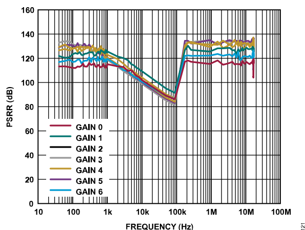
Figure 110. VDD_PGA AC PSRR vs. All Gains, Using the Internal 0.1 \mu\text{F} Supply Decoupling Capacitor Only
