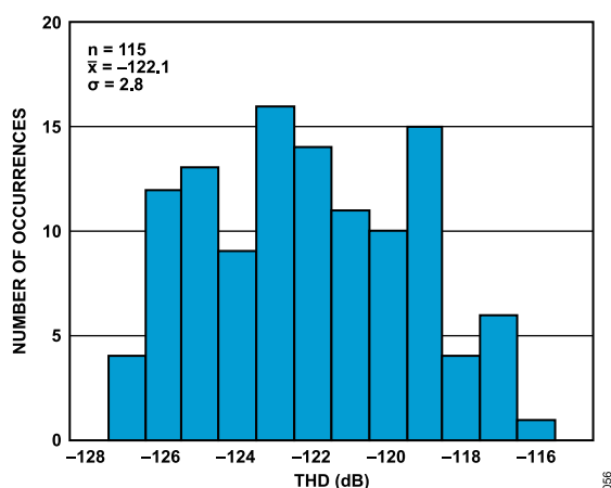
Figure 52. THD Distribution, AFE_GAIN = 1.3 V/V (Gain 2 Mode)
