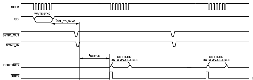
Figure 143. One-Shot Conversion Mode, \overline{SYNC\_IN} Pulse Initiated by a Register Write
