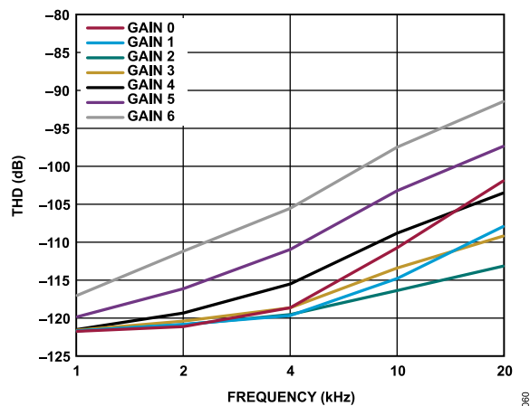
Figure 56. THD vs. Input Frequency Across All Gain Modes, -0.5 dBFS
