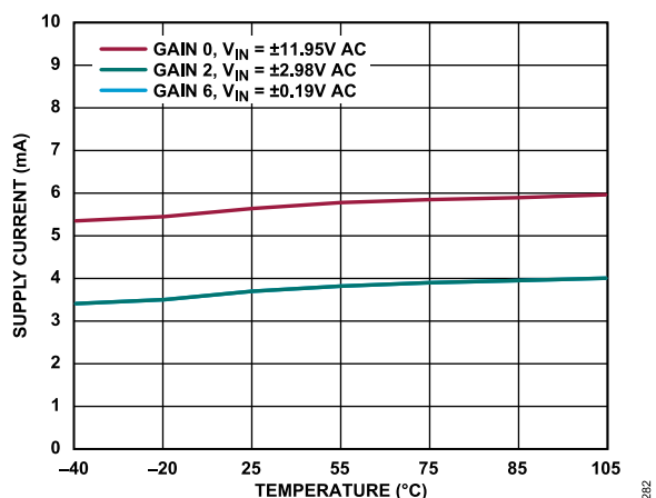
Figure 82. VDD_PGA Supply Current vs. Temperature at Various Gain Modes, AC Input
