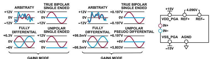
Figure 92. Input Signal Example
