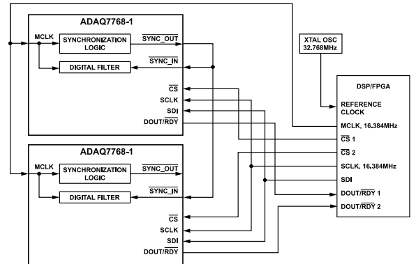
Figure 126. Basic SPI Synchronization Diagram
