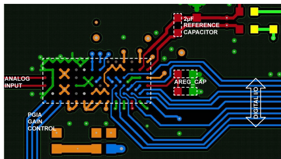
Figure 148. Example Layout of ADAQ7768-1 (Top Layer)
