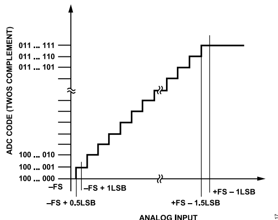
Figure 106. ADC Ideal Transfer Functions (FS is Full-Scale)
