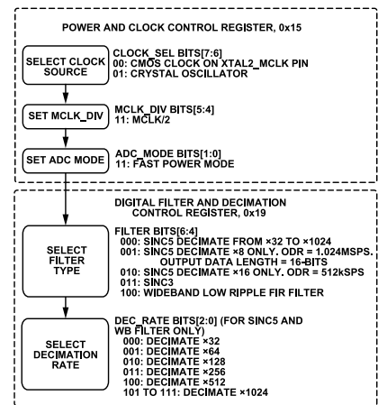
Figure 130. Basic Register Setup for ADAQ7768-1
