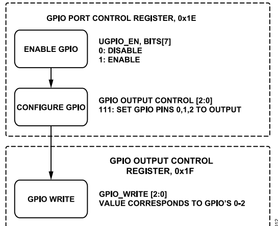
Figure 129. GPIO Gain Control Flowchart
