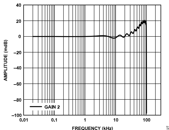
Figure 116. Wideband Low Ripple FIR Filter Magnitude Flatness Response, ODR = 256 kSPS, Gain 2 Mode Normalized
