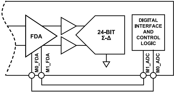
Figure 102. FDA Full-Power Mode Connection
