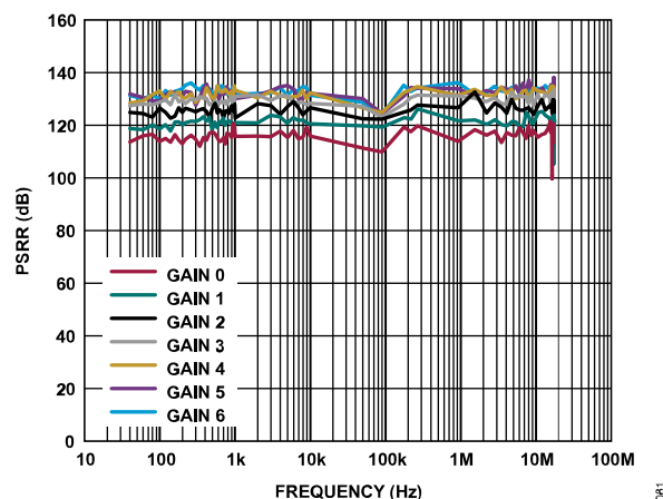
Figure 77. LDO AC PSRR Across All Gain Modes, Connected to VDD2_PGA, VDD_FDA, VDD_ADC, VDD2_ADC with 1 \mu F External Supply Decoupling Capacitor at OUT_LDO
