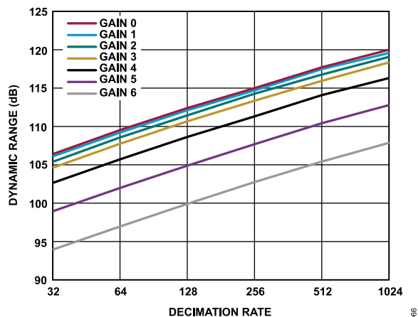
Figure 62. Dynamic Range vs. Decimation Rate Across All Gain Modes, Wideband Low Ripple Filter, Shorted Inputs
