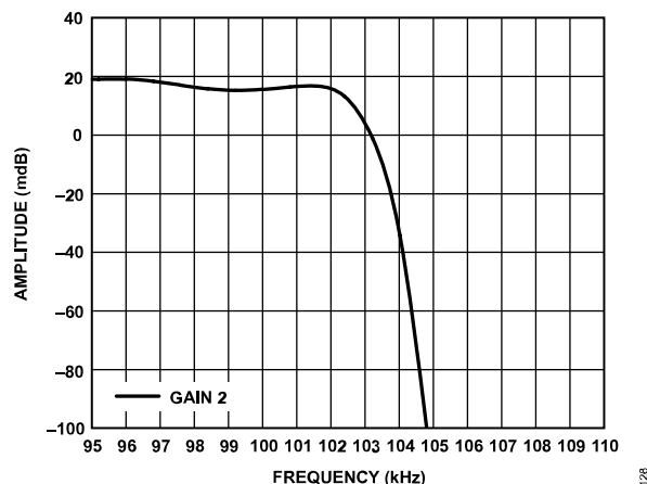
Figure 117. Wideband Low Ripple FIR Filter, -0.1dB Passband
