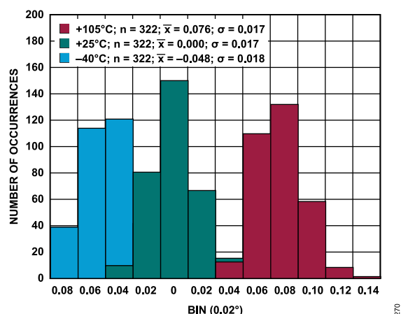
Figure 70. Device-to-Device Phase Angle Mismatch, 20 kHz, AFE_GAIN = 1.3 V/V (Gain 2 Mode), Normalized to the Mean Value at 25°C
