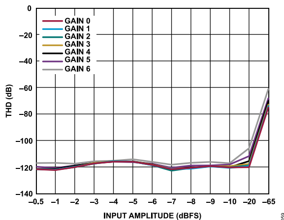
Figure 55. THD vs. Input Amplitude Across All Gain Modes, 1 kHz
