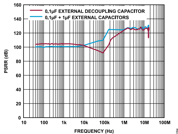
Figure 80. VDD_IO AC PSRR Using External Supply Decoupling Capacitor
