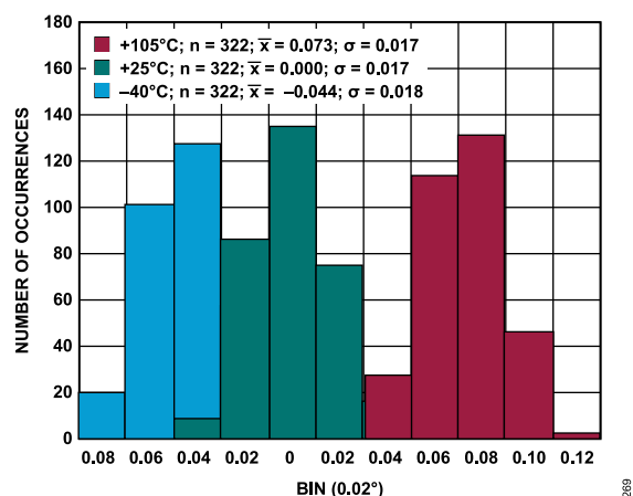
Figure 69. Device-to-Device Phase Angle Mismatch, 20 kHz, AFE_GAIN = 0.65 V/V (Gain 1 Mode), Normalized to the Mean Value at 25°C
