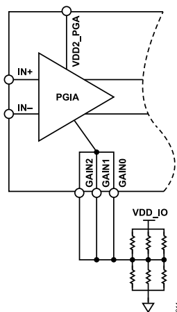
Figure 128. PGIA Gain Control Using External Resistors
