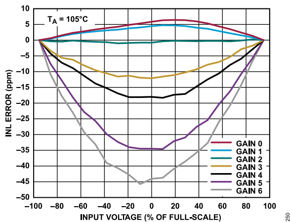
Figure 50. INL Error vs. Input Voltage Across All Gain Modes, Differential Input, Temp = +105°C
