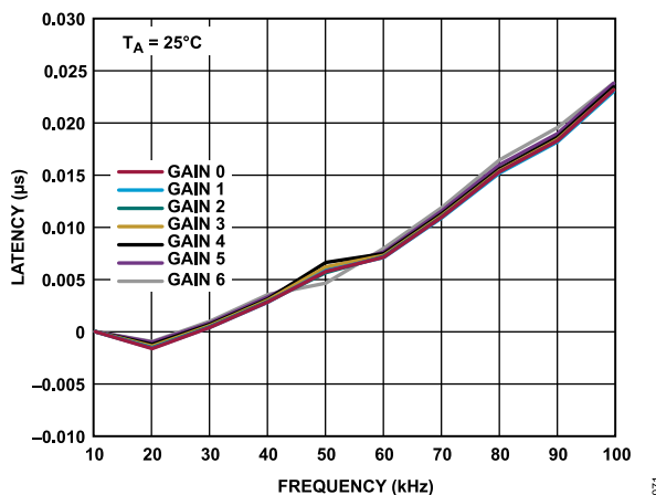
Figure 67. Analog Front-End (AFE) Latency vs. Passband Frequency Across All Gain Modes, at 25°C, Normalized to Latency at 10 kHz
