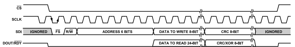
Figure 136. Data Output Format When Using CRC
