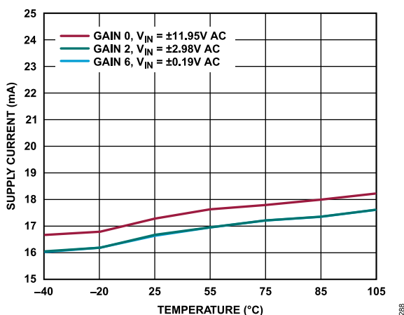
Figure 88. LDO Supply Current vs. Temperature at Various Gain Modes, AC Input, FDA = Low Power, OUT_LDO Connected to VDD2_PGA, VDD_FDA, VDD_ADC, VDD2_ADC
