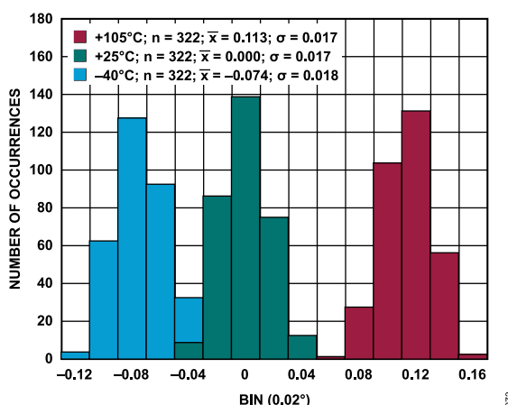
Figure 73. Device-to-Device Phase Angle Mismatch, 20 kHz, AFE_GAIN = 10.4 V/V (Gain 5 Mode), Normalized to the Mean Value at 25°C
