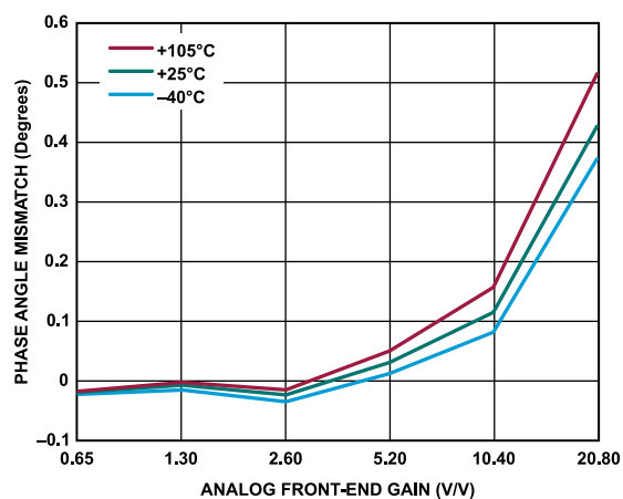
Figure 63. Phase Angle Mismatch vs. Analog Front-End (AFE) Gain over Temperature, Normalized to AFE_GAIN = 0.325 V/V (Gain 0 Mode)
