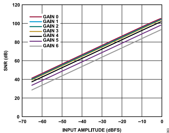
Figure 59. SNR vs. Input Amplitude Across All Gain Modes, 1 kHz
