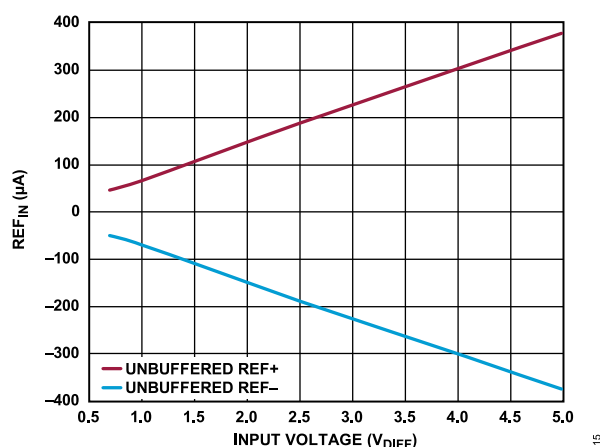
Figure 104. Reference Input Current ( \text{REF}_{\text{IN}} ) vs. Input Voltage, Unbuffered REF+ and REF-
