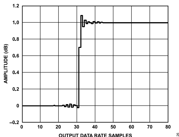
Figure 115. Wideband Low Ripple FIR Filter Step Response
