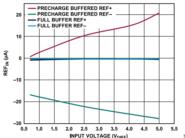
Figure 105. Reference Input Current ( \text{REF}_{\text{IN}} ) vs. Input Voltage, Precharge Buffered REF+ and REF-, and Full Buffer REF+ and REF-
