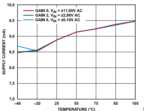
Figure 90. VDD_IO Supply Current vs. Temperature at Various Gain Modes, AC Input
