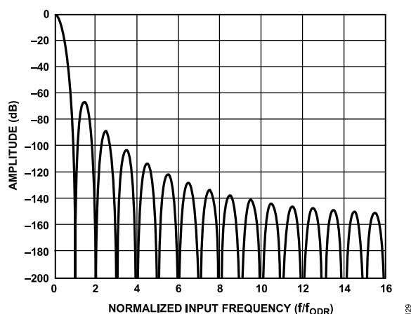
Figure 118. Sinc5 Filter Frequency Response
