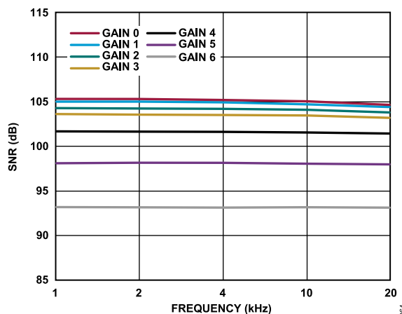
Figure 60. SNR vs. Input Frequency Across All Gain Modes, 1 kHz
