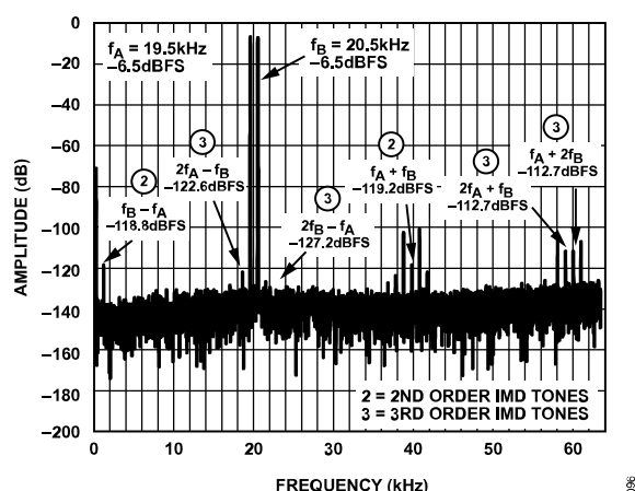
Figure 93. Two-Tone Input, IN+ = -6.5 dBFS, 19.5 kHz Sine, IN- = -6.5 dBFS, 20.5 kHz Sine, ODR = 256 kSPS, V_{REF} = 4.096 V, AFE_GAIN = 0.325 V/V (Gain 0 Mode)
