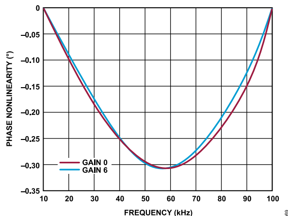
Figure 65. Analog Front-End (AFE) Phase Nonlinearity vs. Passband Frequency at Gain 0 and Gain 6, Endpoint Method (10 kHz to 100 kHz)
