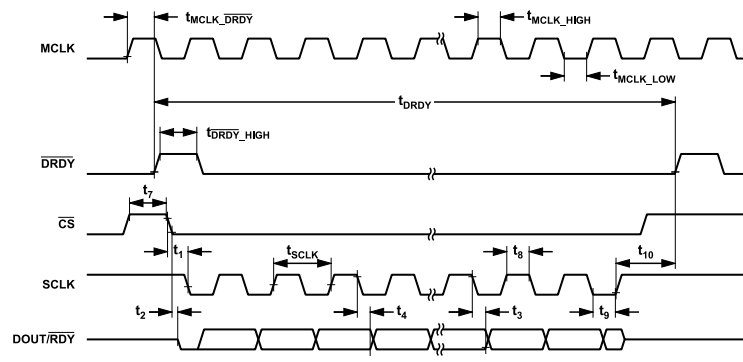
Figure 137. Serial Interface Timing Diagram, Example Reflects Reading an ADC Conversion in the Continuous Read Mode
