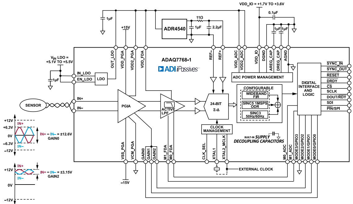
Figure 127. Typical Connection Diagram
