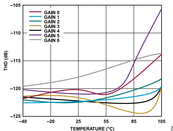
Figure 54. THD vs. Temperature Across All Gain Modes, -0.5 dBFS, 1 kHz
