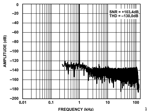
Figure 94. Bipolar Single-Ended Input, IN+ = -0.5 dBFS, 1 kHz Sine, IN- = 0V, ODR = 256 kSPS, V_{REF} = 4.096V, AFE_GAIN = 1.3 V/V (Gain 2 Mode)
