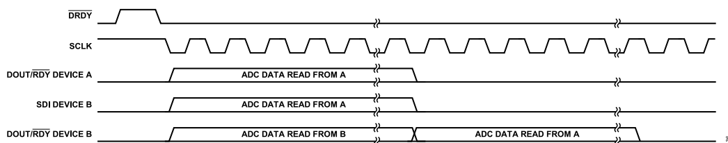
Figure 125. Data Output Format When Devices are Daisy-Chained ( \overline{\text{PIN}} Control Mode Only)
