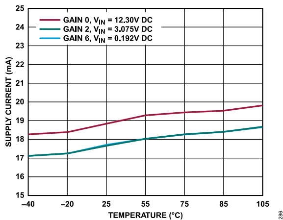
Figure 86. LDO Supply Current vs. Temperature at Various Gain Modes, DC Input, FDA = Low Power, OUT_LDO Connected to VDD2_PGA, VDD_FDA, VDD_ADC, VDD2_ADC
