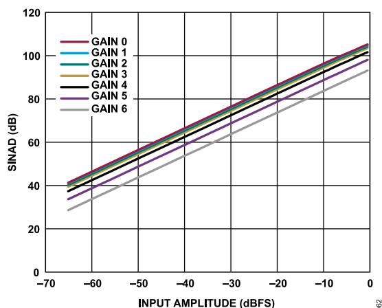
Figure 58. SINAD vs. Input Amplitude Across All Gain Modes, 1 kHz
