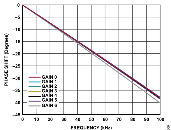
Figure 64. Analog Front-End (AFE) Phase Response Across All Gain Modes at 25°C
