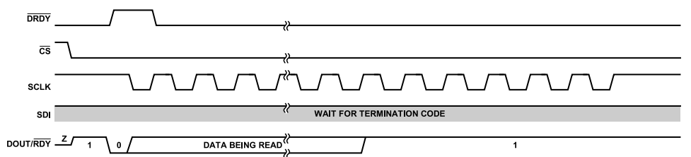
Figure 139. Continuous ADC Read Data Format with \overline{\text{RDY}} Function Enabled on the DOUT/ \overline{\text{RDY}} Pin
