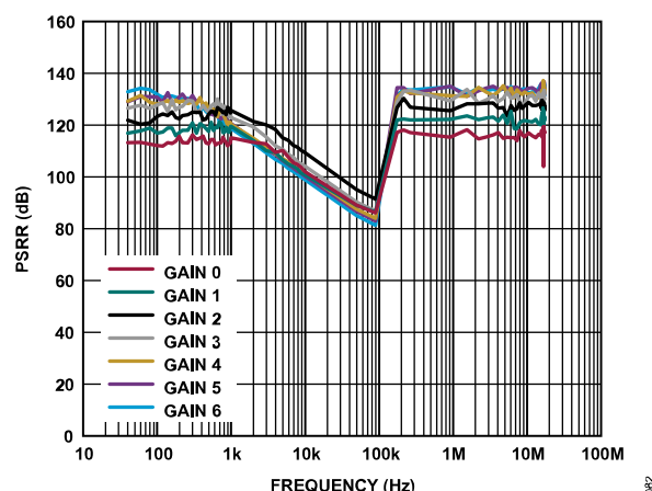
Figure 78. VDD_PGA AC PSRR Across All Gain Modes, Using the Internal Supply Decoupling Capacitor Only
