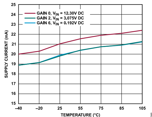
Figure 85. LDO Supply Current vs. Temperature at Various Gain Modes, DC Input, FDA = Full Power, OUT_LDO Connected to VDD2_PGA, VDD_FDA, VDD_ADC, VDD2_ADC
