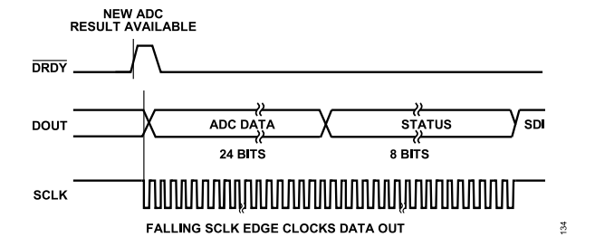
Figure 123. \overline{\text{PIN}} Mode Data Output Format (Without the \overline{\text{CS}} Signal)
