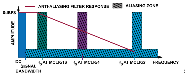
Figure 122. Anti-Alias Filter Response vs. MCLK Divider
