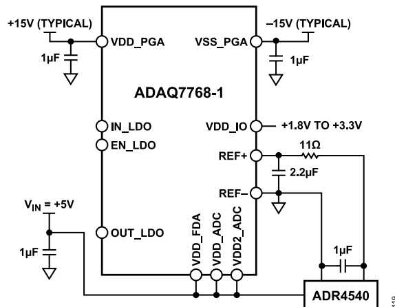
Figure 108. ADAQ7768-1 Power Supply Connection Using External 5 V Supply
