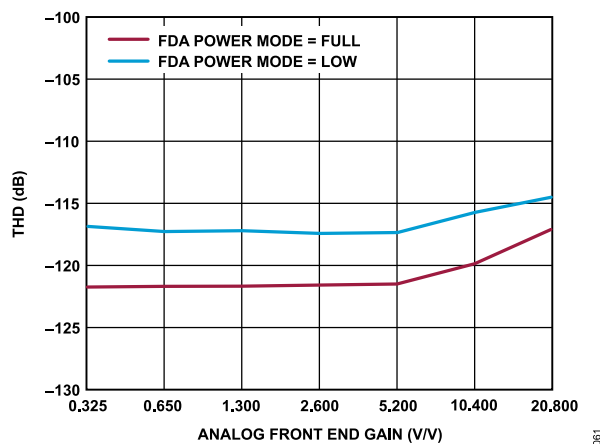
Figure 57. THD vs. Analog Front-End (AFE) Gain over FDA Power Mode, -0.5 dBFS, 1 kHz
