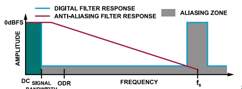
Figure 101. Simplified Illustration of the Overall Frequency Response
