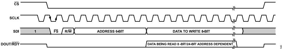
Figure 133. SPI Basic Read/Write Frame
