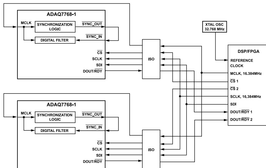
Figure 144. Synchronization in Channel-to-Channel Isolated Systems
