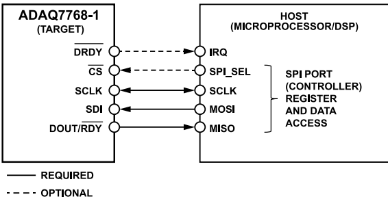
Figure 131. Basic Serial Port Connection Diagram
