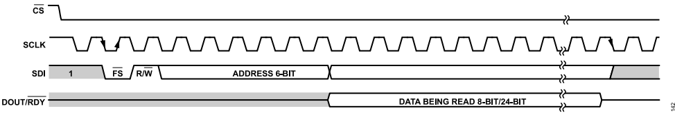
Figure 135. 3-Wire SPI Read Frame ( \overline{CS} = 0 )
