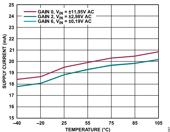
Figure 87. LDO Supply Current vs. Temperature at Various Gain Modes, AC Input, FDA = Full Power, OUT_LDO Connected to VDD2_PGA, VDD_FDA, VDD_ADC, VDD2_ADC
