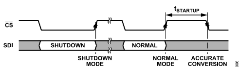
Figure 6. Shutdown Mode to Normal Mode Timing
