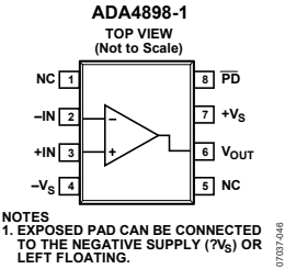
Figure 5. Single 8-Lead SOIC_N_EP Pin Configuration
