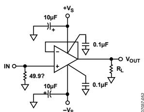
Figure 38. Typical Noninverting Load Configuration
