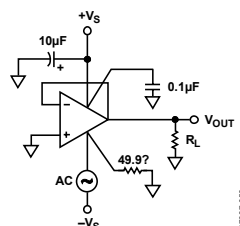
Figure 41. Typical Capacitive Load Configuration
