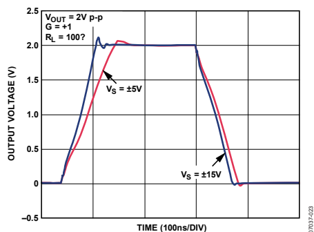
Figure 25. Small Signal Transient Response for Various Gains
