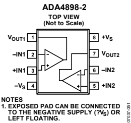
Figure 6. Dual 8-Lead SOIC_N_EP Pin Configuration
