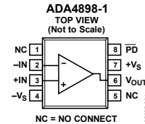
Figure 1. Single 8-Lead ADA4898-1 SOIC_N_EP (RD-8-4)
