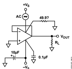
Figure 38. Typical Noninverting Load Configuration
