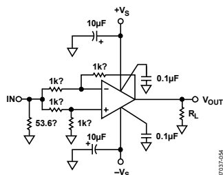
Figure 39. Positive Power Supply Rejection
