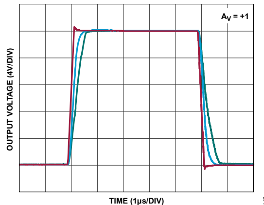
Figure 137. 20 V Step into ADA4620 in A_V = +1 . Red is 80 V/ \mu s Input Pulse, Blue is After 330 \Omega , 330 pF RC into the +IN Pin, Green is Well-Behaved Output
