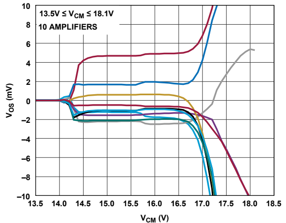
Figure 23. V_{OS} vs. V_{CM} , High V_{CM} Operation
