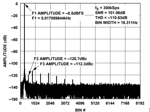
Figure 128. 8192 Bin FFT Gathered from the Circuit at 300 kSps, -0.5 dBFS, 5.017 kHz Input Sinusoid
