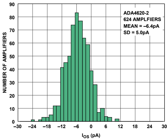
Figure 45. ADA4620-2 I_{os} Distribution (+125°C)
