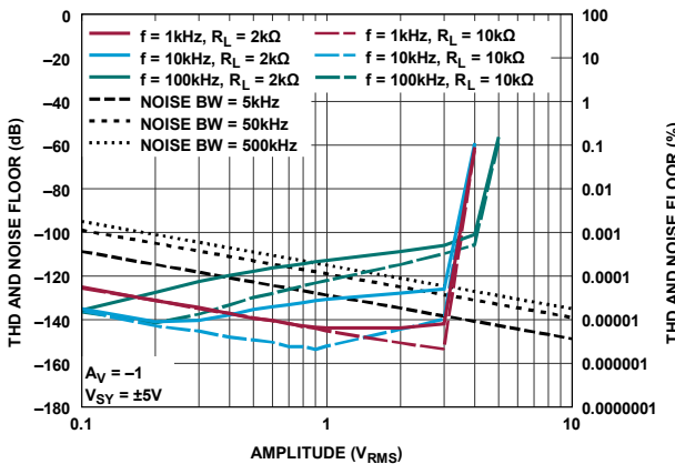
Figure 99. ADA4620-2 THD vs. Amplitude vs. R_L ( A_V = -1 , V_{SY} = \pm 5V )
