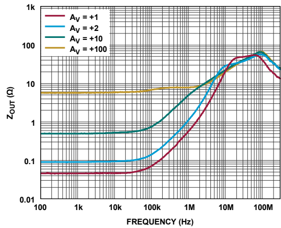
Figure 69. Closed-Loop Output Impedance ( Z_{OUT} ) vs. Frequency, High V_{CM} Operation
