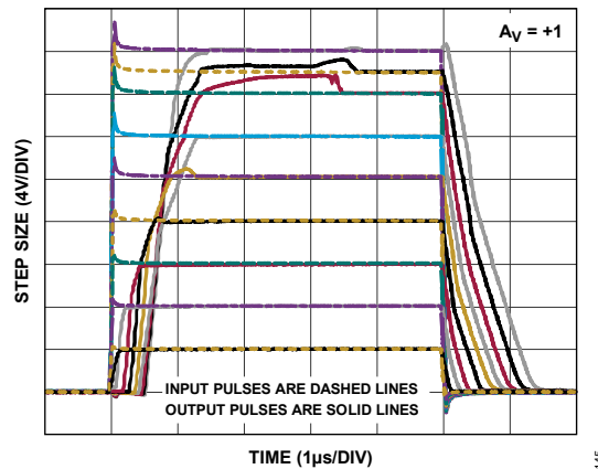
Figure 135. Large Signal Noninverting Output Behavior, Without Input RC
