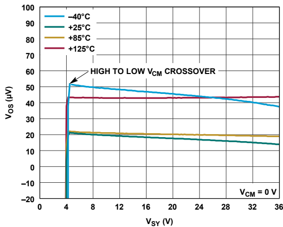
Figure 28. V_{OS} vs. V_{SY} , Single Supply, Four Temperatures
