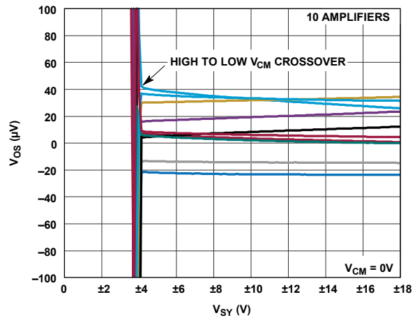
Figure 27. V_{OS} vs. V_{SY} , Dual Supply
