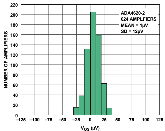
Figure 11. ADA4620-2 V_{OS} Distribution ( +85^\circ\text{C} )
