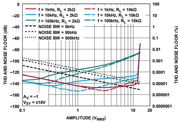
Figure 97. ADA4620-2 THD vs. Amplitude vs. R_L ( A_V = -1 )
