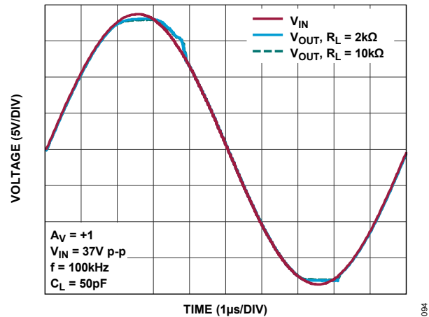
Figure 93. No Phase Reversal (Sine Freq. = 100 kHz)
