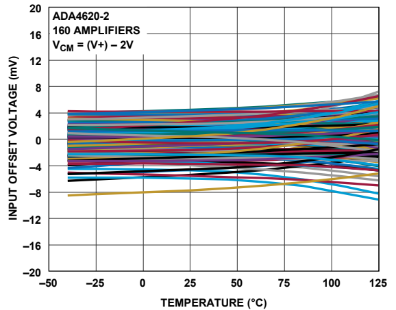
Figure 19. ADA4620-2 V_{OS} vs. Temperature, High V_{CM} Operation
