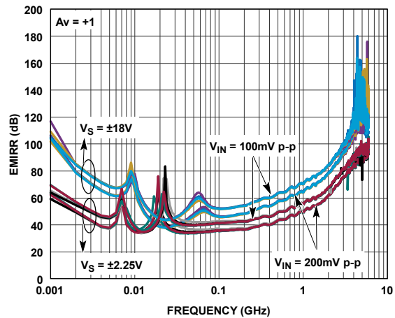
Figure 71. EMIRR vs. Frequency
