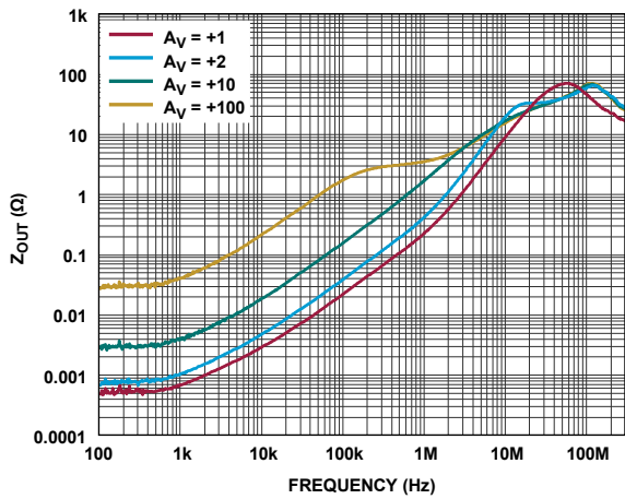
Figure 68. Closed-Loop Output Impedance ( Z_{OUT} ) vs. Frequency
