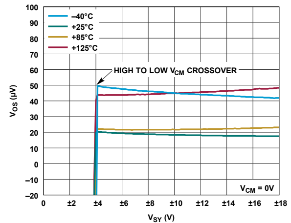
Figure 29. V_{OS} vs. V_{SY} , Dual Supply, Four Temperatures
