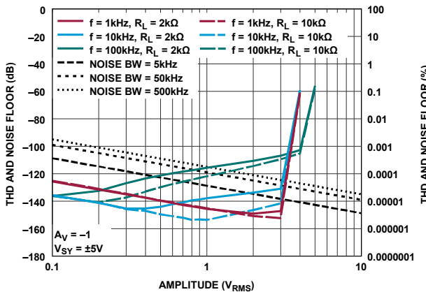
Figure 98. ADA4620-1 THD vs. Amplitude vs. R_L ( A_V = -1 , V_{SY} = \pm 5V )
