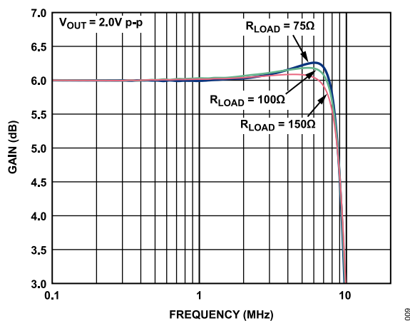
Figure 27. 1 dB Flatness Response at Various Load Resistances
