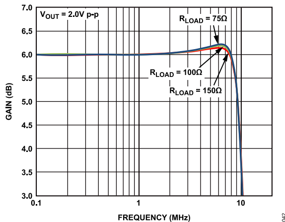
Figure 9. 1 dB Flatness Response at Various Load Resistances
