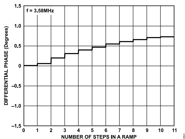
Figure 16. Differential Phase Plot
