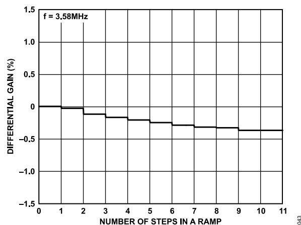
Figure 13. Differential Gain Plot
