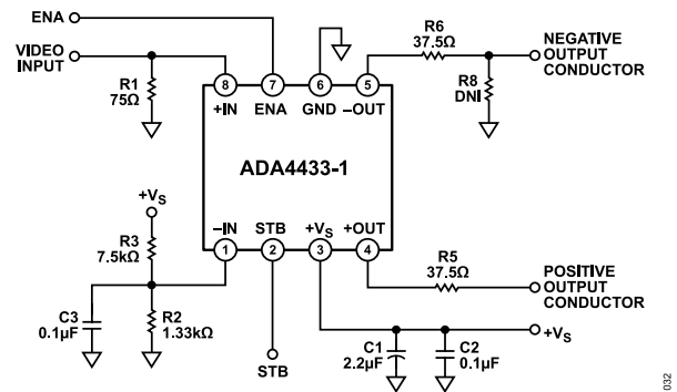
Figure 51. Example Compatible Schematic Configured for the ADA4433-1
