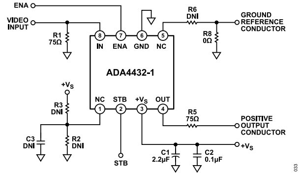
Figure 49. Example Compatible Schematic Configured for the ADA4432-1
