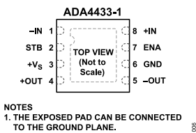
Figure 6. ADA4433-1 8-Lead LFCSP Pin Configuration, Top View
