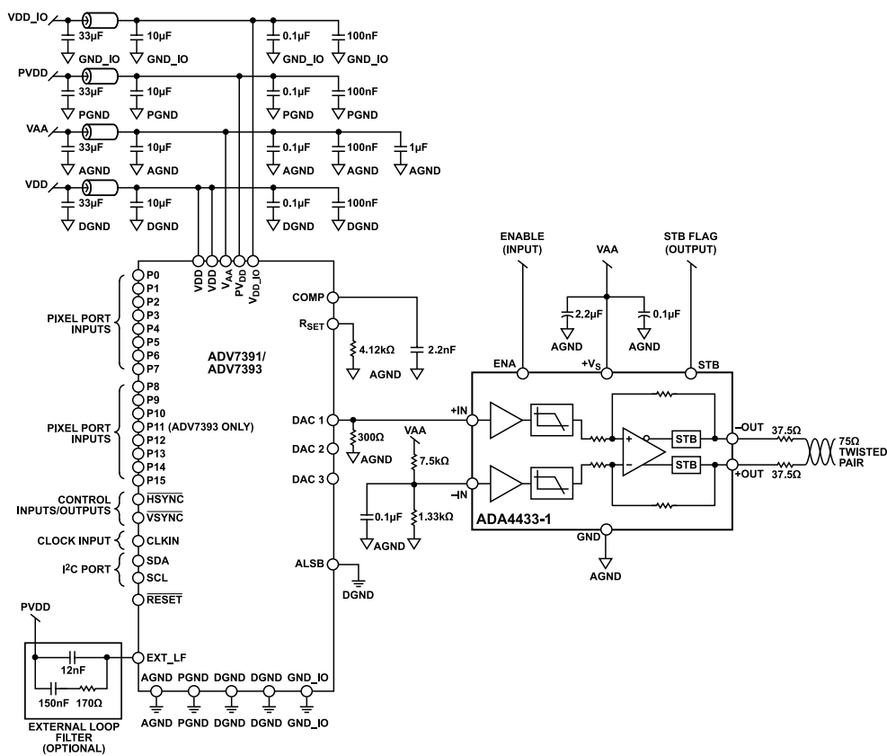
Figure 53. ADA4433-1 and ADV7391/ADV7393 Video Encoder Application Circuit
