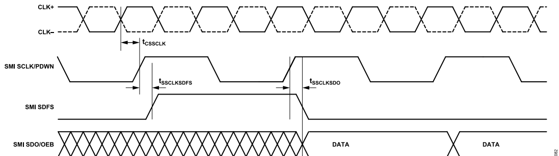
Figure 5. Signal Monitor SPORT Output Timing (Divide-by-2 Mode)
