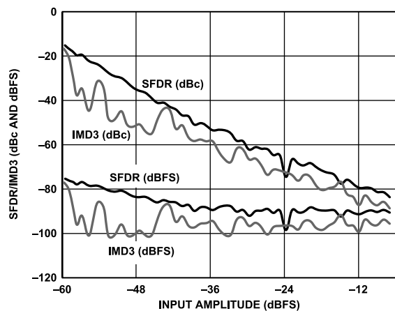
Figure 33. AD9600-150 Two-Tone SFDR/IMD3 vs. Input Amplitude ( A_{IN} ) with f_{IN1} = 29.1 MHz, f_{IN2} = 32.1 MHz, f_s = 150 MSPS
