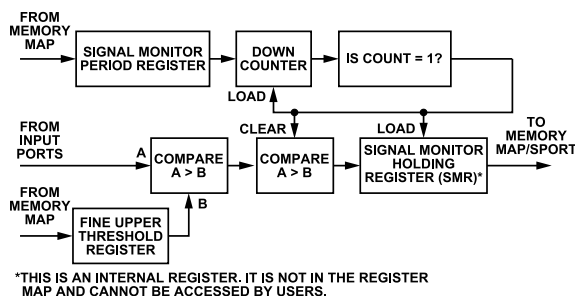
Figure 69. ADC Input Threshold Crossing Block Diagram
