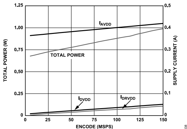
Figure 63. AD9600-150 Power and Current vs. Sample Rate
