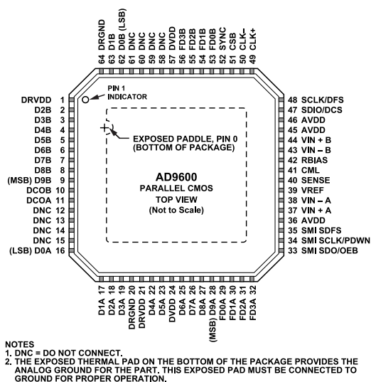
Figure 6. Parallel CMOS Mode Pin Configuration (Top View)
