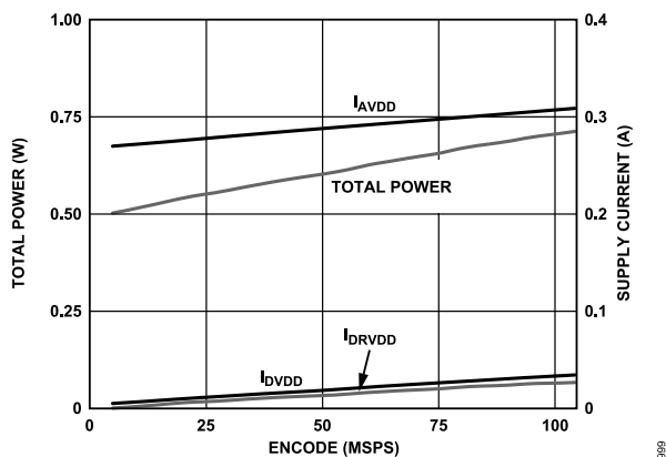
Figure 65. AD9600-105 Power and Current vs. Sample Rate
