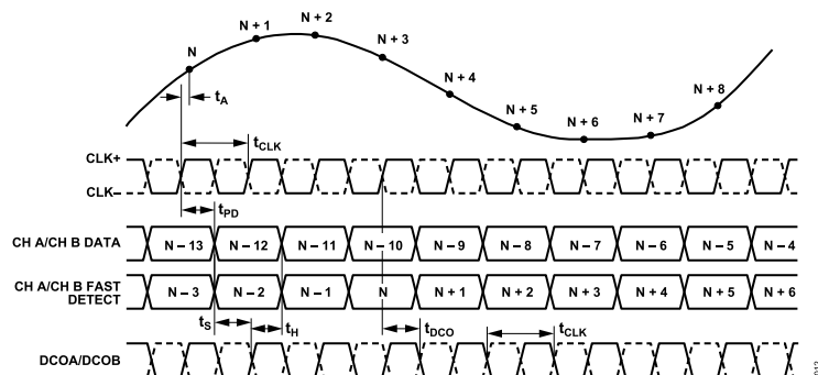
Figure 2. CMOS Output Mode Data and Fast Detect Output Timing
