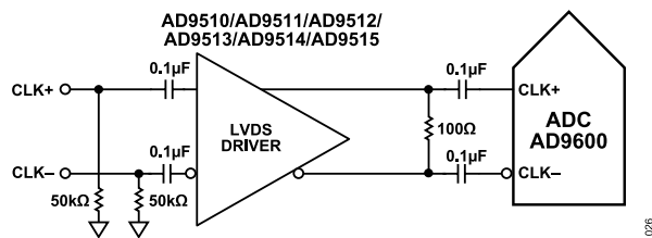
Figure 59. Differential LVDS Sample Clock (up to 150 MSPS)
