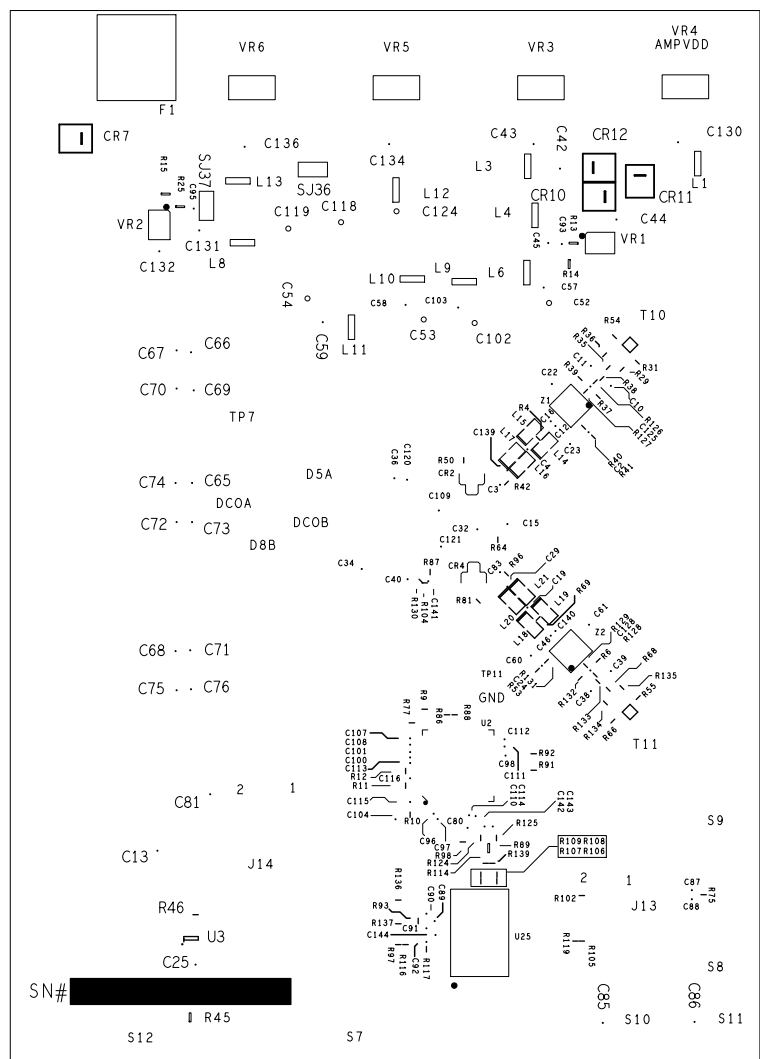
Figure 91. Evaluation Board Layout, Silk Screen, Secondary Side
