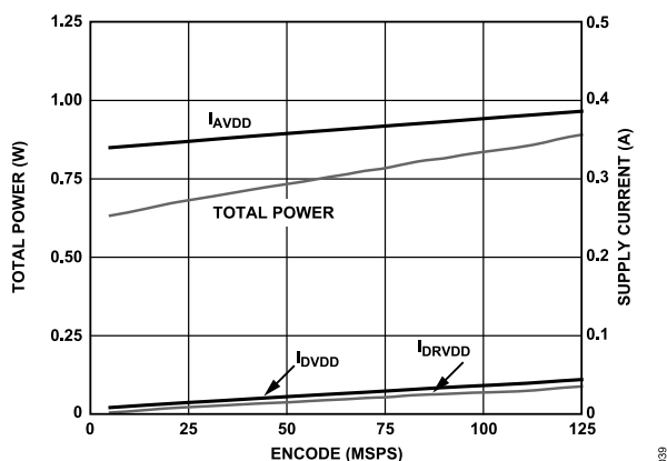
Figure 64. AD9600-125 Power and Current vs. Sample Rate
