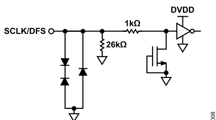
Figure 12. Equivalent SCLK/DFS Input Circuit
