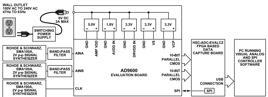
Figure 73. Evaluation Board Connection
