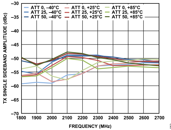
Figure 52. TX Single Sideband (SSB) Rejection vs. Frequency, 3.075 MHz Offset
