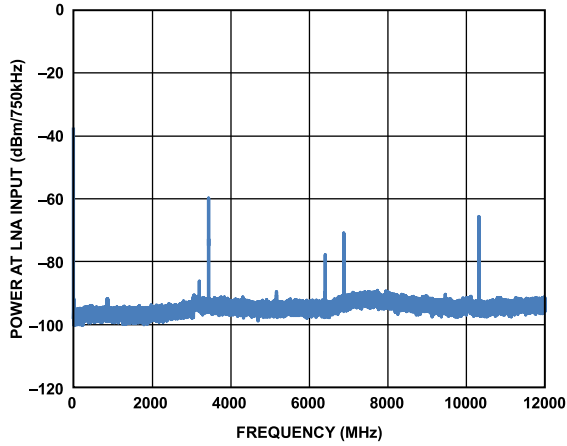
Figure 15. RX Emission at LNA Input, DC to 12 GHz, f_{LO\_RX} = 800 MHz, LTE 10 MHz, f_{LO\_TX} = 860 MHz
