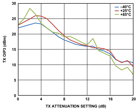
Figure 28. TX Third-Order Output Intercept Point (OIP3) vs. TX Attenuation Setting
