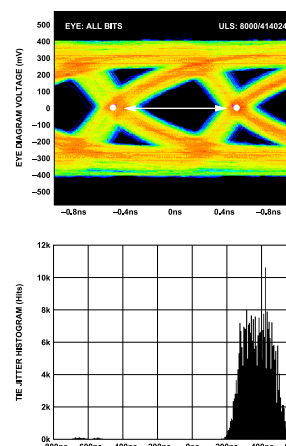
Figure 73. Data Eye for LVDS Outputs in ANSI-644 Mode with Trace Lengths Greater than 24 Inches on Standard FR-4 Material, External 100 \Omega Far-End Termination Only
