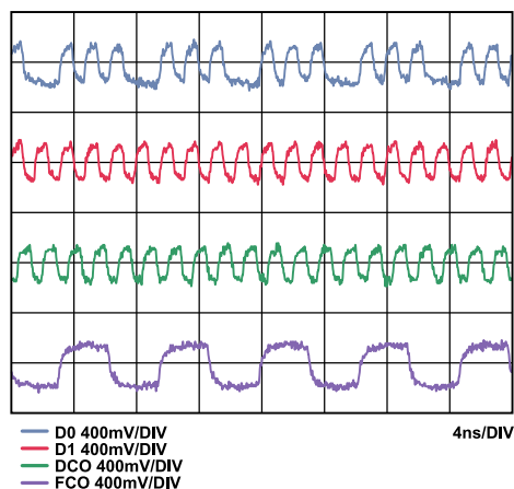
Figure 71. AD9253-125, LVDS Output Timing Example in Reduced Range Mode
