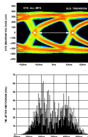
Figure 72. Data Eye for LVDS Outputs in ANSI-644 Mode with Trace Lengths Less than 24 Inches on Standard FR-4 Material, External 100 \Omega Far-End Termination Only
