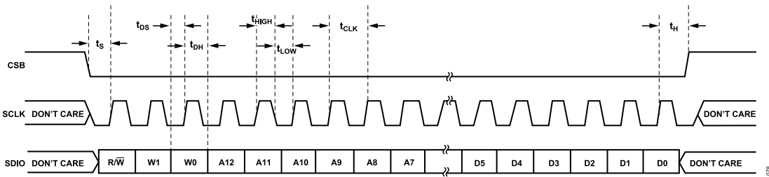
Figure 74. Serial Port Interface Timing Diagram
