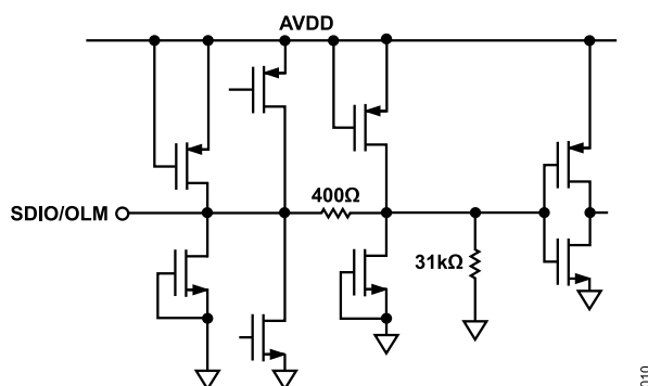
Figure 49. Equivalent SDIO/OLM Input Circuit
