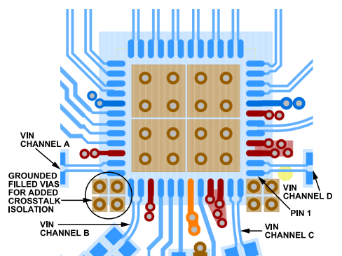
Figure 76. Layout Technique to Maximize Crosstalk Performance
