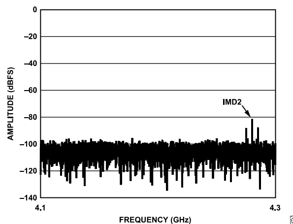
Figure 31. Two-Tone FFT, IMD2 Zoom In, f_{IN1} = 2137.5 MHz, f_{IN2} = 2142.5 MHz, A_{IN1} and A_{IN2} = -7 dBFS (See Figure 30), 10 GSPS
