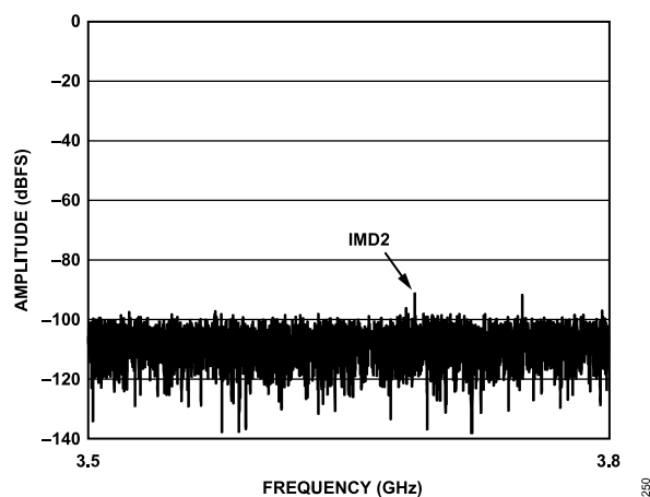
Figure 28. Two-Tone FFT, IMD2 Zoom In, f_{IN1} = 1841.5 MHz, f_{IN2} = 1846.5 MHz, A_{IN1} and A_{IN2} = -15 dBFS (See Figure 27), 10 GSPS
