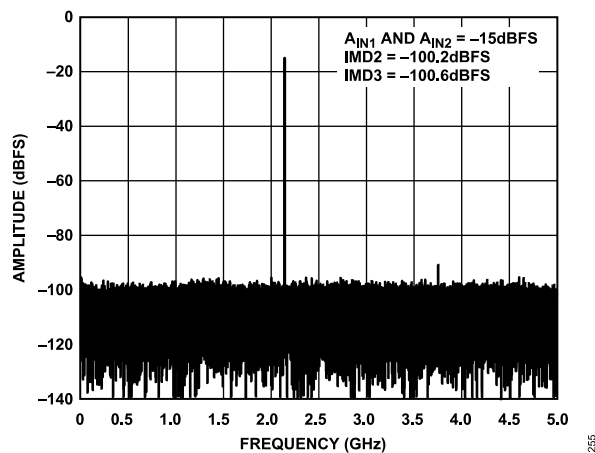
Figure 33. Two-Tone FFT, f_{IN1} = 2137.5 MHz, f_{IN2} = 2142.5 MHz, A_{IN1} and A_{IN2} = -15 dBFS, 10 GSPS
