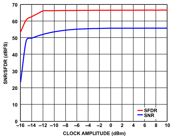
Figure 20. SNR/SFDR vs. Clock Amplitude, f_{IN} = 1000 MHz, 10 GSPS
