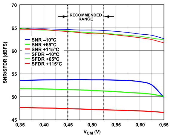
Figure 19. SNR/SFDR vs. V_{CM} , 10 GSPS, Temperatures
