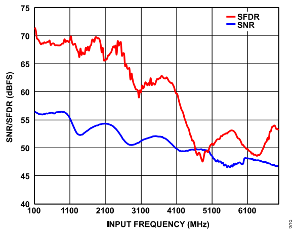
Figure 18. SNR/SFDR vs. Input Frequency ( f_{IN} ), 10 GSPS, A_{IN} = -1 dBFS
