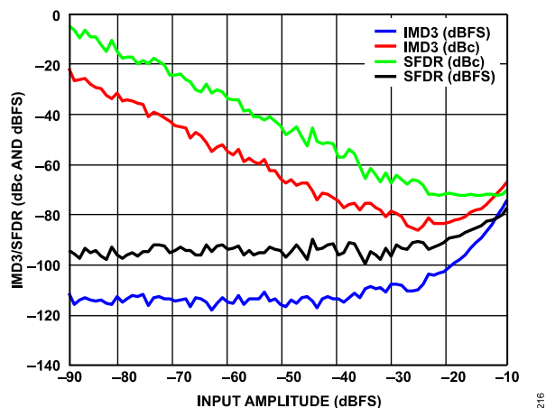
Figure 37. IMD3/SFDR vs. Input Amplitude, f_{IN1} = 2137.5 MHz, f_{IN2} = 2142.5 MHz, 10 GSPS
