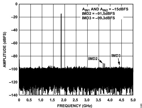
Figure 27. Two-Tone FFT, f_{IN1} = 1841.5 MHz, f_{IN2} = 1846.5 MHz, A_{IN1} and A_{IN2} = -15 dBFS, 10 GSPS
