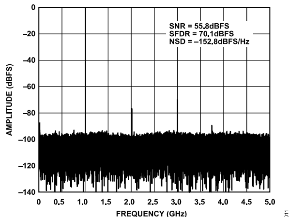
Figure 4. Single-Tone FFT with f_{IN} = 1 GHz, 10 GSPS
