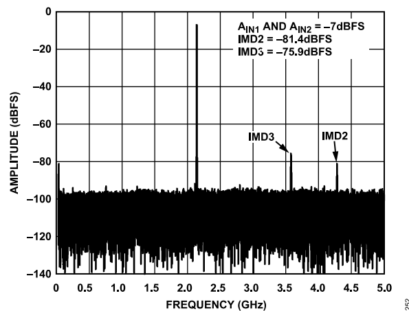
Figure 30. Two-Tone FFT, f_{IN1} = 2137.5 MHz, f_{IN2} = 2142.5 MHz, A_{IN1} and A_{IN2} = -7 dBFS, 10 GSPS
