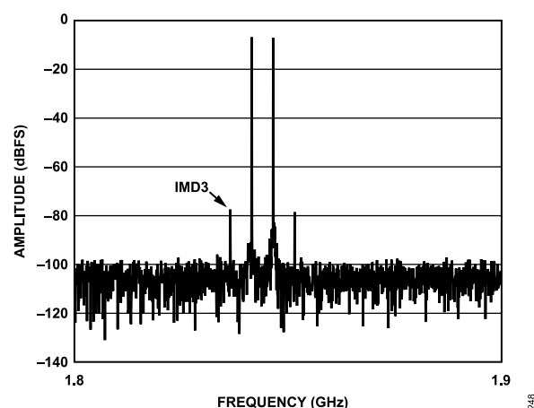
Figure 25. Two-Tone FFT, IMD3 Zoom In, f_{IN1} = 1841.5 MHz, f_{IN2} = 1846.5 MHz, A_{IN1} and A_{IN2} = -7 dBFS (See Figure 24ph>), 10 GSPS
