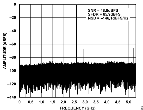
Figure 10. Single Tone FFT with f_{IN} = 2.6 GHz, 10.75 GSPS
