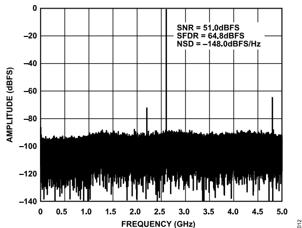
Figure 5. Single-Tone FFT with f_{IN} = 2.6 GHz, 10 GSPS
