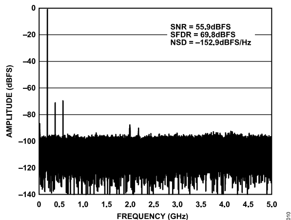
Figure 3. Single-Tone FFT with f_{IN} = 170 MHz, 10 GSPS
