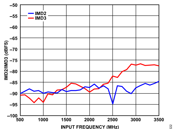
Figure 38. IMD2/IMD3 vs. Input Frequency, ( A_{IN} = -7 dBFS), 100 MHz Spacing, 10 GSPS
