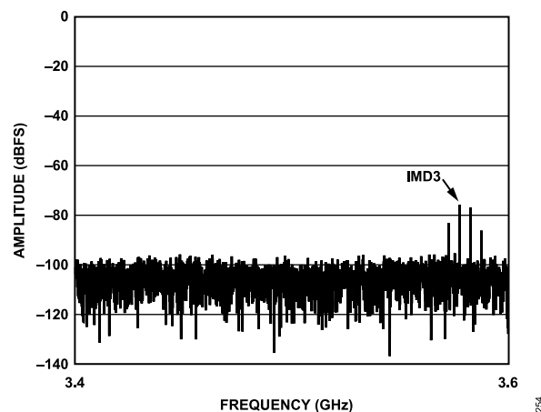
Figure 32. Two-Tone FFT, IMD3 Zoom In, f_{IN1} = 2137.5 MHz, f_{IN2} = 2142.5 MHz, A_{IN1} and A_{IN2} = -7 dBFS (See Figure 30), 10 GSPS
