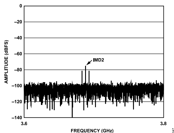
Figure 26. Two-Tone FFT, IMD2 Zoom In, f_{IN1} = 1841.5 MHz, f_{IN2} = 1846.5 MHz, A_{IN1} and A_{IN2} = -7 dBFS (See Figure 24), 10 GSPS
