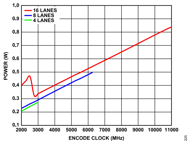
Figure 12. Power vs. Encode Clock ( f_s ) for a Various Number of JESD204B Lanes, f_{IN} = 170 MHz, 10 GSPS
