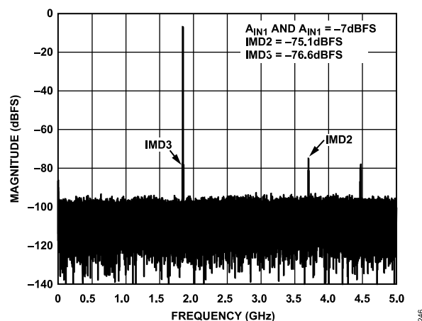
Figure 24. Two-Tone FFT, f_{IN1} = 1841.5 MHz, f_{IN2} = 1846.5 MHz, A_{IN1} and A_{IN2} = -7 dBFS, 10 GSPS
