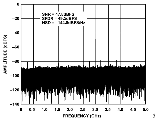
Figure 8. Single-Tone FFT with f_{IN} = 6.5 GHz, 10 GSPS
