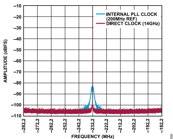
Figure 102. ADC Direct Clock vs Internal PLL Clock with 200MHz Reference Frequency at 2.267GHz Analog Input Frequency
