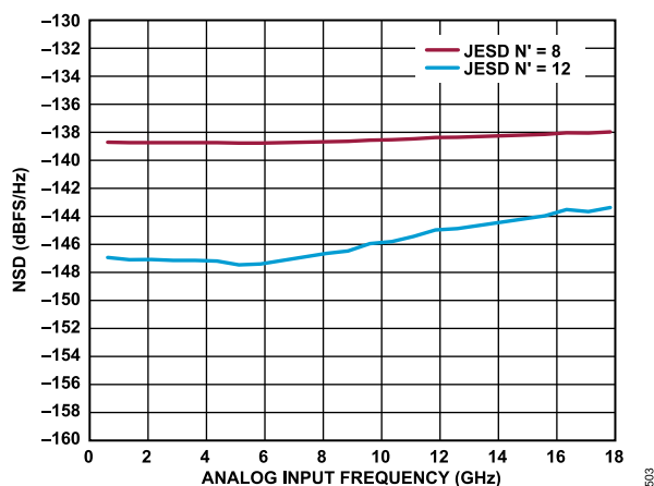
Figure 91. Single-Tone NSD vs Analog Input Frequency at -7\text{dBFS} , Multiple JESDN' Settings
