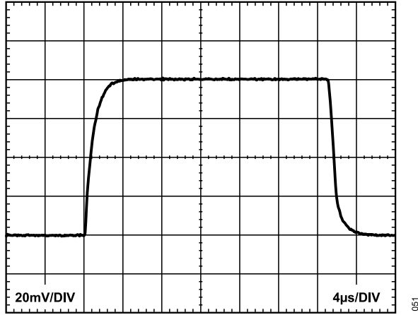
Figure 51. Small Signal Pulse Response, G = 1 , R_L = 20\text{ k}\Omega , C_L = 100\text{ pF}
