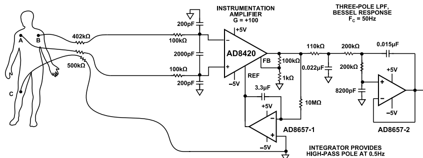
Figure 69. AD8420 in an ECG Front End
