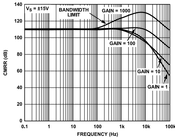
Figure 28. CMRR vs. Frequency, RTI, V_S = \pm 15 V
