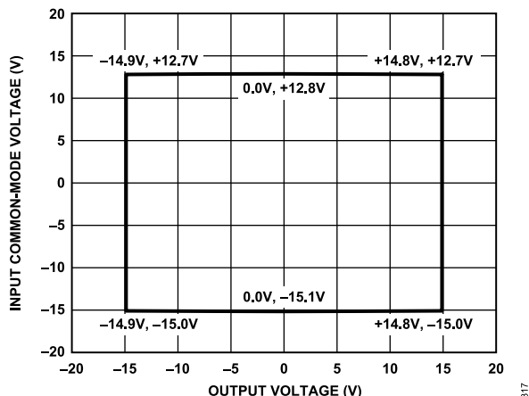
Figure 17. Input Common-Mode Voltage vs. Output Voltage, G = 100 , V_S = \pm 15 V
