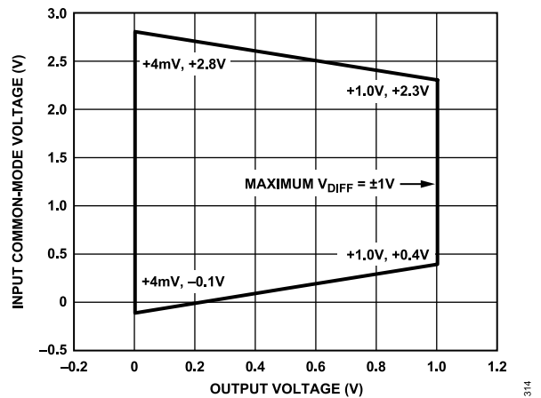
Figure 14. Input Common-Mode Voltage vs. Output Voltage, G = 1, V S = 5 V, V REF = 0 V
