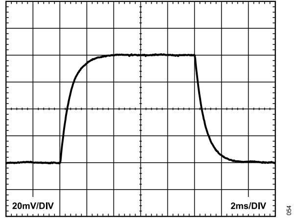
Figure 54. Small Signal Pulse Response, G = 1000 , R_L = 20\text{ k}\Omega , C_L = 100\text{ pF}
