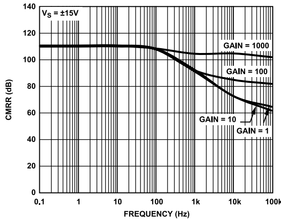
Figure 29. CMRR vs. Frequency, RTI, 1 k \Omega Source Imbalance, V_S = \pm 15 V
