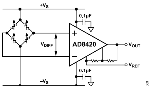
Figure 70. Classic Bridge Circuit
