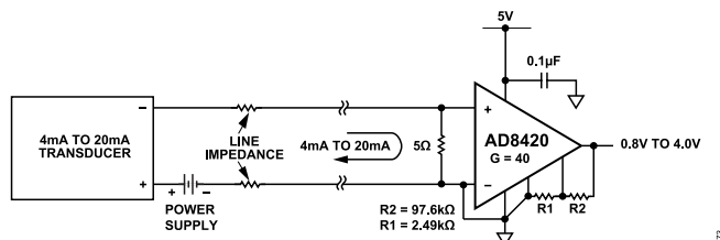
Figure 71. 4 mA to 20 mA Receiver Circuit
