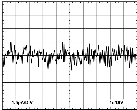
Figure 46. 0.1 Hz to 10 Hz Current Noise
