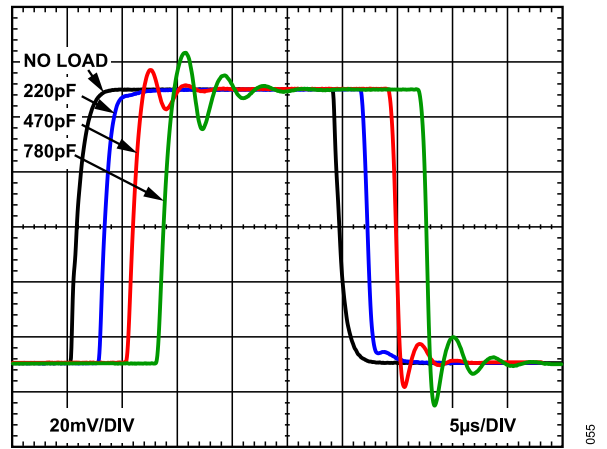
Figure 55. Small Signal Response with Various Capacitive Loads, G = 1 , R_L = \infty
