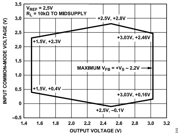
Figure 15. Input Common-Mode Voltage vs. Output Voltage, G = 1 , V_S = 5 V , V_{REF} = 2.5 V
