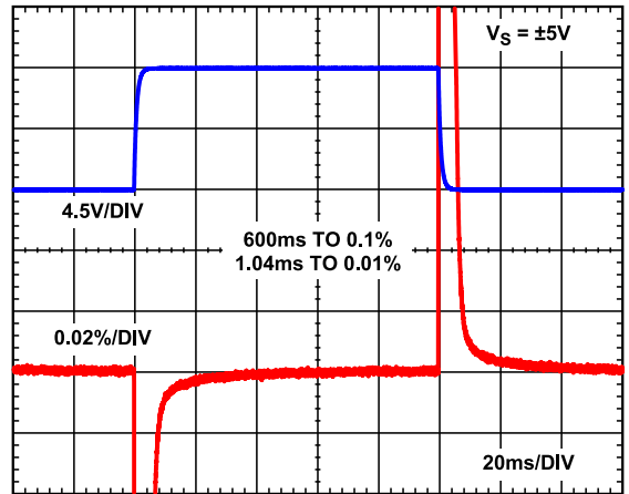
Figure 50. Large Signal Pulse Response and Settling Time, G = 100
