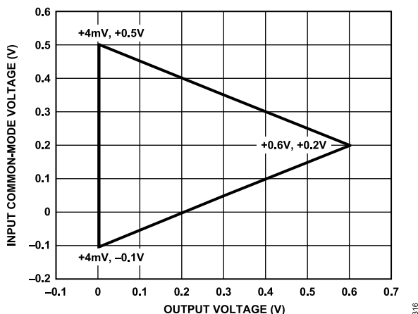
Figure 16. Input Common-Mode Voltage vs. Output Voltage, G = 1 , V_S = 2.7 V , V_{REF} = 0 V
