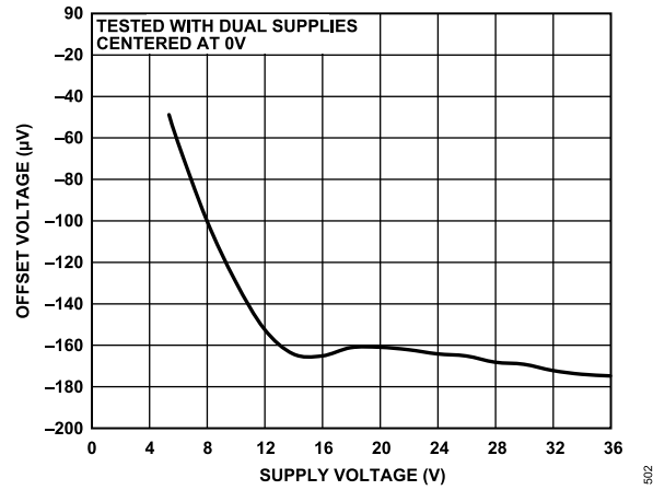
Figure 57. Offset Voltage vs. Total Supply Voltage
