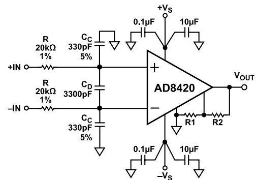
Figure 66. Suggested RFI Suppression Filter
