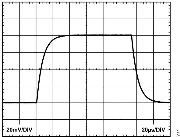
Figure 52. Small Signal Pulse Response, G = 10 , R_L = 20\text{ k}\Omega , C_L = 100\text{ pF}
