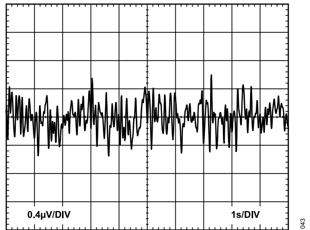
Figure 44. 0.1 Hz to 10 Hz RTI Voltage Noise, G = 1
