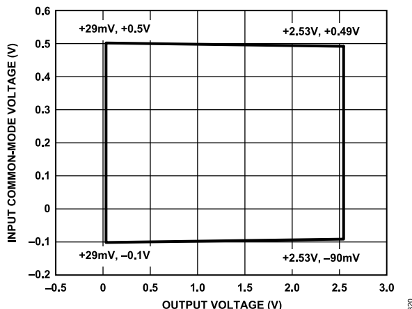
Figure 20. Input Common-Mode Voltage vs. Output Voltage, G = 100 , V_S = 2.7 V , V_{REF} = 0 V
