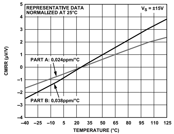
Figure 37. CMRR vs. Temperature, G = 1 , V_S = \pm 15\text{ V}
