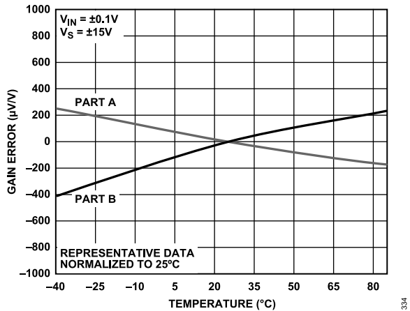
Figure 35. Gain Error vs. Temperature, G = 1 , V_{IN} = \pm 0.1\text{ V} , V_S = \pm 15\text{ V}
