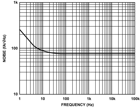
Figure 45. Current Noise Spectral Density vs. Frequency
