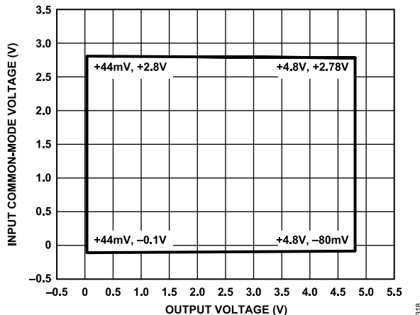
Figure 18. Input Common-Mode Voltage vs. Output Voltage, G = 100 , V_S = 5 V , V_{REF} = 0 V
