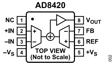
Figure 2. Pin Configuration
