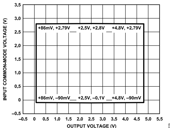
Figure 19. Input Common-Mode Voltage vs. Output Voltage, G = 100 , V_S = 5 V , V_{REF} = 2.5 V
