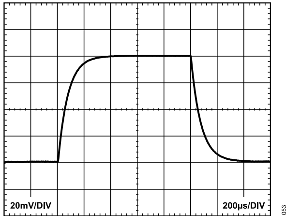
Figure 53. Small Signal Pulse Response, G = 100 , R_L = 20\text{ k}\Omega , C_L = 100\text{ pF}
