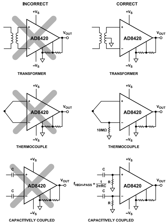
Figure 65. Creating an I BIAS Path
