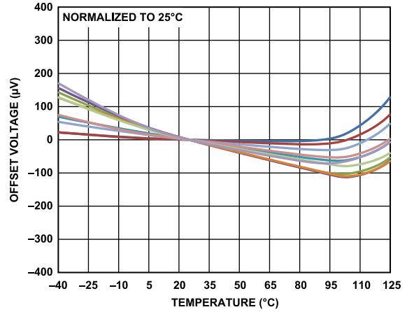
Figure 36. Offset Drift
