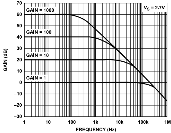
Figure 27. Gain vs. Frequency, 2.7 V Single Supply
