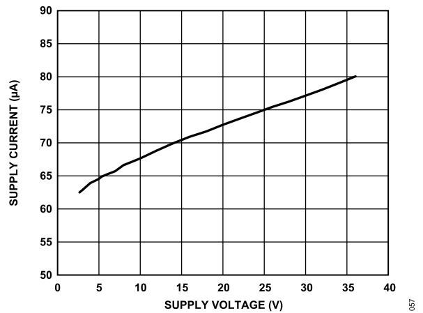
Figure 56. Supply Current vs. Total Supply Voltage
