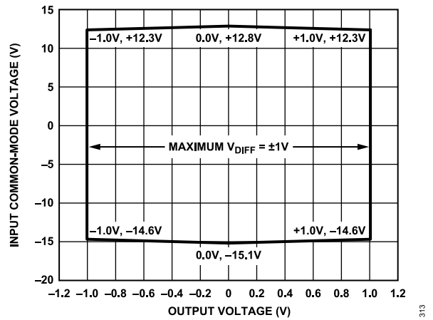
Figure 13. Input Common-Mode Voltage vs. Output Voltage, G = 1, V S = ±15 V
