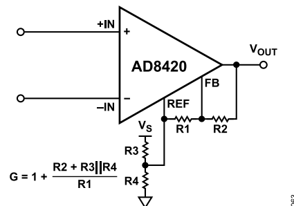
Figure 64. Using Resistor Divider to Set Reference Voltage
