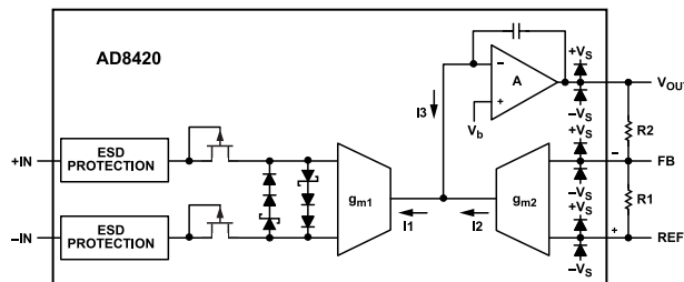
Figure 58. Simplified Schematic
