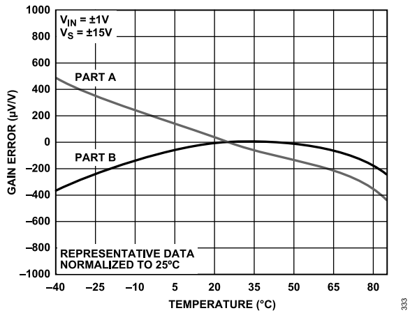
Figure 34. Gain Error vs. Temperature, G = 1 , V_{IN} = \pm 1\text{ V} , V_S = \pm 15\text{ V}
