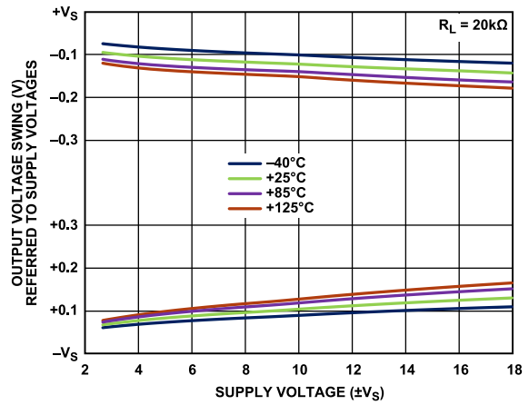
Figure 38. Output Voltage Swing vs. Supply Voltage, R_L = 20\text{ k}\Omega
