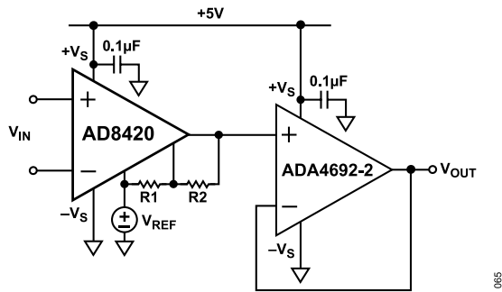
Figure 67. Output Buffering
