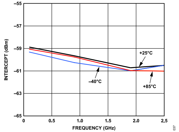
Figure 23. Intercept vs. Frequency -40°C, +25°C, and +85°C
