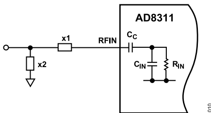
Figure 34. Narrow Band Reactive Input Coupling Option
