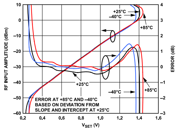
Figure 8. Input Amplitude and Log Conformance vs. V SET at 2.5 GHz -40°C, +25°C, and +85°C
