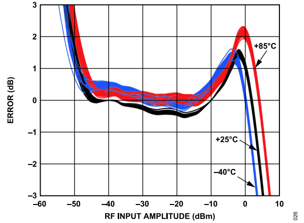
Figure 12. Distribution of Error over Temperature After Ambient Normalization vs. Input Amplitude at 1.9 GHz
