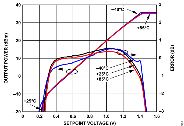
Figure 32. P_{OUT} vs. V_{SET} at 0.9 GHz for Dual Mode Handset Power Amplifier Application; -40°C, +25°C, and +85°C
