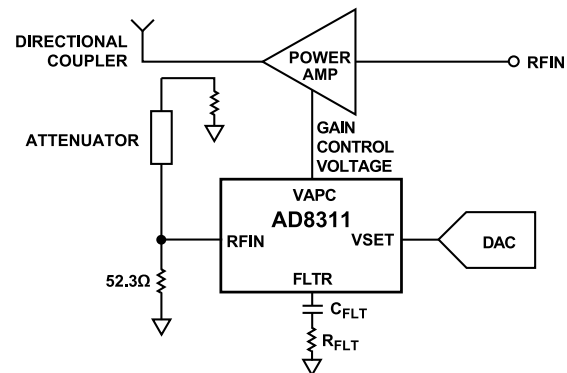
Figure 30. Typical Application
