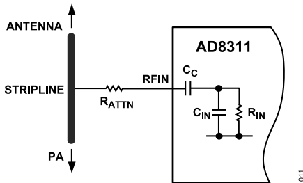
Figure 35. Series Attention Input Coupling Option
