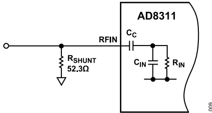
Figure 33. Broadband Resistive Input Coupling Option
