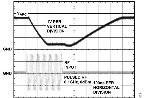
Figure 18. V_{APC} Response Time, Full-Scale Amplitude Change, Open-Loop
