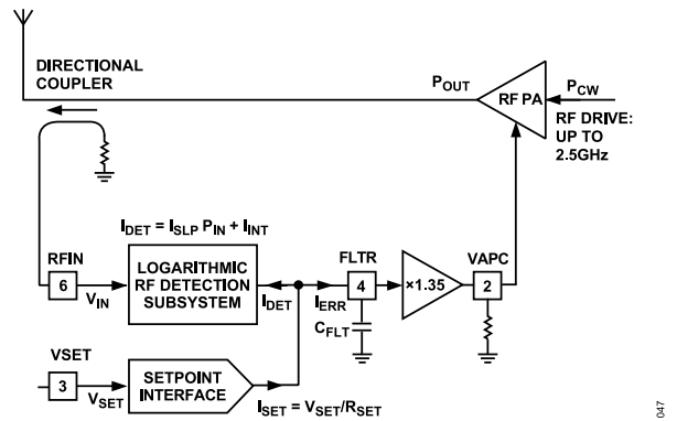
Figure 27. Behavioral Model of the AD8311
