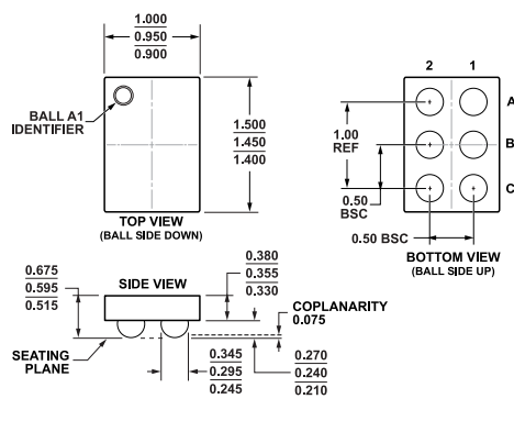
Figure 46. 6-Ball Wafer Level Chip Scale Package [WLCSP] (CB-6-2) Dimensions shown in millimeters
