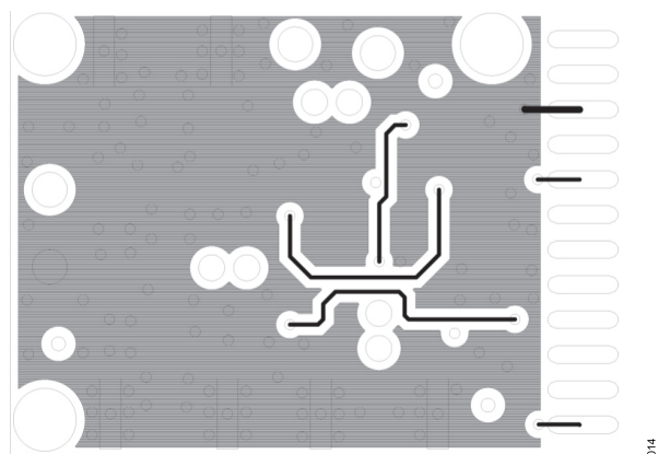
Figure 43. Layout of Circuit Side (WLCSP)
