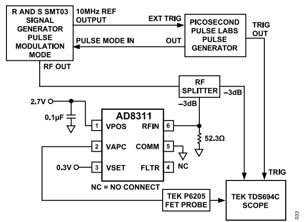
Figure 19. Test Setup for V_{APC} Response Time
