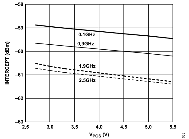
Figure 24. Intercept vs. Supply Voltage
