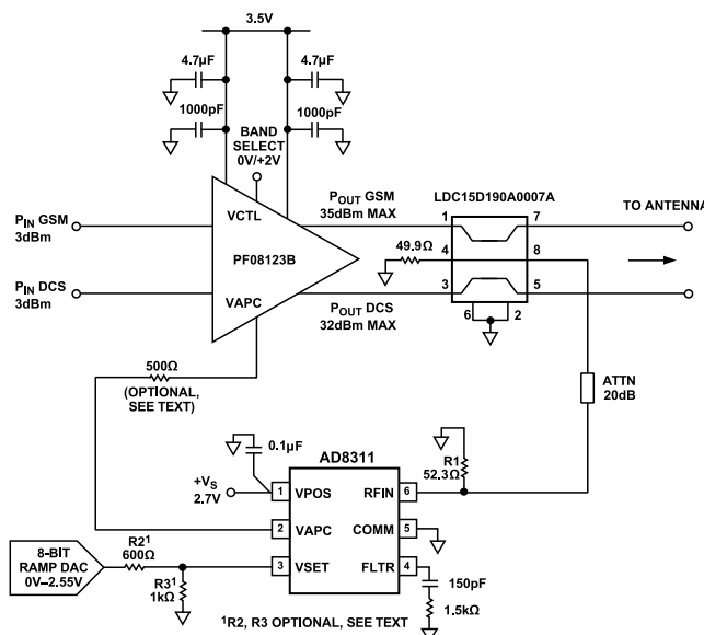
Figure 31. Dual Mode (GSM/DCS) PA Control Example
