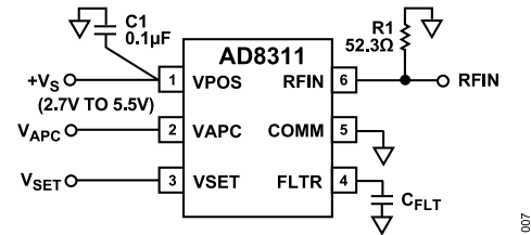
Figure 29. Basic Connections
