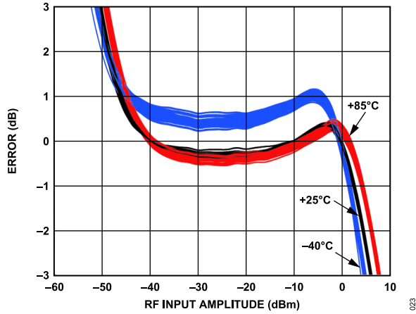
Figure 9. Distribution of Error over Temperature After Ambient Normalization vs. Input Amplitude at 0.1 GHz
