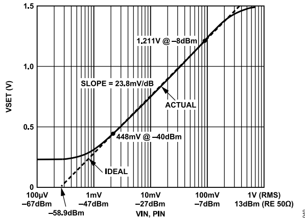
Figure 26. Basic Calibration of the AD8311 at 0.1 GHz
