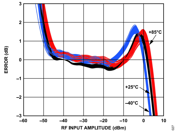
Figure 13. Distribution of Error over Temperature after Ambient Normalization vs. Input Amplitude at 2.5 GHz
