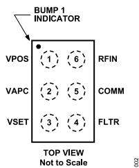
Figure 2. Pin Configuration
