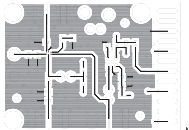
Figure 42. Layout of Component Side (WLCSP)
