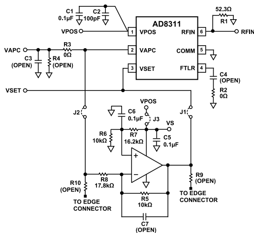
Figure 41. Evaluation Board Schematic
