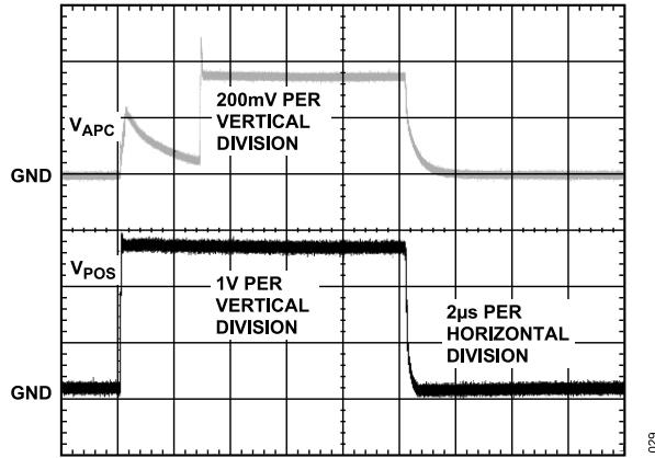
Figure 15. Power-On and -Off Response with VSET Grounded
