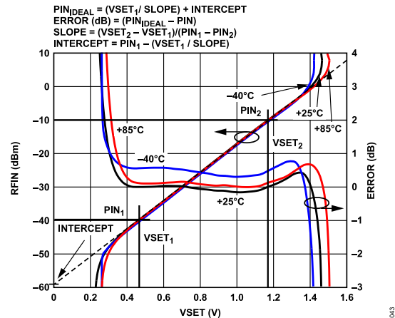
Figure 37. Transfer Function of AD8311 at 0.9 GHz
