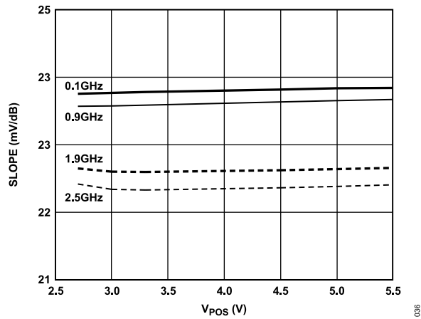
Figure 22. Slope vs. Supply Voltage
