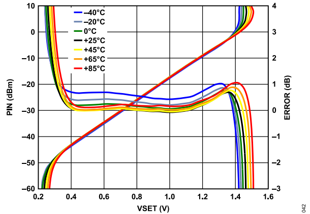
Figure 36. Typical Drift at 900 GHz for Various Temperatures
