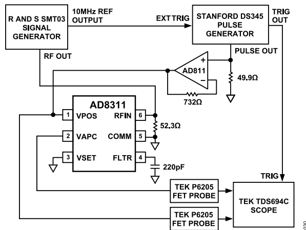
Figure 16. Test Setup for Power-On and -Off Response with VSET Grounded
