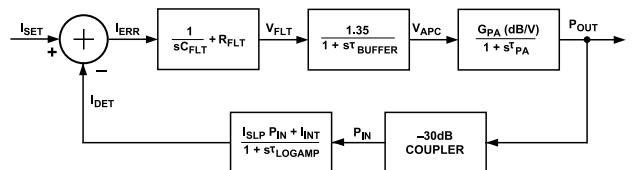
Figure 28. Control Loop Block Diagram
