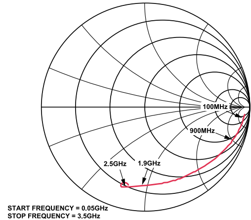
Figure 14. Input Impedance vs. Frequency, No Termination Resistor on RFIN
