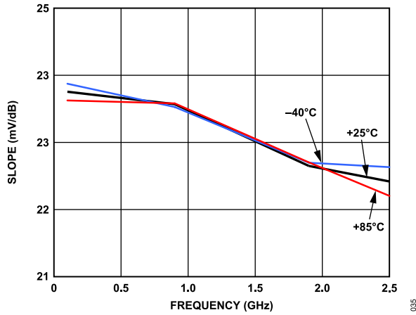
Figure 21. Slope vs. Frequency -40°C, +25°C, and +85°C
