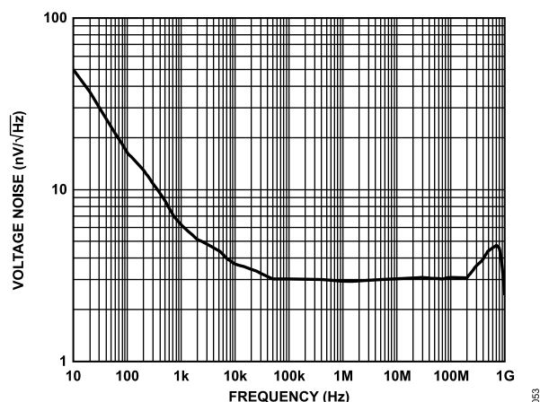
Figure 44. Voltage Noise vs. Frequency
