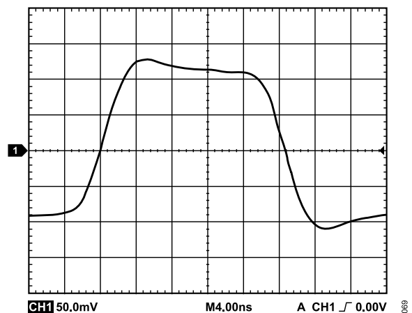
Figure 71. Small Signal Transient Response of 90 MHz LPF
