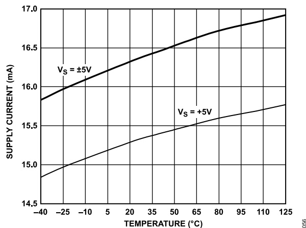
Figure 57. Supply Current vs. Temperature for Various Supplies
