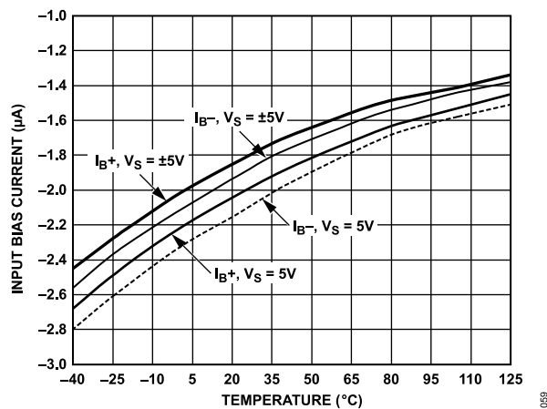
Figure 55. Input Bias Current vs. Temperature for Various Supplies
