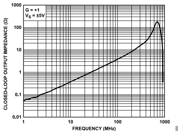
Figure 49. Output Impedance vs. Frequency
