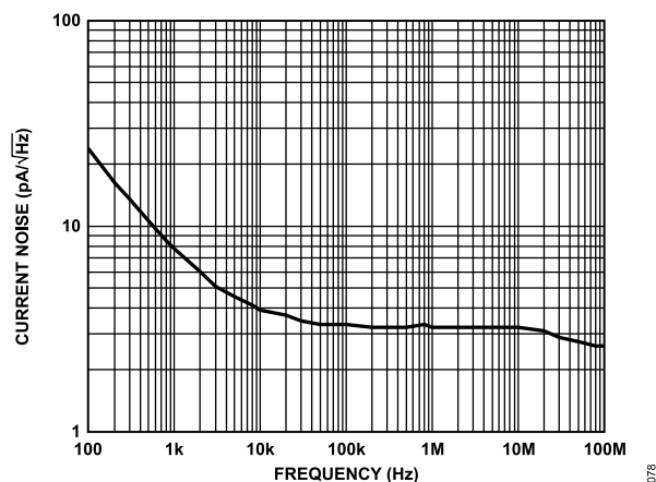
Figure 45. Current Noise vs. Frequency
