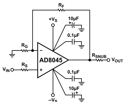
Figure 61. Noninverting Configuration
