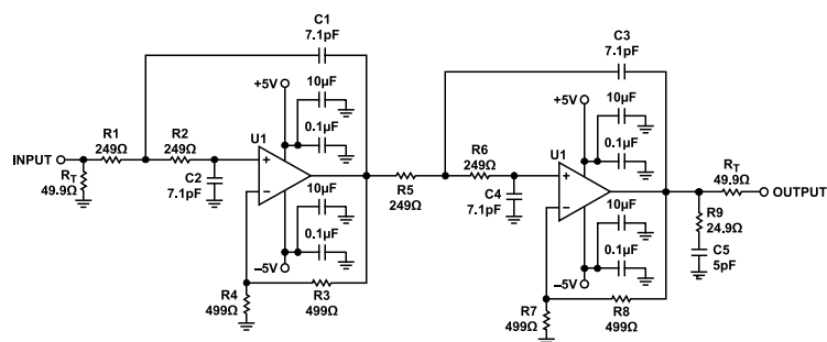
Figure 73. 4-Pole, 90 MHz, Sallen-Key Low-Pass Filter
