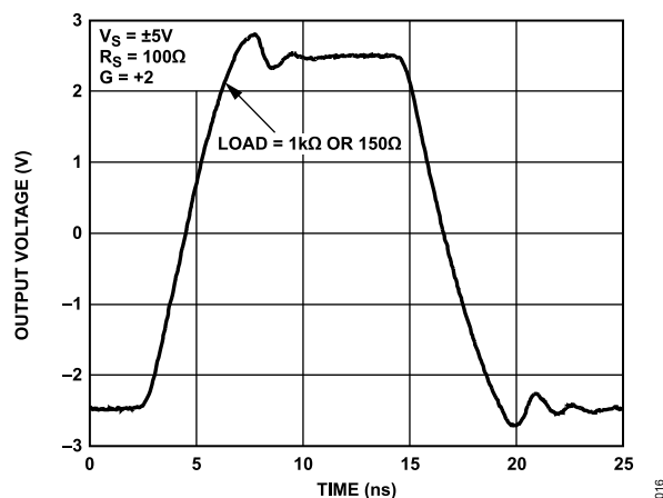
Figure 38. Large Signal Transient Response for Various Loads
