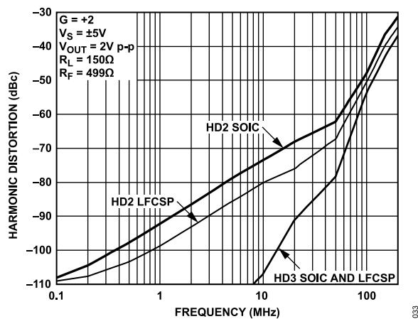
Figure 22. Harmonic Distortion vs. Frequency for Various Packages
