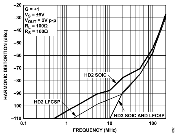
Figure 19. Harmonic Distortion vs. Frequency for Various Packages
