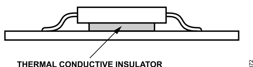
Figure 76. SOIC with Thermal Conductive Pad Material
