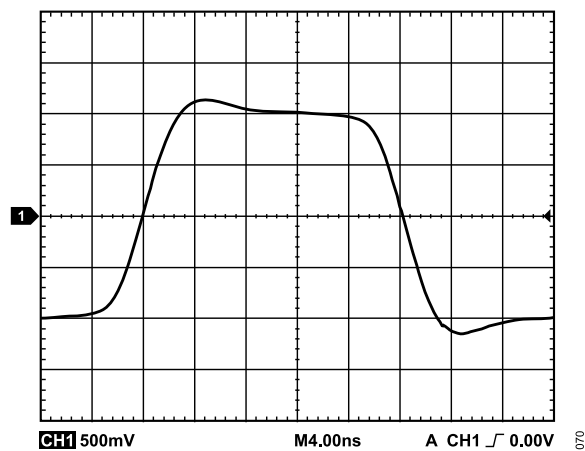
Figure 72. Large Signal Transient Response of 90 MHz LPF
