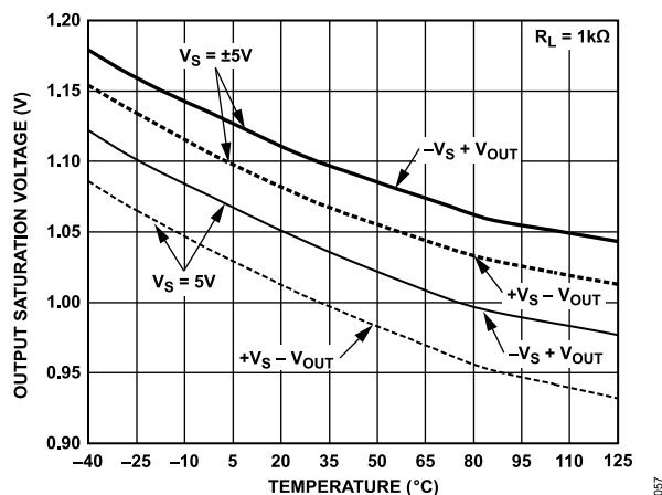
Figure 56. Output Saturation Voltage vs. Temperature for Various Supplies
