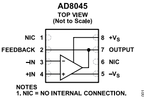
Figure 2. 8-Lead AD8045 LFCSP (CP-8)
