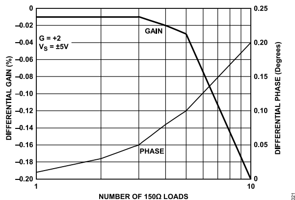
Figure 51. Differential Gain and Phase vs. Number of 150 \Omega Loads
