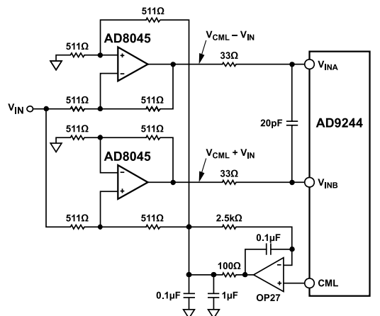
Figure 67. High Speed ADC Driver
