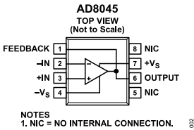
Figure 3. 8-Lead AD8045 SOIC/EP (RD-8)
