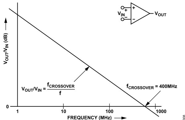
Figure 63. Open-Loop Response
