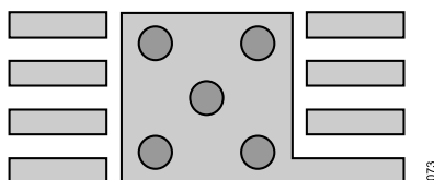
Figure 75. LFCSP Exposed Paddle Layout
