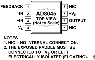
Figure 5. 8-Lead SOIC Pin Configuration
