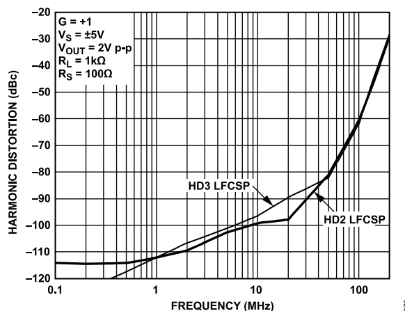
Figure 1. Harmonic Distortion vs. Frequency for Various Packages
