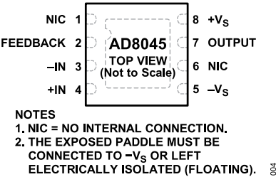
Figure 6. 8-Lead LFCSP Pin Configuration
