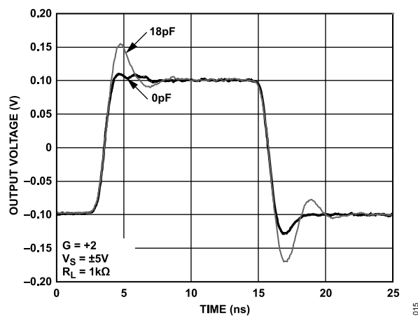
Figure 37. Small Signal Transient Response with Capacitive Load
