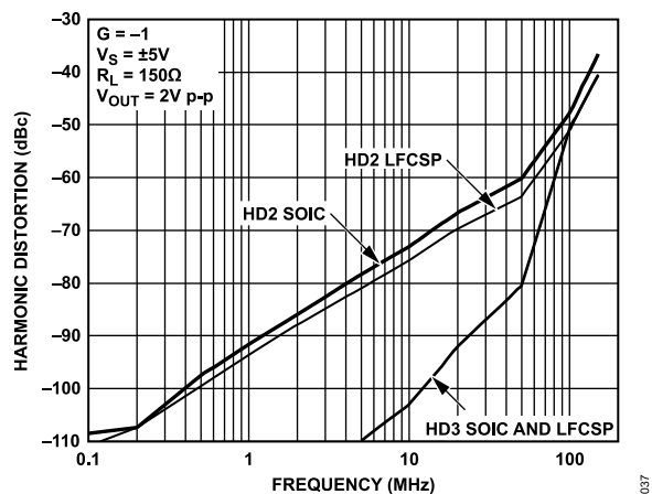
Figure 21. Harmonic Distortion vs. Frequency for Various Packages
