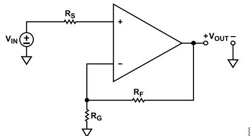
Figure 64. Noninverting Configuration
