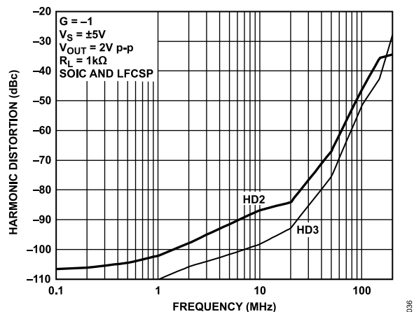
Figure 20. Harmonic Distortion vs. Frequency for Various Packages
