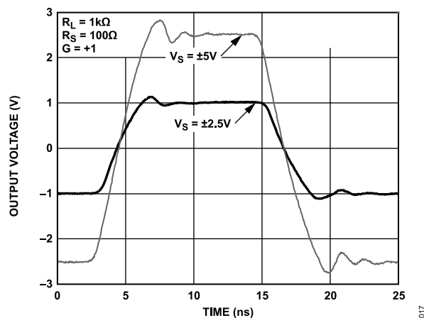
Figure 39. Large Signal Transient Response for Various Supplies
