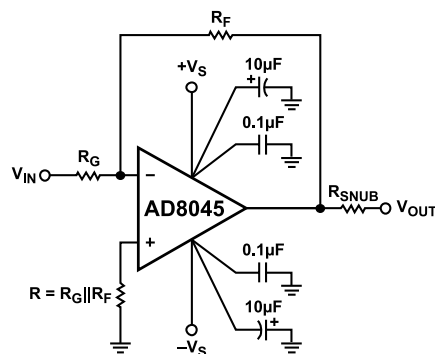
Figure 62. Inverting Configuration
