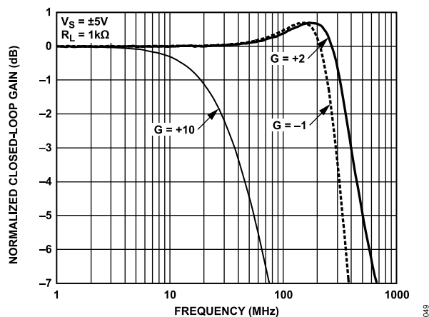
Figure 7. Small Signal Frequency Response for Various Gains
