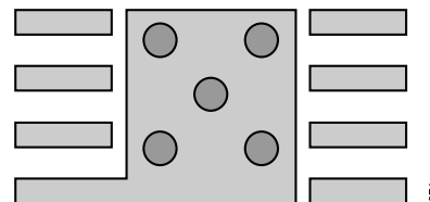
Figure 74. SOIC Exposed Paddle Layout
