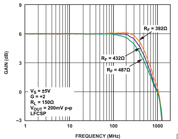
Figure 8. Small Signal Frequency Response vs. R_F
