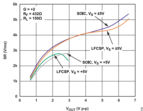
Figure 37. Slew Rate vs. Output Level
