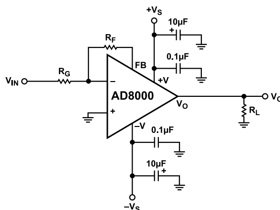
Figure 51. Inverting Configuration
