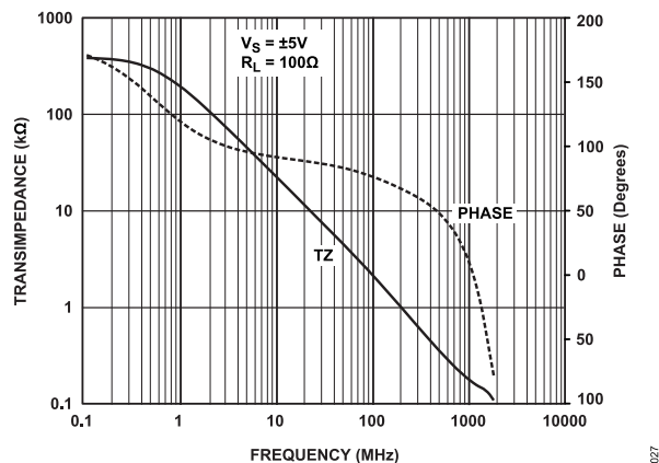
Figure 10. Transimpedance and Phase vs. Frequency
