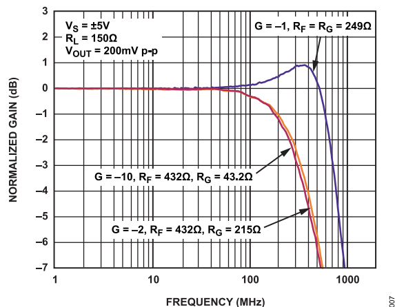
Figure 6. Small Signal Frequency Response vs. Various Gains
