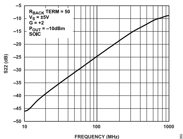
Figure 45. Output Voltage Standing Wave Ratio (S22)
