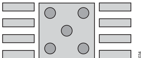
Figure 53. LFCSP Exposed Paddle Layout
