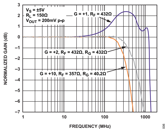
Figure 5. Small Signal Frequency Response vs. Various Gains
