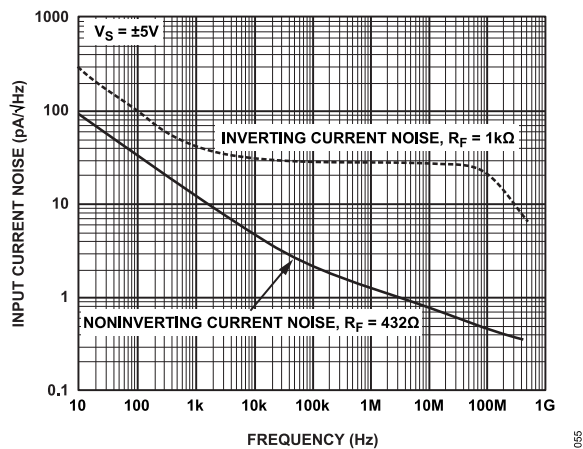
Figure 41. Input Current Noise
