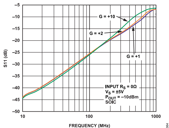
Figure 46. Input Voltage Standing Wave Ratio (S11)
