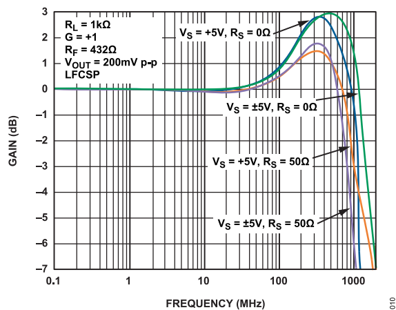
Figure 11. Small Signal Frequency Response vs. Supply Voltage
