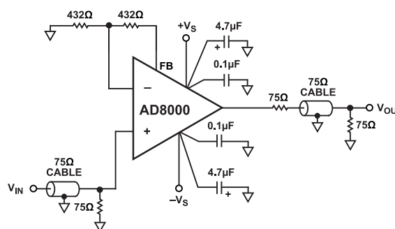
Figure 52. Video Line Driver
