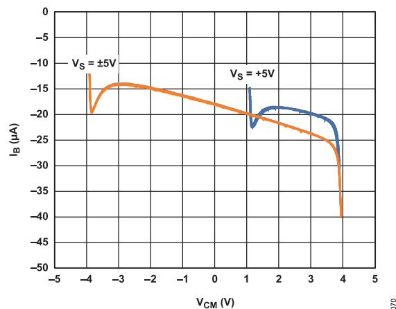
Figure 44. Input Bias Current vs. Common-Mode Voltage
