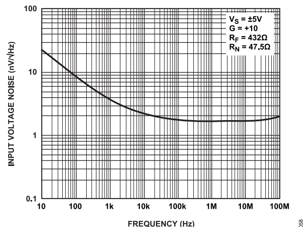
Figure 40. Input Voltage Noise
