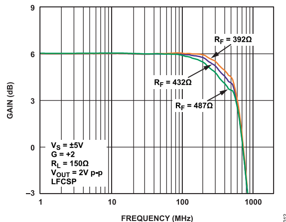
Figure 9. Large Signal Frequency Response vs. R_F
