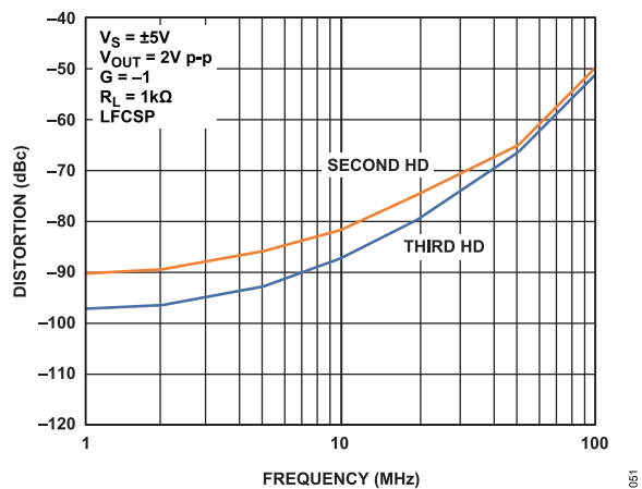
Figure 29. Harmonic Distortion vs. Frequency
