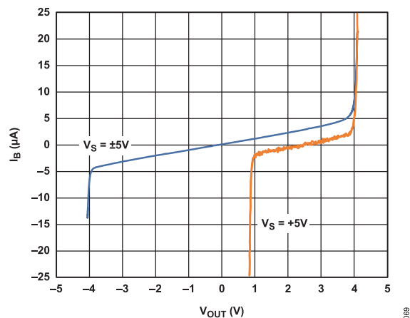
Figure 43. Input Bias Current vs. Output Voltage
