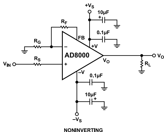
Figure 50. Noninverting Configuration
