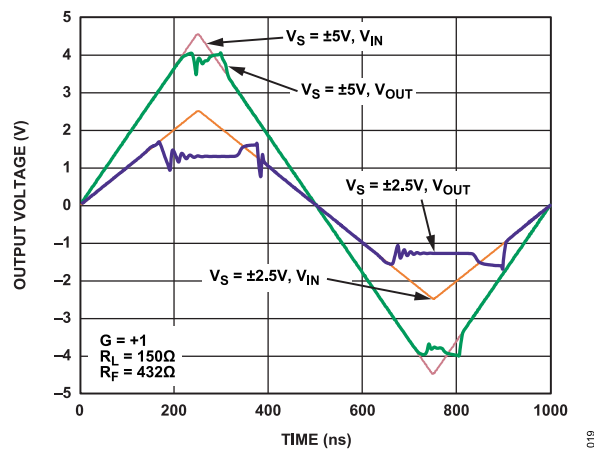
Figure 38. Input Overdrive
