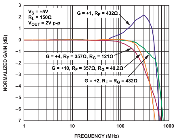
Figure 7. Large Signal Frequency Response vs. Various Gains
