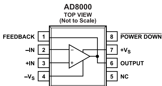
Figure 2. 8-Lead AD8000, 3 mm × 3 mm LFCSP (CP-8-13)
