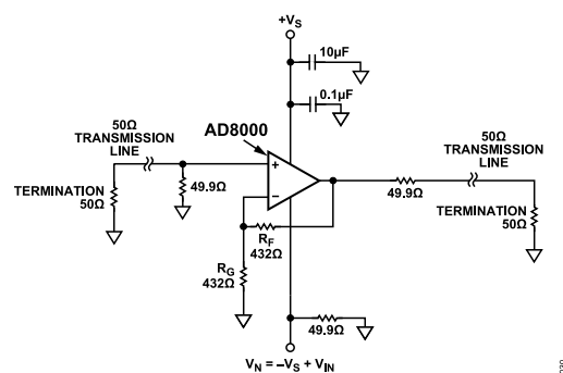
Figure 49. Negative PSRR
