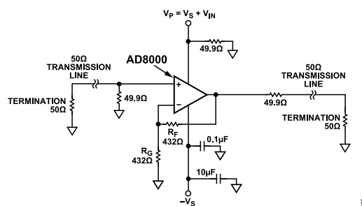
Figure 48. Positive PSRR
