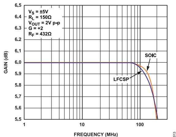
Figure 13. 0.1 dB Flatness
