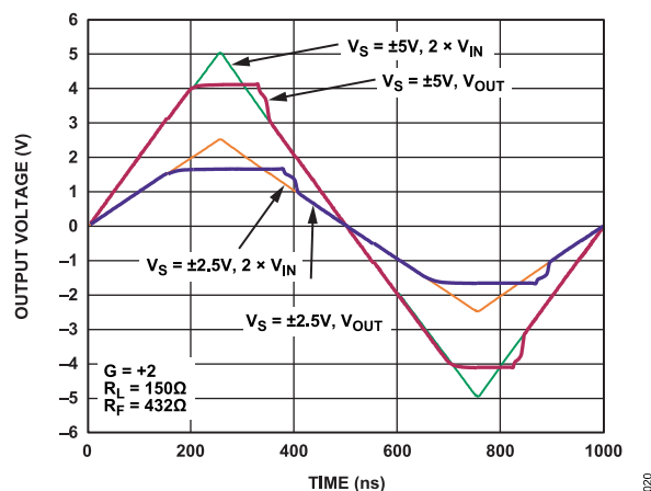
Figure 39. Output Overdrive
