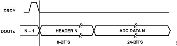
Figure 108. ADC Output—8-Bit Header + 24-Bit Conversion Data
