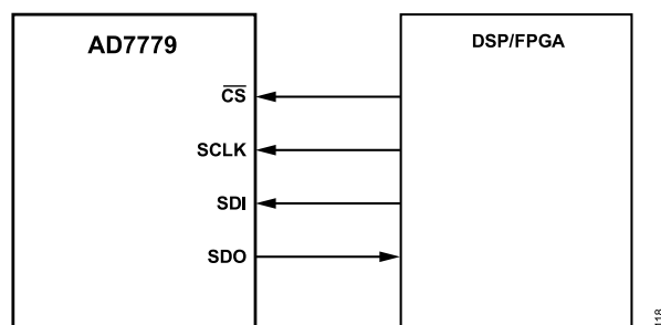
Figure 101. SPI Control Interface—AD7779 is the SPI Subordinate, Digital Signal Processor (DSP)/Field Programmable Gate Array (FPGA) is the Main
