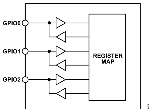
Figure 100. GPIO Pin Functionality
