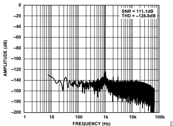
Figure 19. FFT, Median Mode, Sinc5 Filter, -0.5 dBFS
