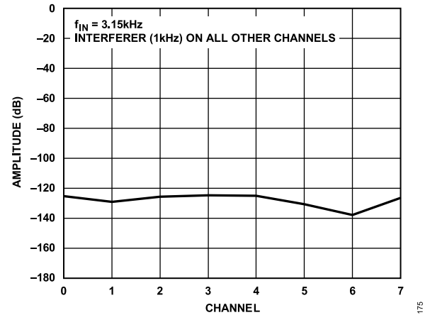
Figure 33. Crosstalk
