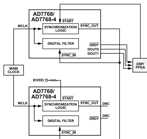
Figure 110. Synchronizing Multiple AD7768/AD7768-4 Devices Using SYNC OUT
