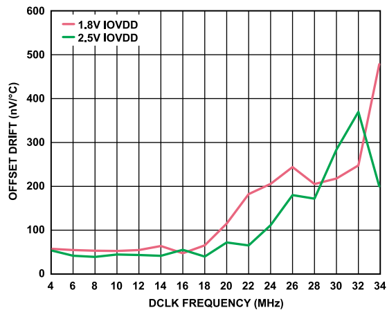
Figure 49. Offset Drift vs. DCLK Frequency
