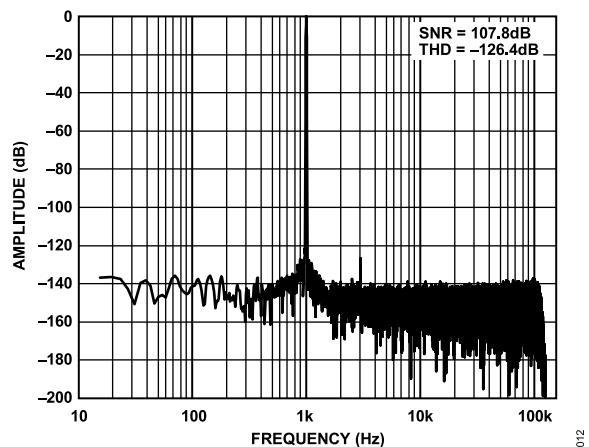
Figure 12. Fast Fourier Transform (FFT), Fast Mode, Wideband Filter, -0.5 dBFS
