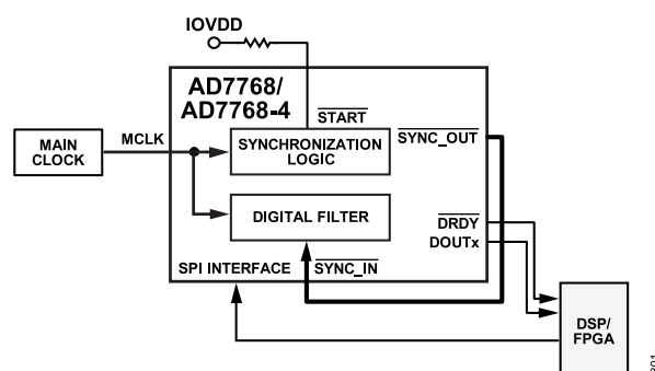
Figure 81. Connection Diagram for Synchronization Using SPI SYNC
