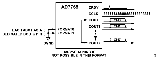
Figure 95. AD7768 FORMATx = 00, Eight Data Output Pins
