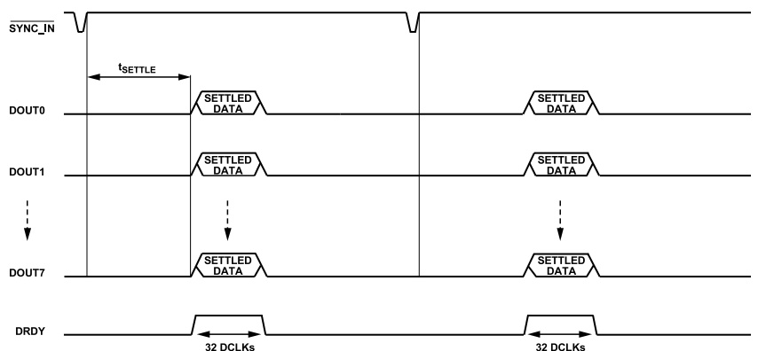
Figure 108. AD7768 One Shot Mode
