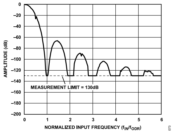
Figure 60. Amplitude vs. Normalized Input Frequency ( f_{IN}/f_{ODR} ), Sinc5 Filter Profile
