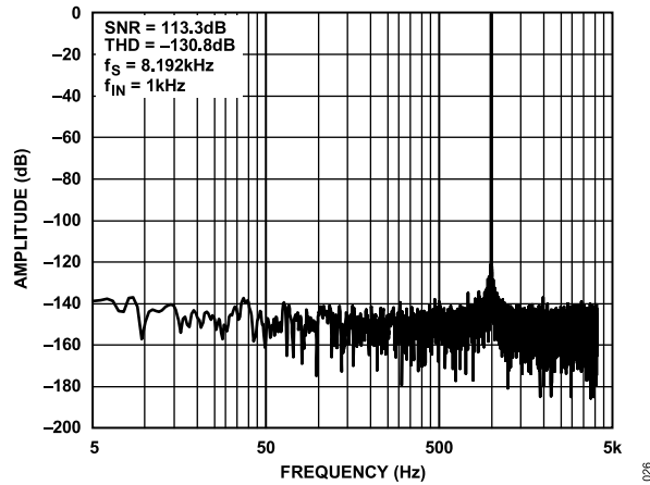
Figure 24. FFT One Shot Mode, Sinc5 Filter, Median Mode, Decimation = \times 64 , -0.5 dBFS, \text{SYNC\_IN} Frequency = \text{MCLK}/4000
