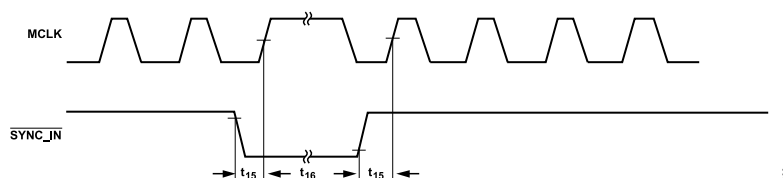
Figure 6. Synchronous SYNC_IN Pulse Timing Diagram
