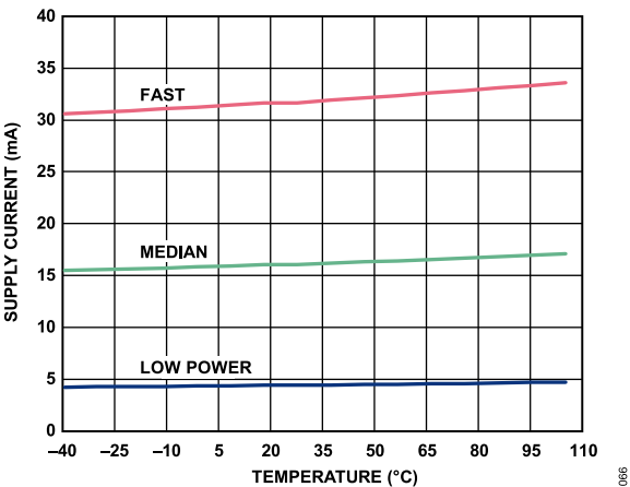
Figure 65. Supply Current vs. Temperature, AVDD1
