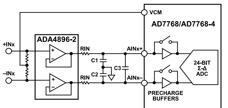
Figure 87. Typical Input Structure for an RC Network
