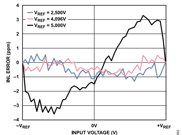
Figure 40. INL Error vs. Input Voltage for Various V_{REF} Levels, Fast Mode
