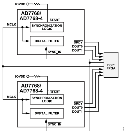
Figure 111. Synchronizing Multiple AD7768/AD7768-4 Devices Using Only SYNC_IN
