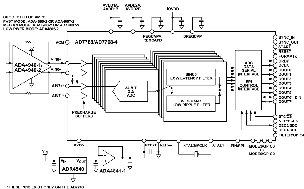
Figure 73. Typical Connection Diagram
