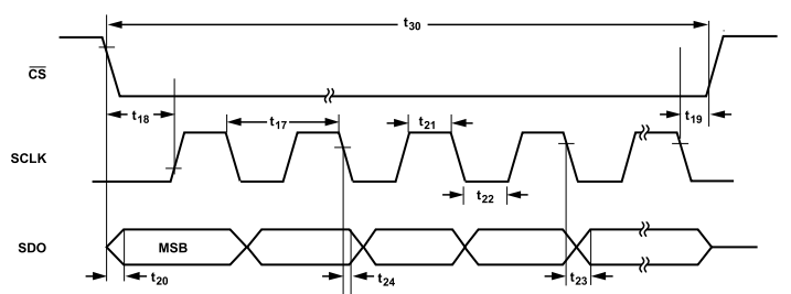
Figure 7. SPI Serial Read Timing Diagram
