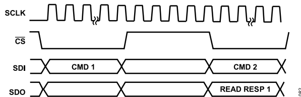
Figure 79. Off Frame Protocol
