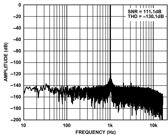
Figure 20. FFT, Low Power Mode, Sinc5 Filter, -0.5 dBFS
