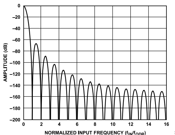
Figure 89. Sinc5 Filter Frequency Response (Decimation = \times 32 )
