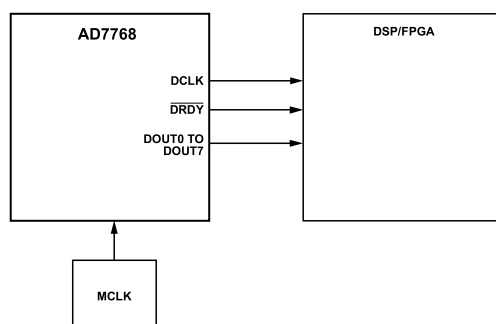
Figure 107. Data Interface: Standard Conversion Operation, AD7768 = Main, DSP/FPGA = Subordinate
