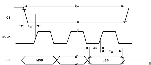
Figure 8. SPI Serial Write Timing Diagram
