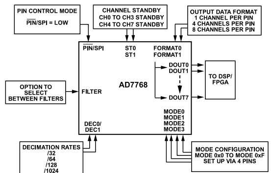
Figure 76. AD7768 Pin Configurable Functions
