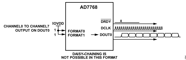
Figure 98. AD7768 FORMATx = 10 or 11, or AD7768-4 FORMAT0 = 1, One Data Output Pin
