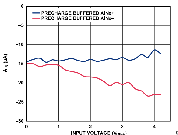
Figure 86. Analog Input Current ( I_{AIN} ) vs. Input Voltage, Analog Input Precharge Buffer On, V_{CM} = 2.5 V, f_{MOD} = 8.192 MHz
