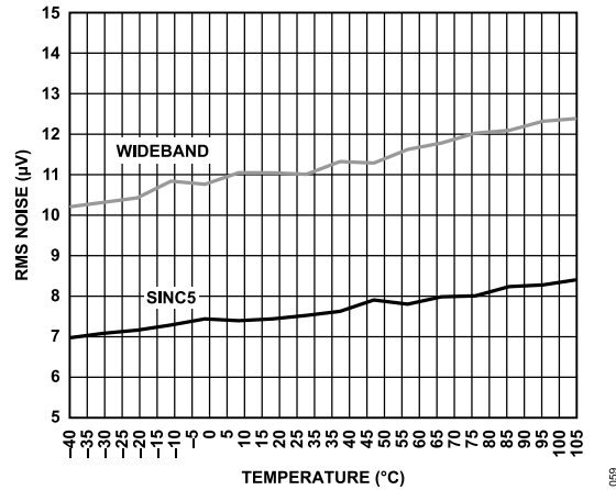
Figure 30. RMS Noise vs. Temperature, Median Mode
