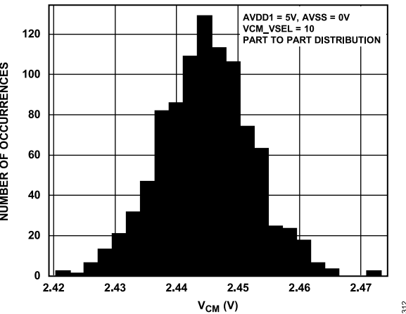
Figure 64. VCM Output Voltage Distribution
