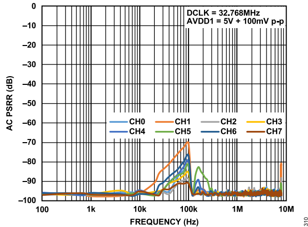
Figure 54. AC PSRR vs. Frequency, AVDD1
