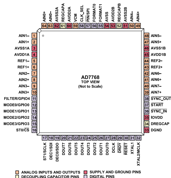
Figure 10. AD7768 Pin Configuration
