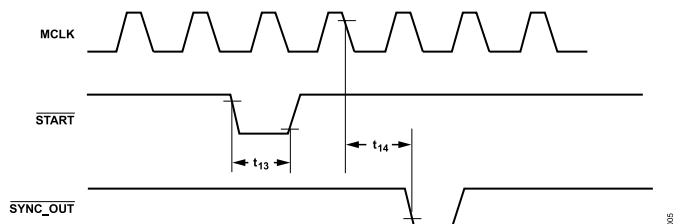
Figure 5. Asynchronous START and SYNC_OUT Timing Diagram
