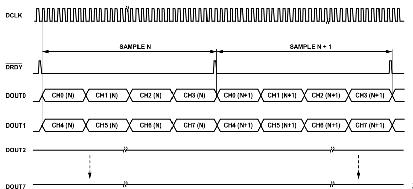
Figure 101. AD7768 FORMATx = 01: Channel 0 to Channel 3 Share DOUT0, and Channel 4 to Channel 7 Share DOUT1, Maximum Data Rate
