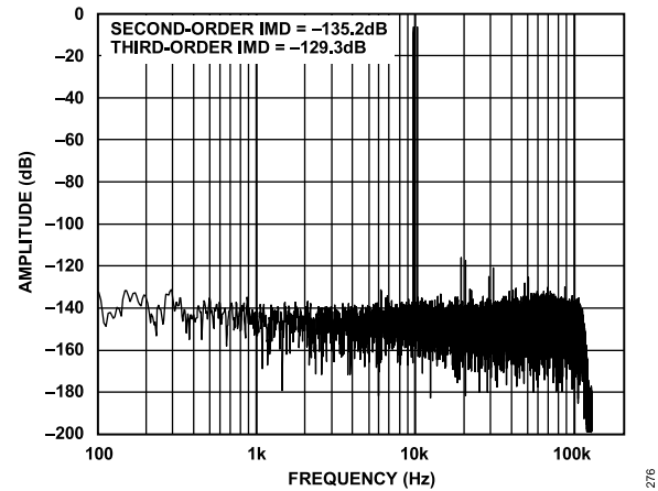
Figure 25. Intermodulation Distortion (IMD) with Input Signals at 9.7 kHz and 10.3 kHz
