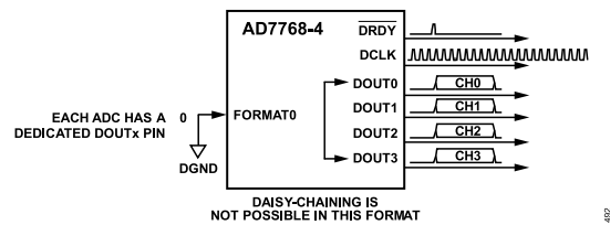
Figure 97. AD7768-4 FORMAT0 = 0, Four Data Output Pins
