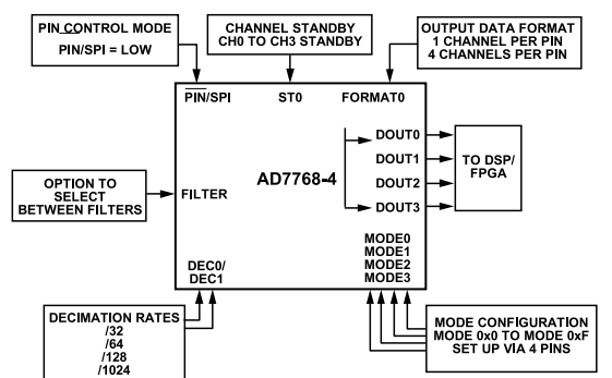
Figure 77. AD7768-4 Pin Configurable Functions
