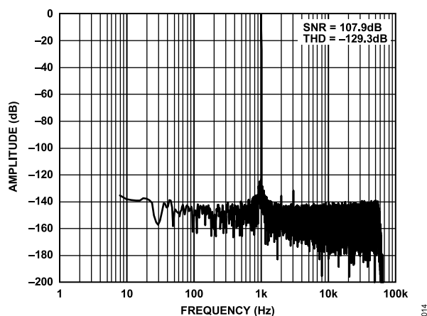
Figure 13. FFT, Median Mode, Wideband Filter, -0.5 dBFS
