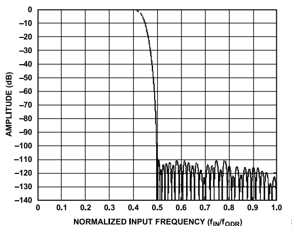
Figure 90. Wideband Filter Frequency Response
