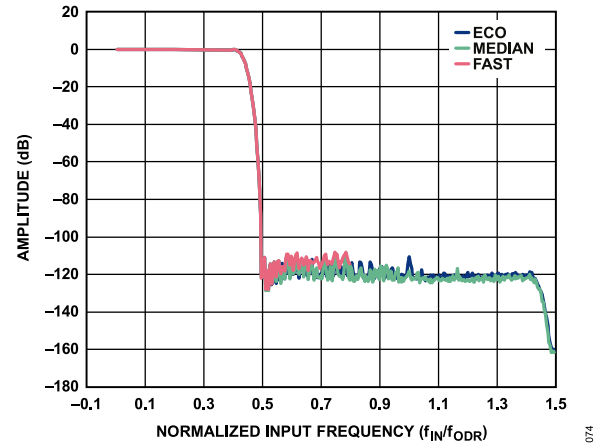
Figure 57. Amplitude vs. Normalized Input Frequency ( f_{IN}/f_{ODR} ), Wideband Filter Profile
