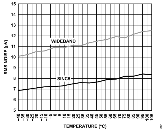
Figure 31. RMS Noise vs. Temperature, Low Power Mode
