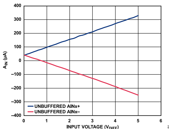
Figure 85. Analog Input Current ( I_{AIN} ) vs. Input Voltage, Analog Input Precharge Buffer Off, V_{CM} = 2.5 V, f_{MOD} = 8.192 MHz
