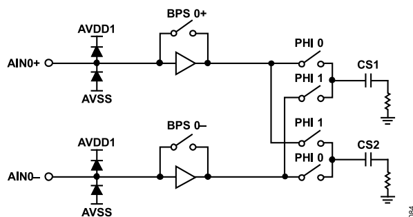
Figure 84. Analog Front End
