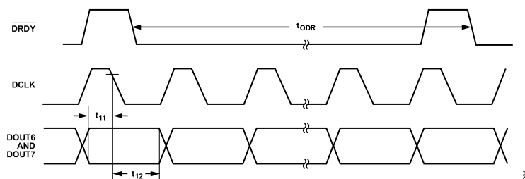
Figure 4. Daisy-Chain Setup and Hold Timing Diagram
