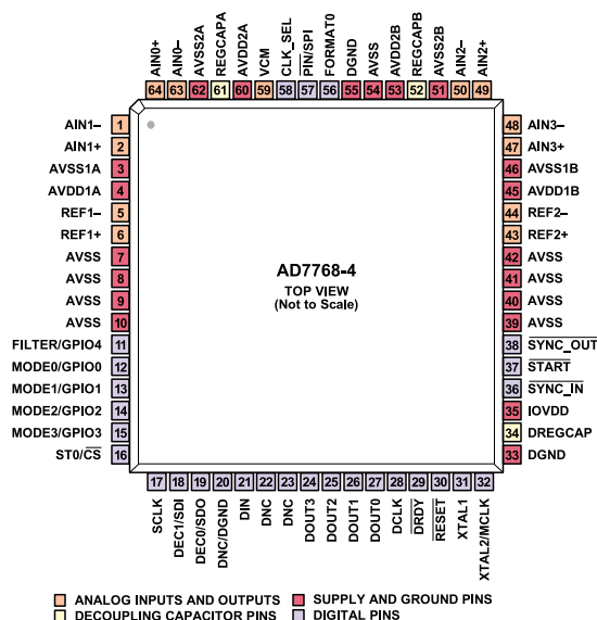
Figure 11. AD7768-4 Pin Configuration
