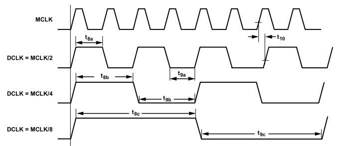
Figure 3. MCLK to DCLK Divider Timing Diagram
