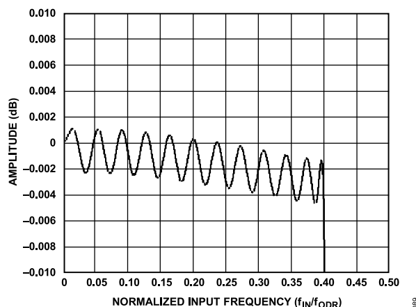
Figure 91. Wideband Filter Pass-Band Ripple
