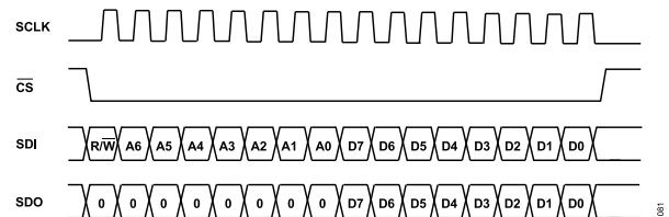
Figure 80. Write/Read Command
