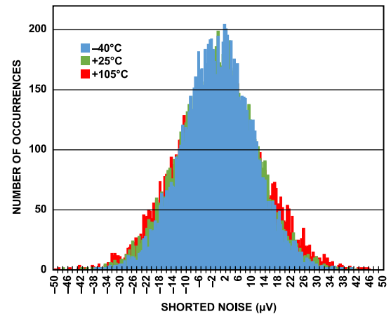
Figure 28. Shorted Noise at Different Temperatures, Wideband Filter
