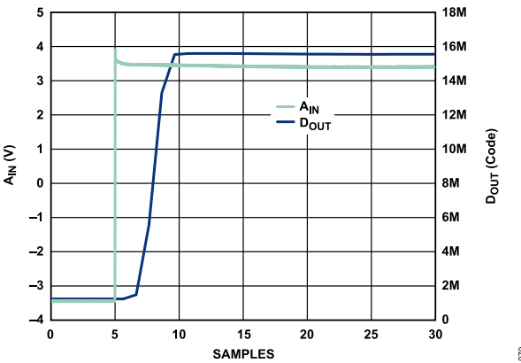
Figure 61. Step Response, Sinc5 Filter
