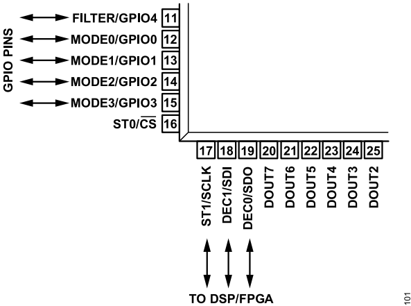
Figure 113. AD7768 GPIO Functionality
