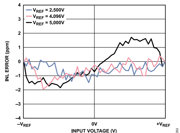
Figure 41. INL Error vs. Input Voltage for Various V_{REF} Levels, Median Mode
