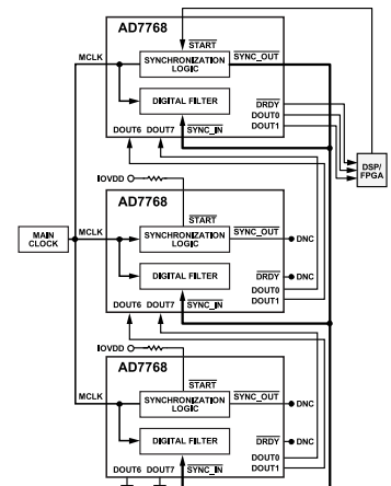
Figure 109. Daisy-Chaining Multiple AD7768 Devices
