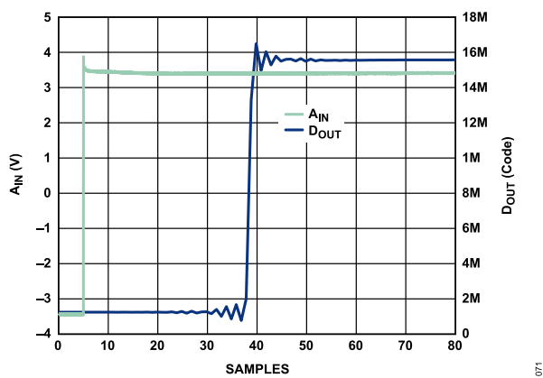
Figure 58. Step Response, Wideband Filter
