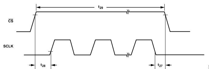
Figure 9. SCLK Enable and Disable Timing Diagram
