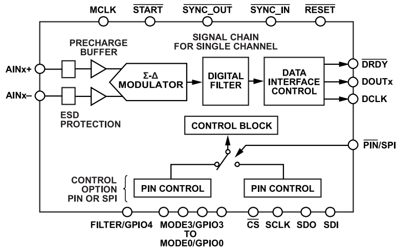
Figure 83. Top Level Core Signal Chain and Control
