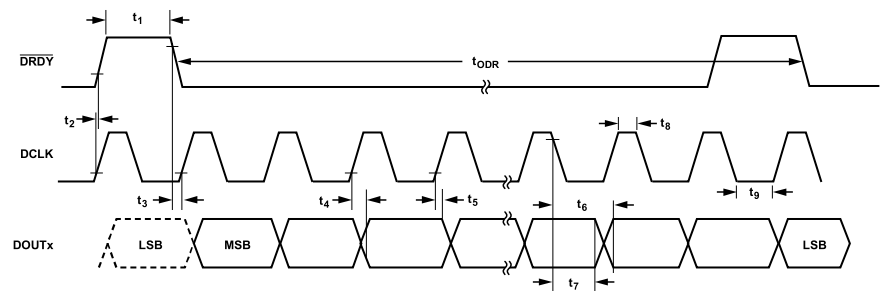
Figure 2. Data Interface Timing Diagram
