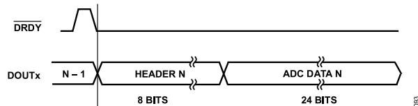
Figure 99. ADC Output: 8-Bit Header, 24-Bit ADC Conversion Data
