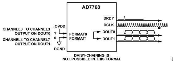
Figure 96. AD7768 FORMATx = 01, Two Data Output Pins
