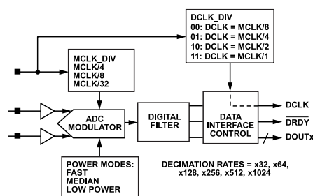
Figure 72. Sampling Structure, Defined by MCLK, DCLK_DIV, and MCLK_DIV Settings
