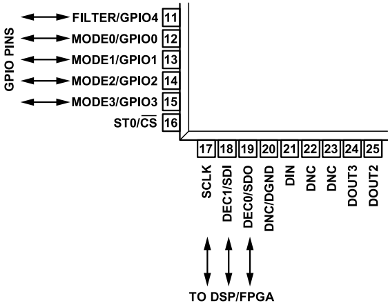
Figure 114. AD7768-4 GPIO Functionality
