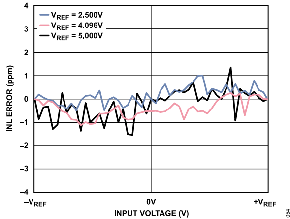
Figure 42. INL Error vs. Input Voltage for Various V_{REF} Levels, Low Power Mode
