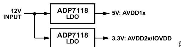
Figure 74. Power Supply Configuration
