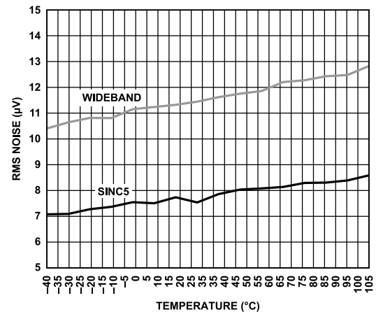
Figure 29. RMS Noise vs. Temperature, Fast Mode
