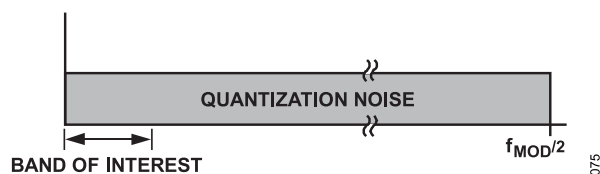
Figure 69. \Sigma - \Delta ADC Quantization Noise (Linear Scale X-Axis)
