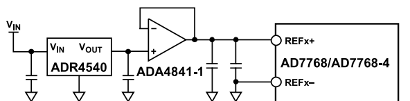
Figure 88. Typical Reference Input Configuration Diagram
