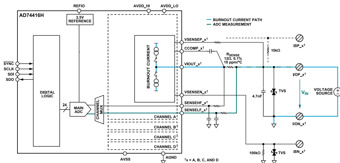
Figure 39. Voltage Input Mode Configuration
