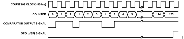
Figure 45. Digital Input Debounce Mode 0 Timing Example
