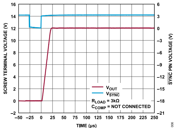
Figure 6. Full-Scale Positive Step without C_{COMP}
