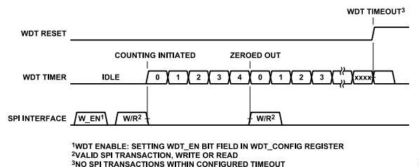
Figure 61. Watchdog Timing Diagram
