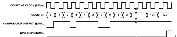
Figure 46. Digital Input Debounce Mode 1 Timing Example
