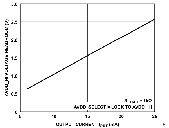
Figure 11. AVDD_{HI} Voltage Headroom vs. I_{OUT}
