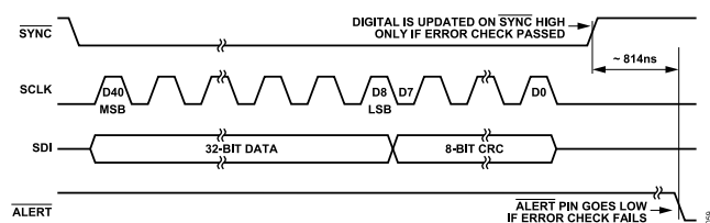
Figure 60. CRC Timing
