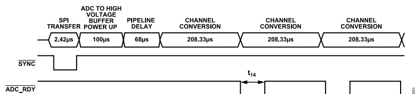
Figure 51. Single Measurement, Continuous Conversions Timing Diagram
