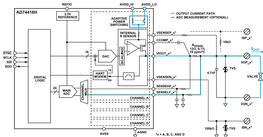
Figure 38. Current Output Mode Configuration
