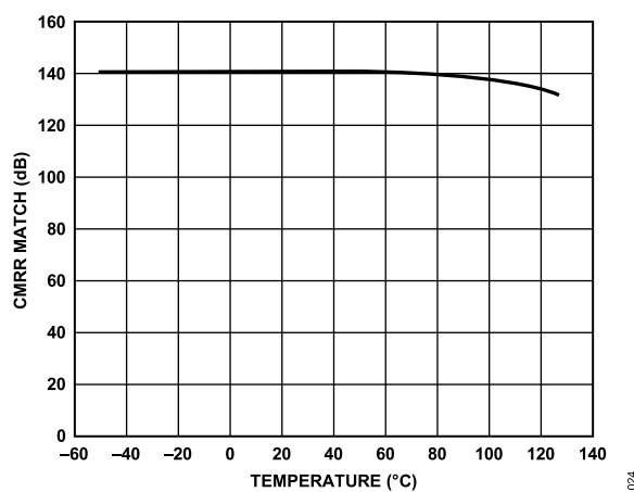
Figure 24. Common-Mode Rejection Ratio (CMRR) Match vs. Temperature
