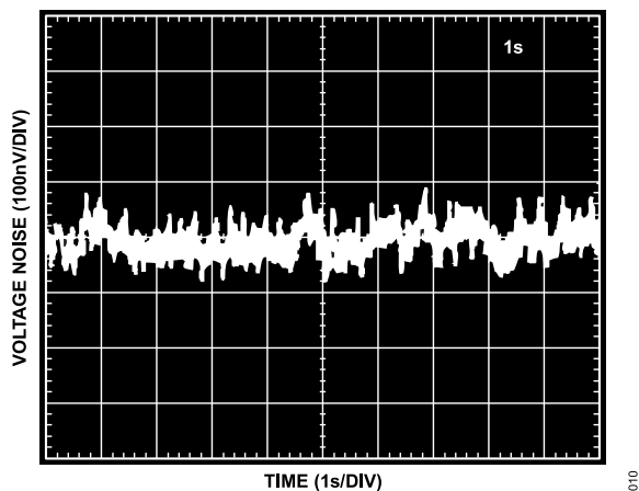
Figure 10. 0.1 Hz to 10 Hz Voltage Noise
