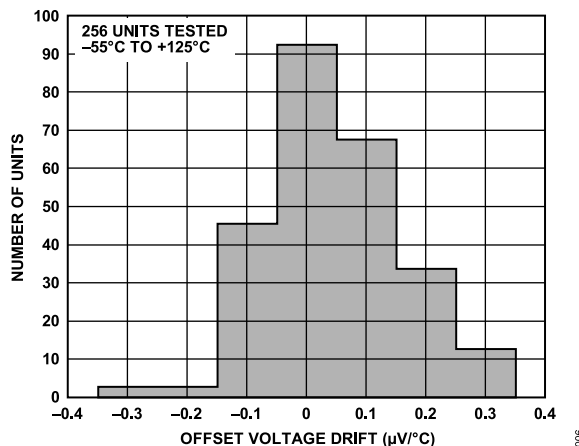
Figure 6. Typical Distribution of Offset Voltage Drift
