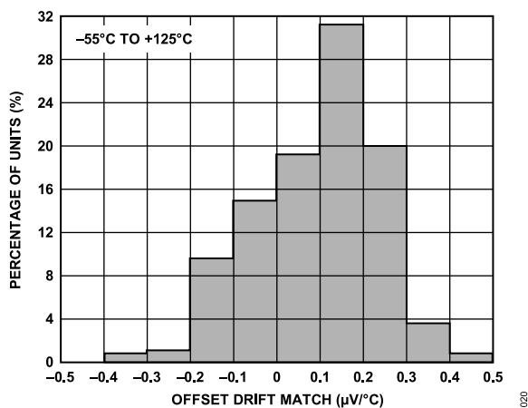
Figure 20. Typical Distribution of Offset Voltage Drift Match
