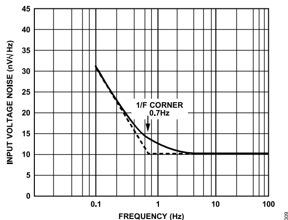
Figure 9. Input Noise Spectral Density
