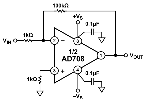
Figure 28. Gain of -100 Configuration
