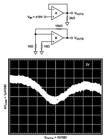
Figure 27. Crosstalk Under Forced Source and Sink Conditions
