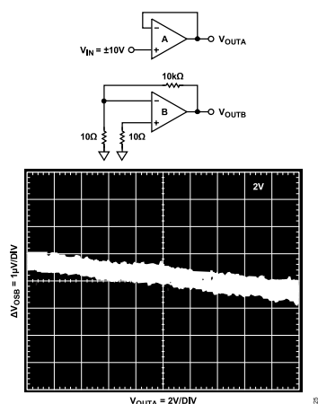
Figure 25. Crosstalk with No Load
