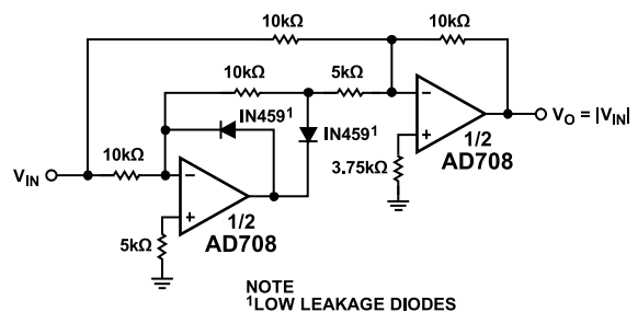
Figure 31. Precision Absolute Value Circuit
