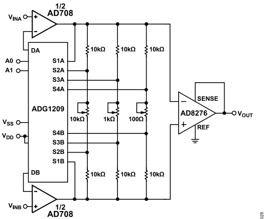
Figure 29. Precision PGA
