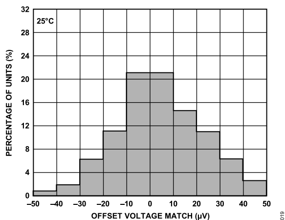
Figure 19. Typical Distribution of Offset Voltage Match
