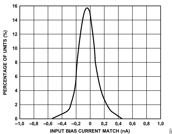
Figure 21. Typical Distribution of Input Bias Current Match
