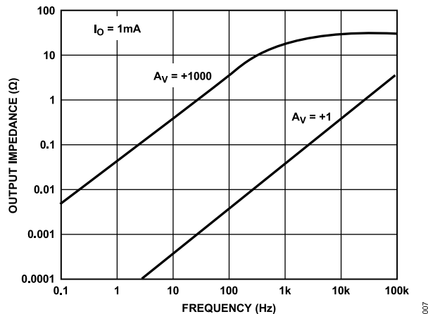
Figure 7. Output Impedance vs. Frequency
