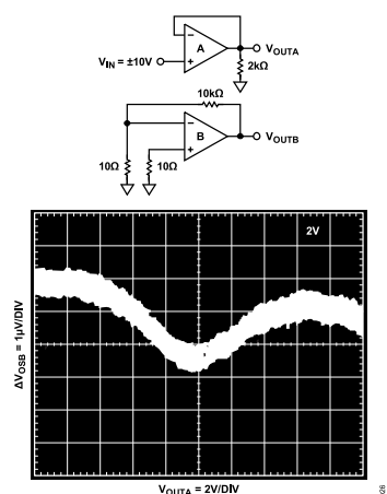
Figure 26. Crosstalk with 2\text{ k}\Omega Load
