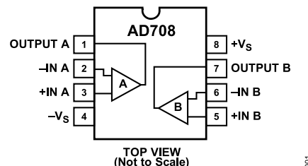
Figure 1. PDIP (N) and CERDIP (Q) Packages
