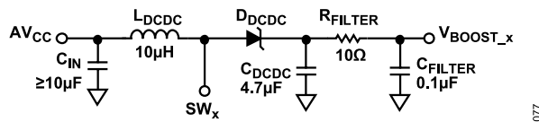
Figure 79. DC-to-DC Circuit
