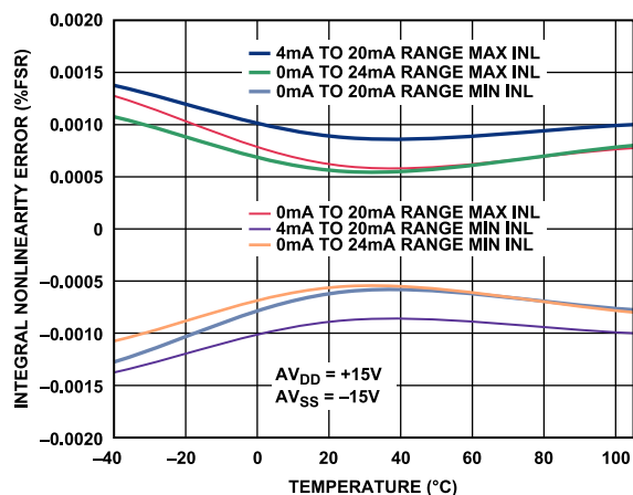
Figure 36. Integral Nonlinearity vs. Temperature, External R_{SET}
