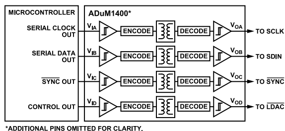
Figure 87. Isolated Interface
