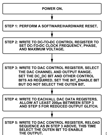
Figure 75. Programming Sequence for Enabling the Output Correctly
