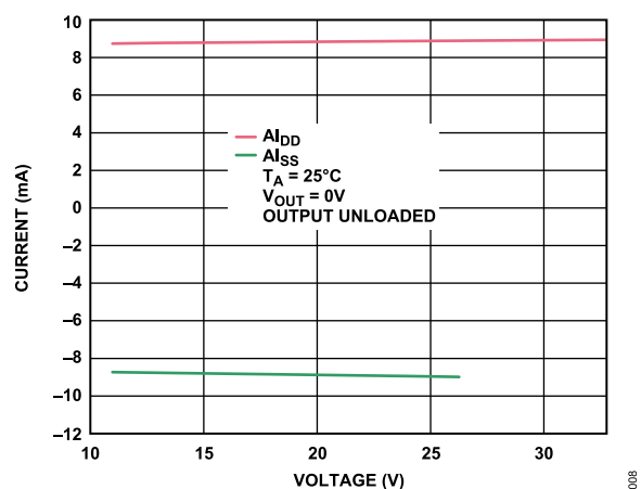
Figure 67. AL_{DD}/AL_{SS} vs. AV_{DD}/AV_{SS}
