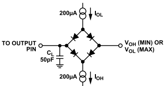
Figure 7. Load Circuit for SDO Timing Diagram
