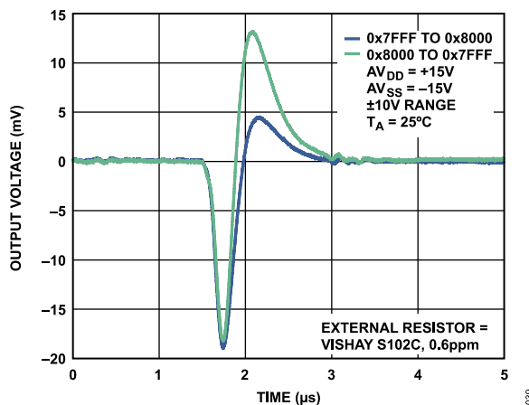
Figure 26. Digital-to-Analog Glitch
