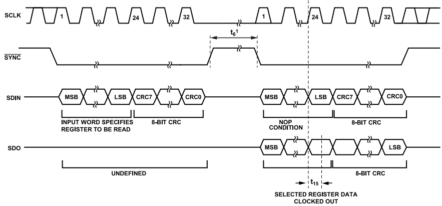
Figure 5. Readback Timing Diagram (Packet Error Checking Enabled)
