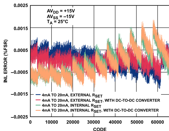
Figure 32. Integral Nonlinearity vs. Code
