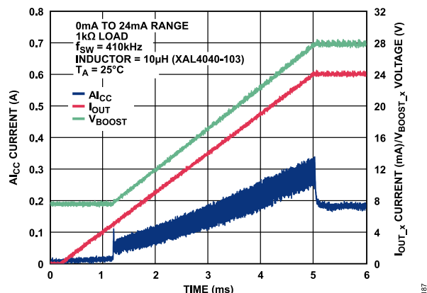
Figure 84. Al_{CC} Current vs. Time for 24 mA Step Through 1 kΩ Load with Slew Rate Control
