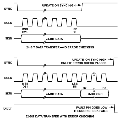
Figure 78. PEC Timing
