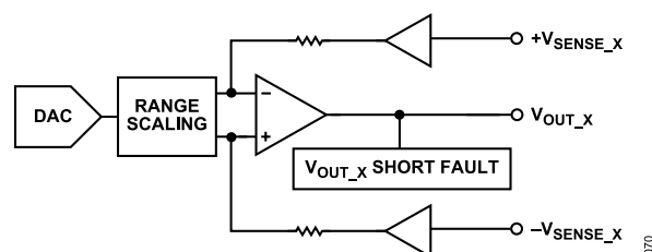
Figure 72. Voltage Output
