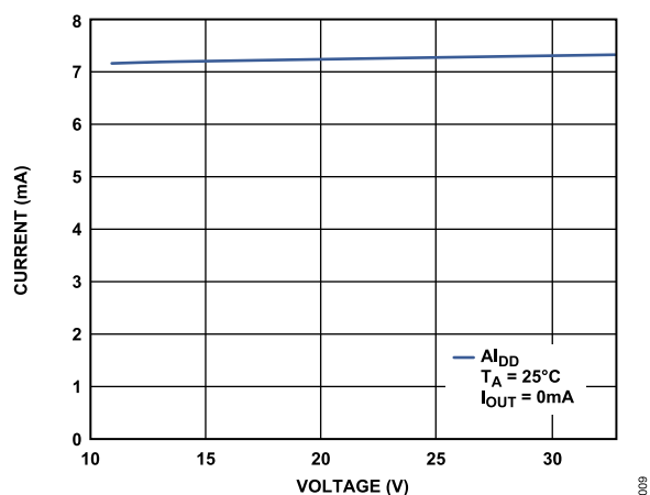
Figure 68. AL_{DD} vs. AV_{DD}
