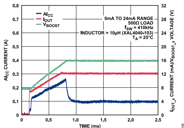
Figure 83. Al_{CC} Current vs. Time for 24 mA Step Through 500 Ω Load with External 51 kΩ Compensation Resistor
