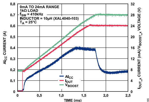
Figure 82. Al_{CC} Current vs. Time for 24 mA Step Through 1 kΩ Load with External 51 kΩ Compensation Resistor
