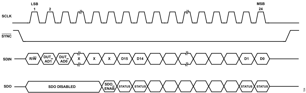
Figure 6. Status Readback During Write
