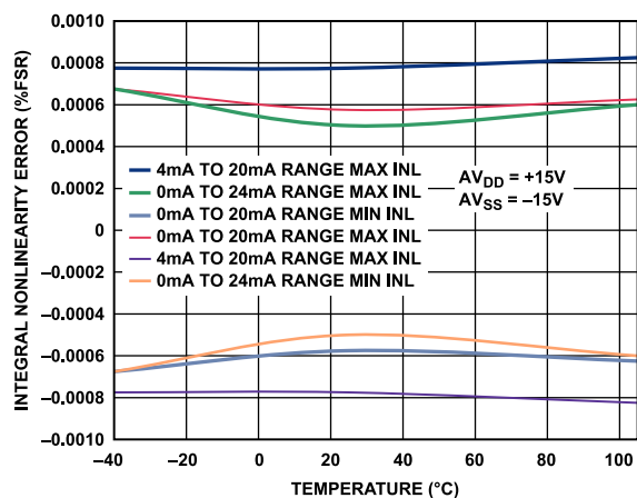
Figure 35. Integral Nonlinearity vs. Temperature, Internal R_{SET}
