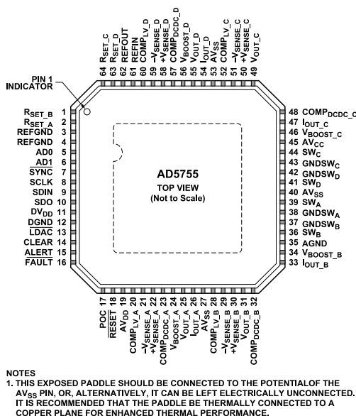
Figure 8. Pin Configuration
