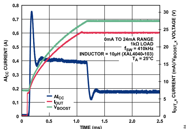
Figure 81. Al_{CC} Current vs. Time for 24 mA Step Through 1 kΩ Load with Internal Compensation Resistor
