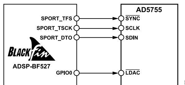
Figure 86. AD5755-to-ADSP-BF527 SPORT Interface
