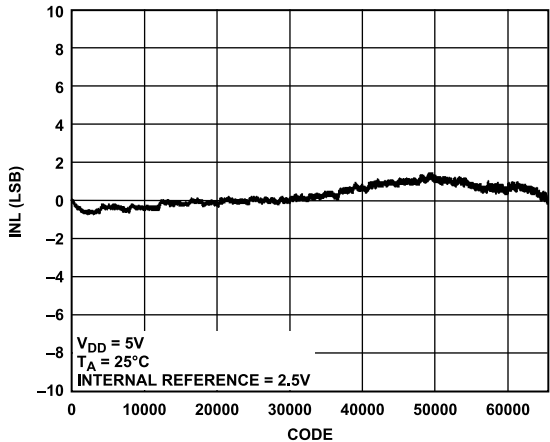
Figure 12. AD5696R INL
