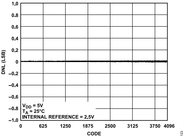
Figure 17. AD5694R DNL
