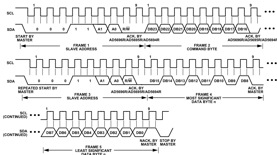
Figure 51. I²C Read Operation
