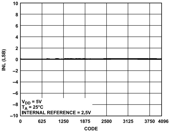
Figure 14. AD5694R INL
