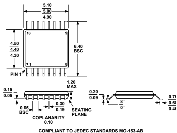
Figure 61. 16-Lead Thin Shrink Small Outline Package [TSSOP] (RU-16) Dimensions shown in millimeters
