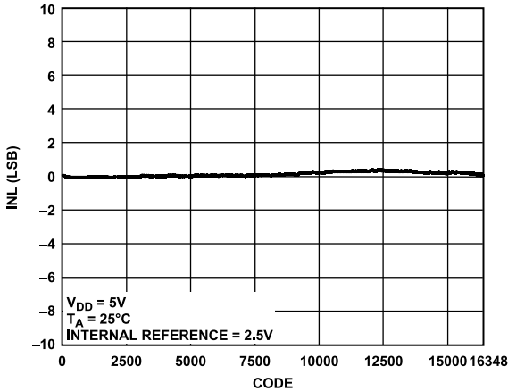
Figure 13. AD5695R INL
