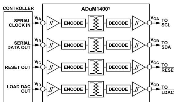
Figure 59. Isolated Interface
