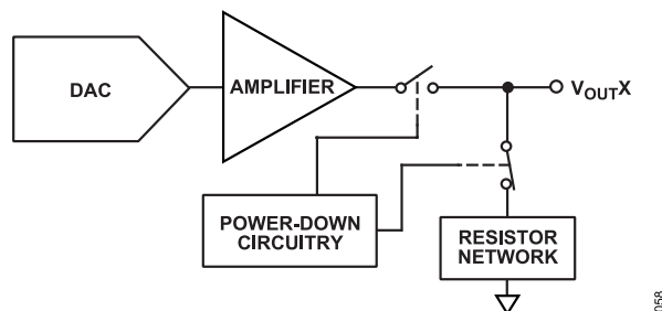
Figure 52. Output Stage During Power-Down
