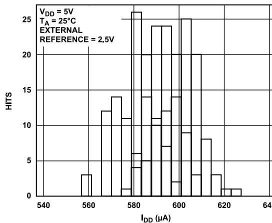
Figure 28. I_{DD} Histogram with External Reference, 5 V
