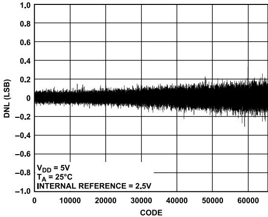
Figure 15. AD5696R DNL
