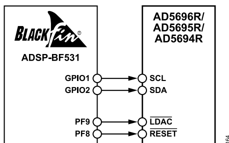
Figure 57. ADSP-BF531 Interface
