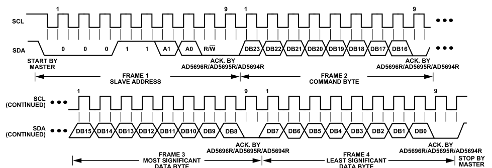
Figure 50. I²C Write Operation
