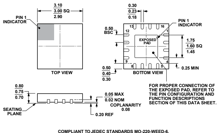
Figure 60. 16-Lead Lead Frame Chip Scale Package [LFCSP_WQ] 3 mm × 3 mm Body, Very Very Thin Quad (CP-16-22) Dimensions shown in millimeters
