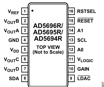
Figure 4. 16-Lead TSSOP Pin Configuration
