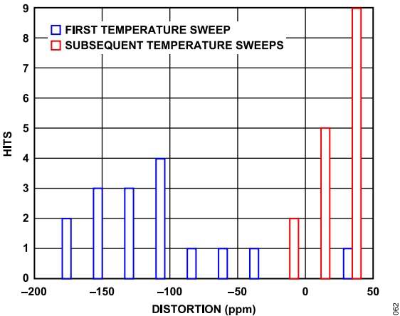
Figure 56. Thermal Hysteresis
