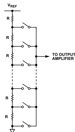
Figure 46. Resistor String Structure
