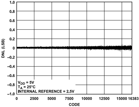
Figure 16. AD5695R DNL
