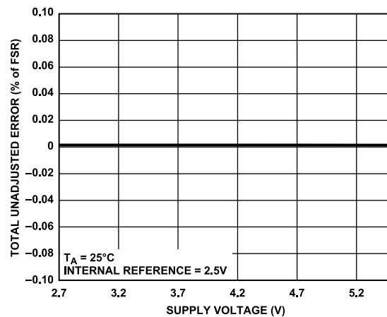
Figure 26. TUE vs. Supply, Gain = 1
