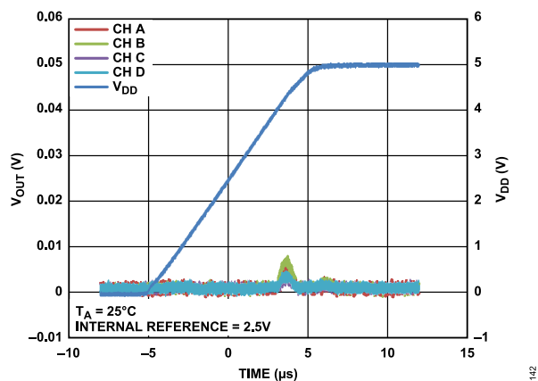
Figure 35. Power-On Reset to 0 V
