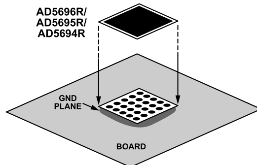
Figure 58. Paddle Connection to Board
