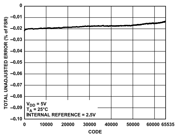
Figure 27. TUE vs. Code
