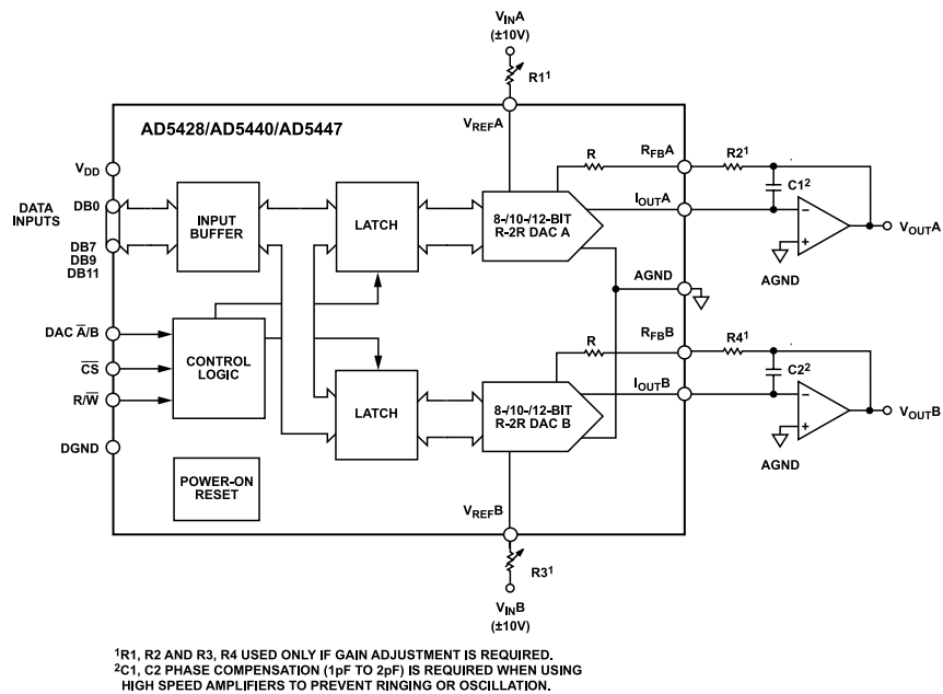
Figure 38. Unipolar Operation
