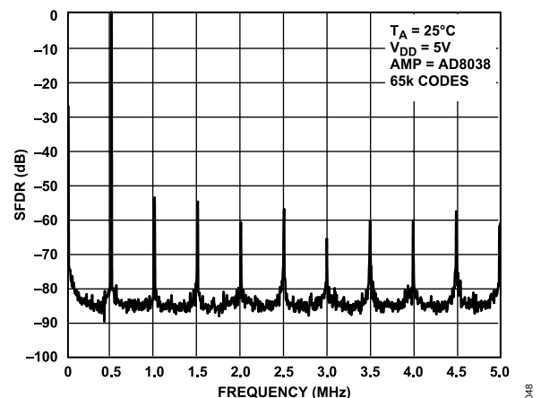
Figure 30. Wideband SFDR, f_{OUT} = 500 kHz, Clock = 10 MHz
