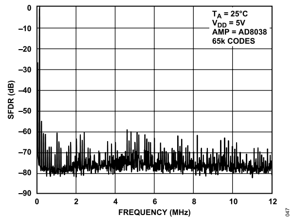
Figure 29. Wideband SFDR, f_{OUT} = 100 kHz, Clock = 25 MHz
