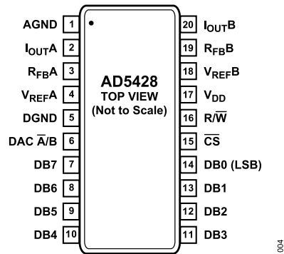
Figure 4. Pin Configuration 20-Lead TSSOP (RU-20)
