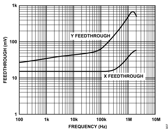
Figure 7. Feedthrough vs. Frequency
