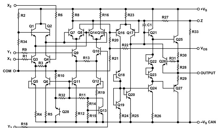
Figure 13. Schematic Diagram
