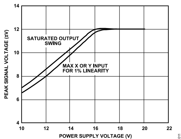
Figure 11. Signal Swing vs. Supply
