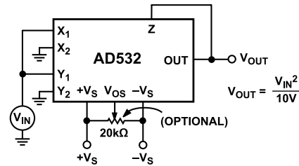
Figure 15. Squarer Connection
