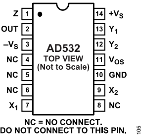
Figure 4. 14-Lead Side Brazed DIP (D-14)
