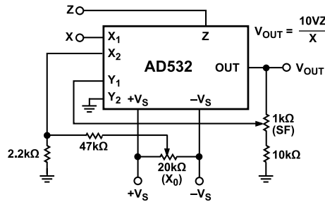
Figure 16. Divider Connection
