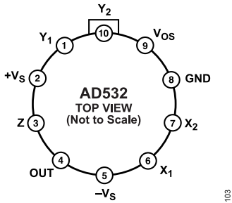
Figure 3. 10-Lead Header Pin Configuration (H-10)
