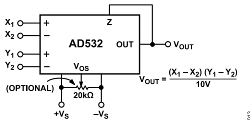
Figure 14. Multiplier Connection
