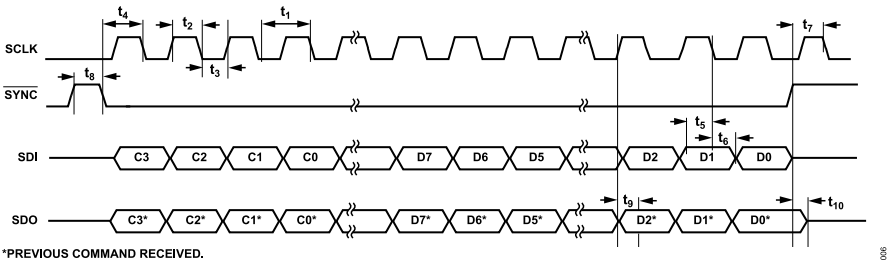
Figure 6. SPI Serial Interface Timing Diagram, CPOL = 0, CPHA = 1
