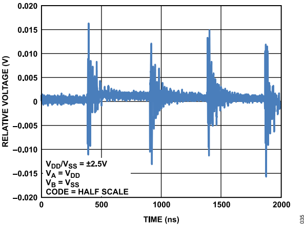
Figure 36. Digital Feedthrough
