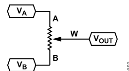
Figure 51. Potentiometer Mode Configuration
