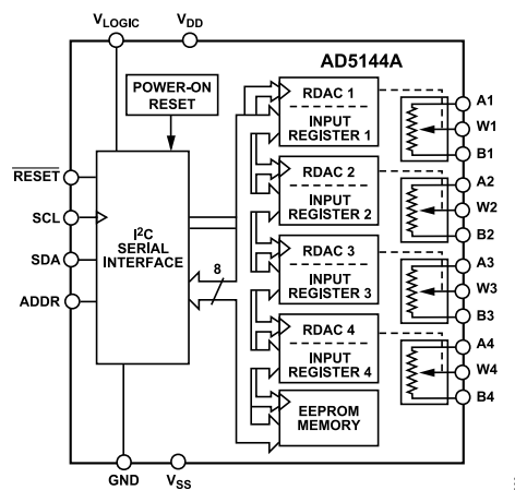
Figure 3. AD5144A 20-Lead TSSOP
