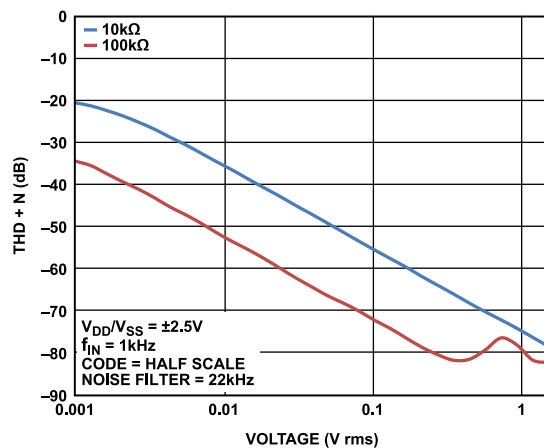
Figure 29. Total Harmonic Distortion Plus Noise (THD + N) vs. Amplitude
