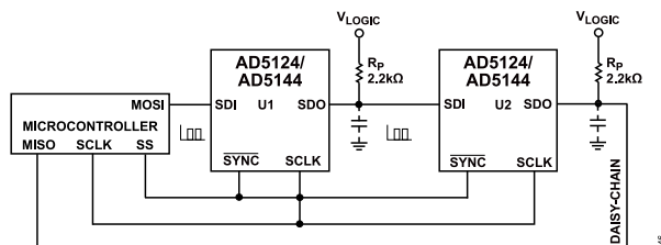
Figure 44. Daisy-Chain Configuration
