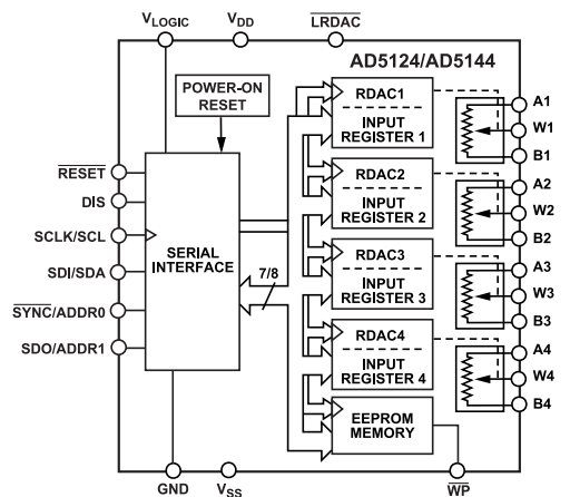
Figure 1. AD5124/AD5144 24-Lead LFCSP
