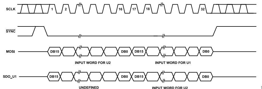
Figure 45. Daisy-Chain Diagram
