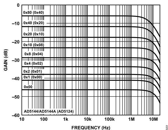
Figure 25. 10 \text{ k}\Omega Gain vs. Frequency vs. Code
