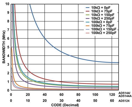
Figure 32. Maximum Bandwidth vs. Code vs. Net Capacitance
