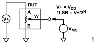
Figure 32. Potentiometer Divider Nonlinearity Error (INL, DNL)
