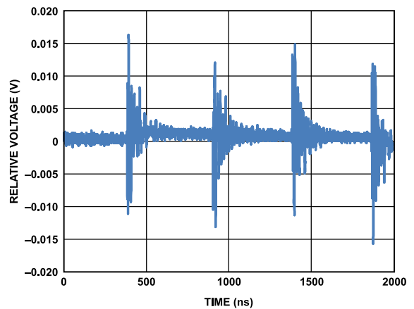
Figure 28. Digital Feedthrough
