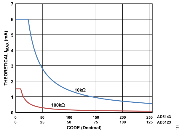
Figure 30. Theoretical Maximum Current vs. Code
