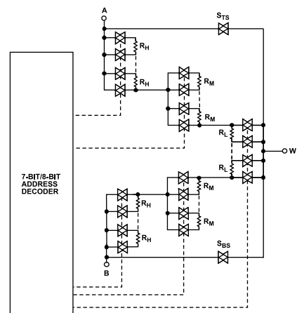
Figure 36. AD5123/AD5143 Simplified RDAC Circuit
