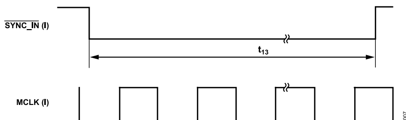
Figure 7. SYNC_IN Pulse Width
