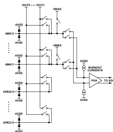
Figure 78. Excitation Current and Bias Voltage Connections
