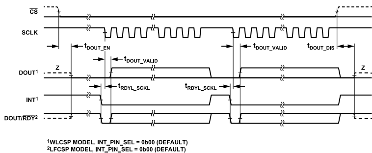
Figure 10. Continuous Read Mode Timing
