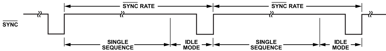
Figure 78. Example of Single Sequence + Idle by \overline{SYNC} Mode Diagram
