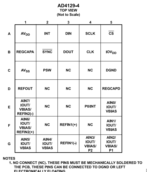
Figure 14. WLCSP Pin Configuration
