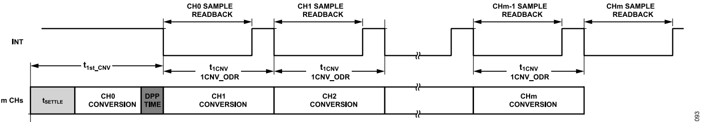
Figure 94. Example of Standard Sequencing Through Multiple Channels with Same Configuration and No Repeat Conversion
