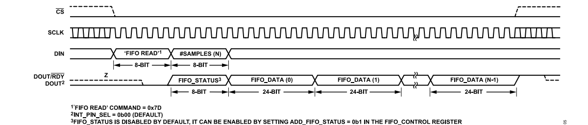
Figure 106. FIFO Readback (FIFO_STATUS Append On and FIFO_HEADER Append Off)
