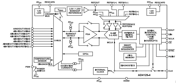
Figure 70. Detailed Block Diagram
