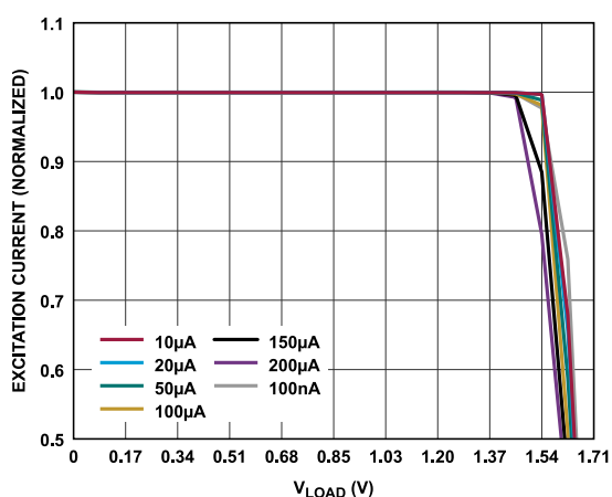
Figure 63. Output Compliance for Various IEXC Sources ( AV_{DD} = 1.71 V)
