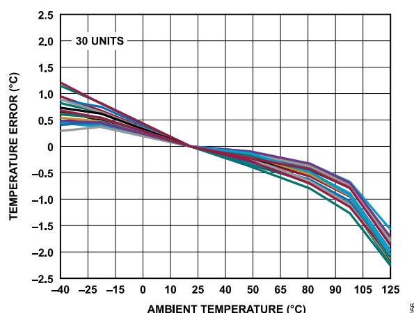
Figure 57. Temperature Sensor Error vs. Ambient Temperature after Calibration at 25°C
