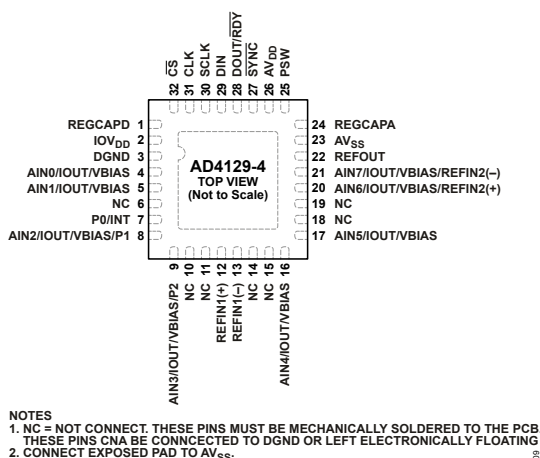
Figure 15. LFCSP Pin Configuration
