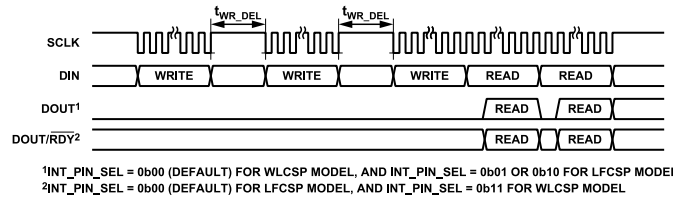
Figure 4. Delay Between Consecutive Serial Operations, 3-Wire Mode (CSB_EN Bit Set to 0), \overline{CS} Pin Tied Low
