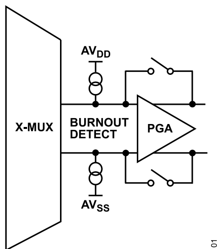
Figure 102. Burnout Currents
