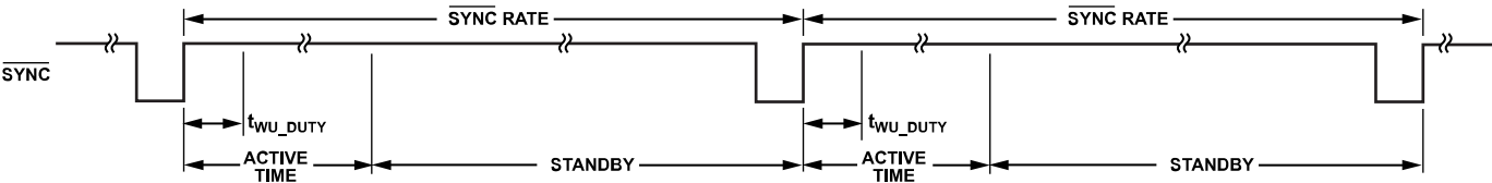
Figure 80. Example of Single Sequence + STBY by \overline{SYNC} Mode Diagram
