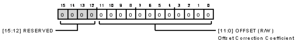
Figure 138. Offset Correction Register
