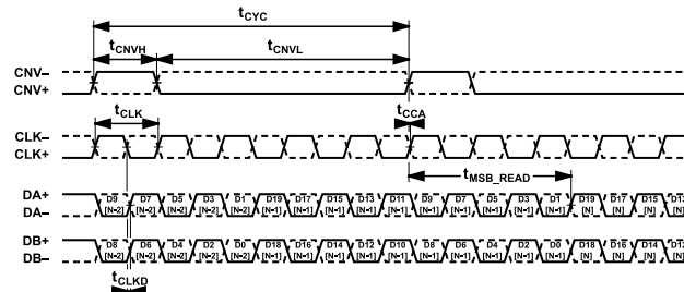
Figure 76. Continuous Conversion Timing, LVDS Data Interface, Single Data Lane, Self Clock Mode
