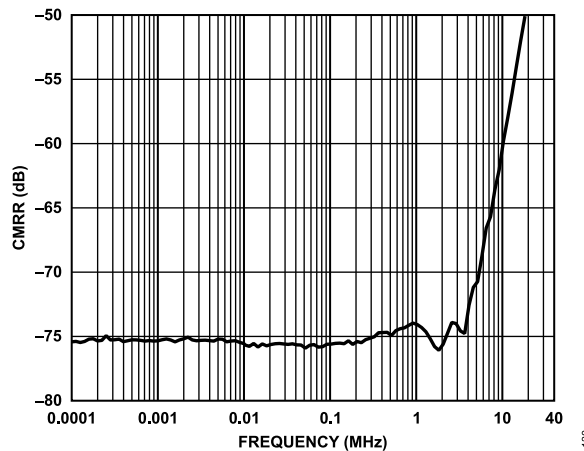
Figure 30. AC CMRR vs. Input Frequency
