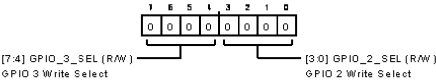
Figure 132. GPIO Configuration C Register
