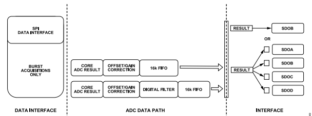
Figure 52. SPI Data Interface Data Path Options
