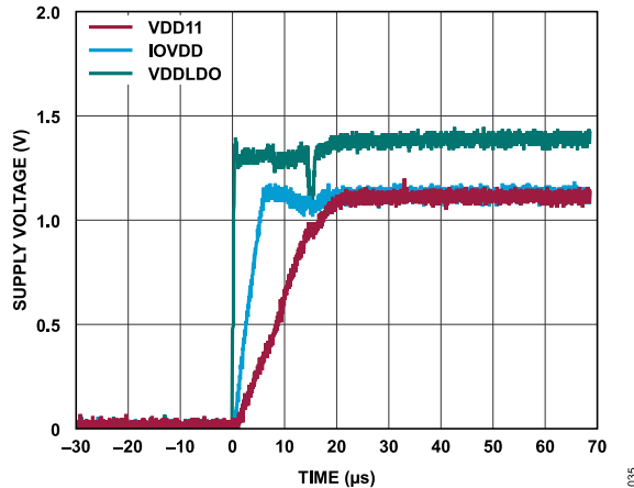
Figure 37. Typical Regulator Start-Up Transient, Converter Idle
