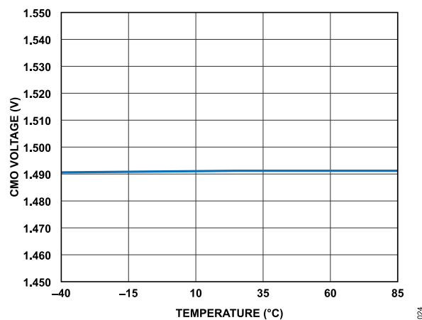
Figure 24. CMO Voltage vs. Temperature
