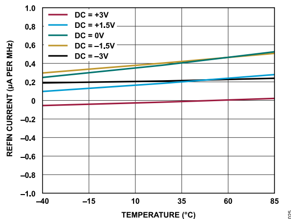
Figure 26. Dynamic REFIN Current vs. Temperature
