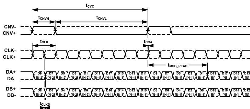
Figure 77. Continuous Conversion Timing, LVDS Data Interface, Dual Data Lane, Self Clock Mode
