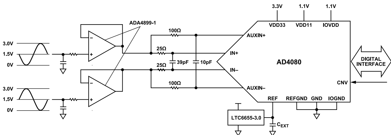
Figure 46. AD4080 Typical Applications Diagram, Single Op-Amp Drivers
