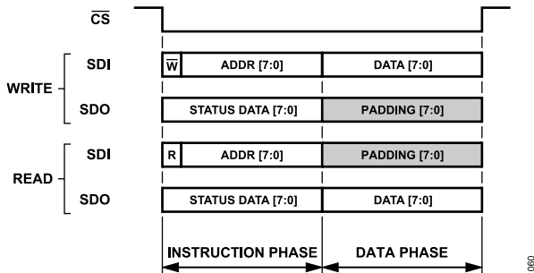
Figure 63. Short Instruction Mode, Data Status Enabled, CRC not Enabled
