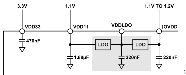
Figure 39. Externally Sourced Supply Configuration
