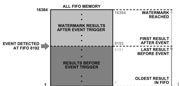
Figure 94. FIFO Event Capture Mode Read All FIFO Mode Example, Locating Event Position in FIFO
