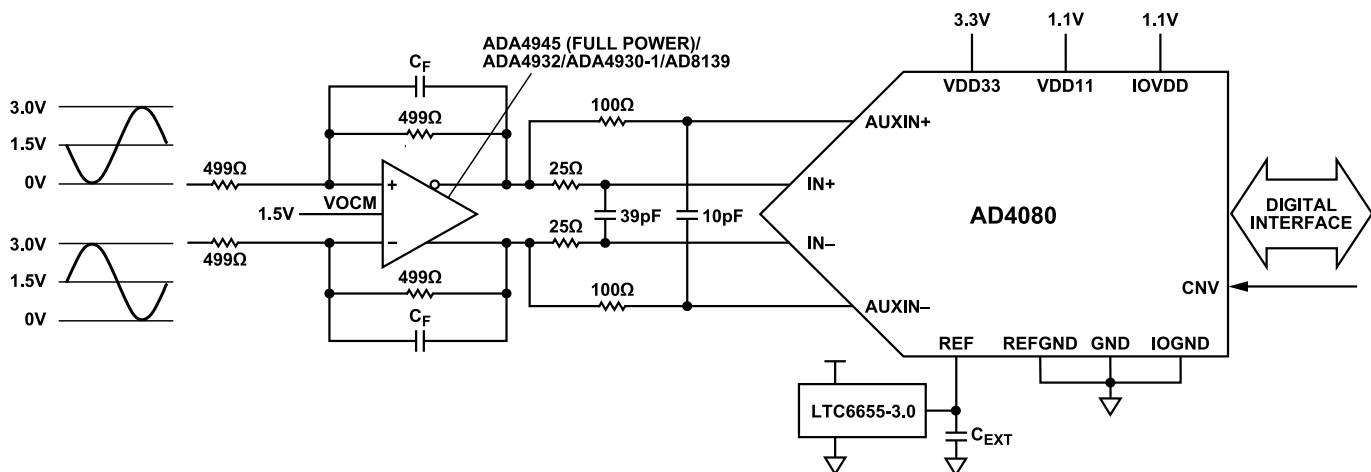
Figure 45. AD4080 Typical Applications Diagram, Fully Differential Amplifier
