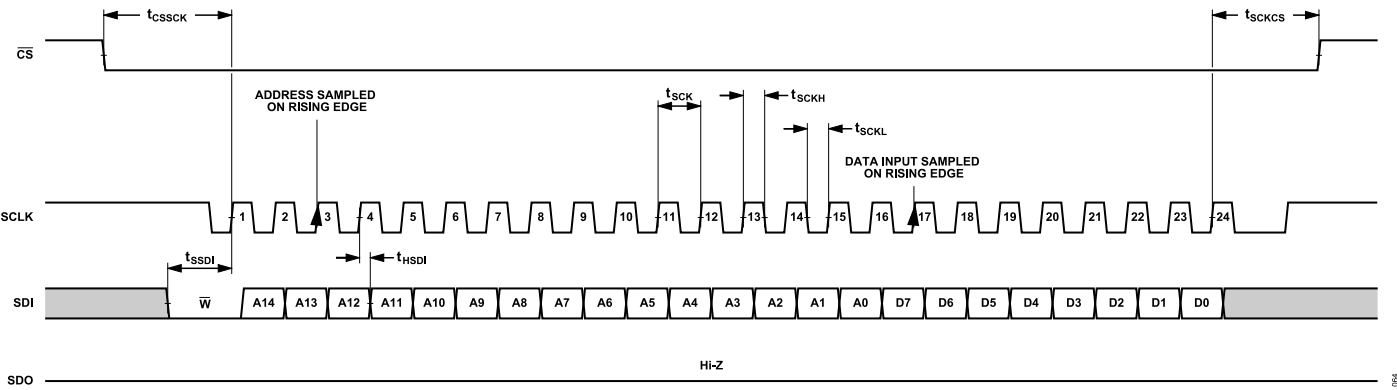
Figure 67. Configuration SPI Timing, Data Write Frame, 16-Bit Instruction Mode (Default)
