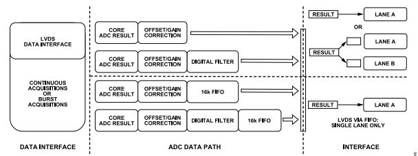
Figure 51. LVDS Data Interface Options
