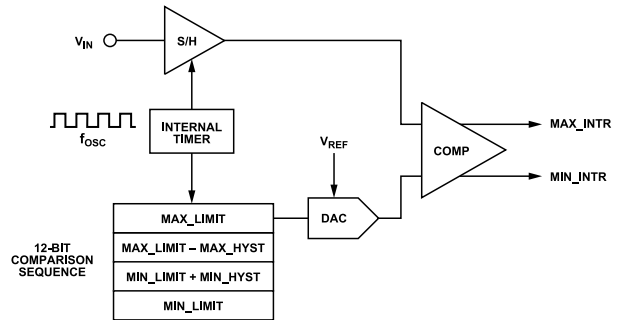
Figure 44. Simplified Schematic of Autonomous Mode Window Comparator
