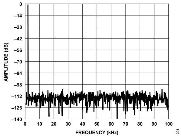
Figure 21. Fast Fourier Transform (FFT), f_S = 200\text{kSPS} , f_{IN} = 1\text{kHz}
