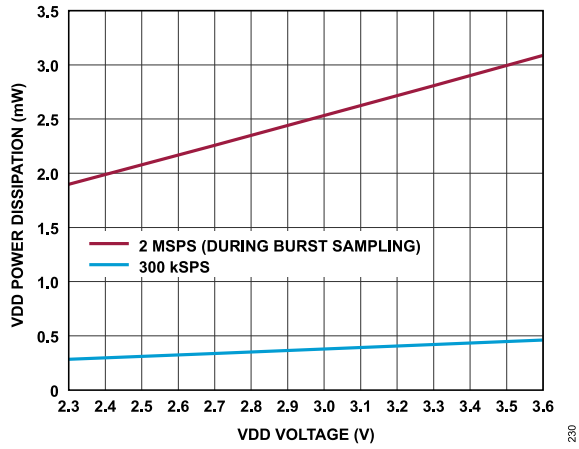
Figure 30. VDD Power Dissipation vs. VDD Voltage
