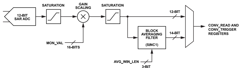
Figure 42. AD4060 Digital Processing Functionality
