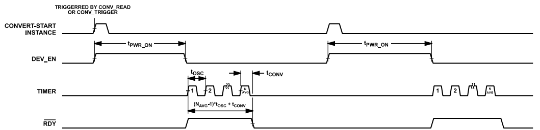
Figure 55. Burst Averaging Mode Timing with DEV_EN Enabled
