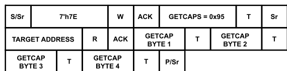
Figure 80. GETCAPS Direct Format
