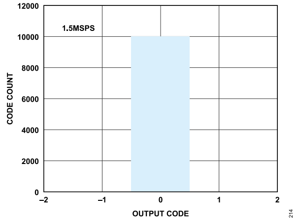
Figure 14. Histogram, Sample Mode (No Averaging)
