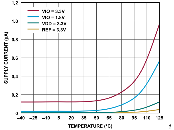
Figure 37. Supply Current (Sleep Mode) vs. Temperature
