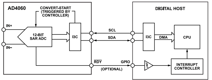
Figure 48. Sample Mode Example Connection Diagram
