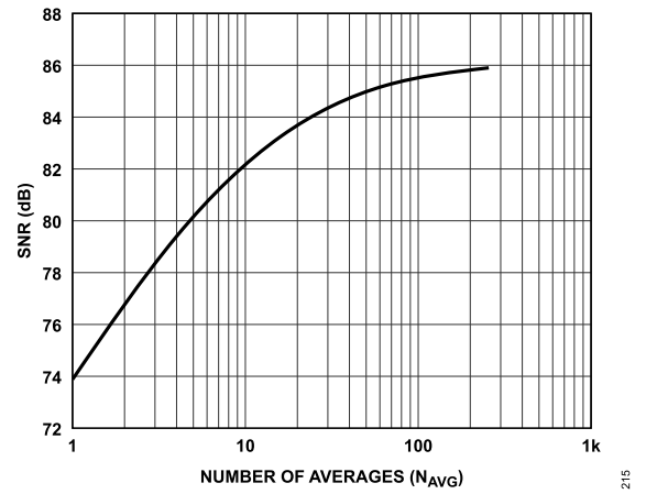
Figure 15. SNR vs. Number of Averages
