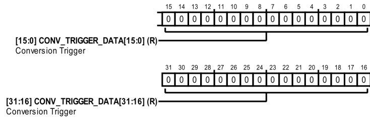
Figure 129. Address: 0x56, Reset: 0x00000000, Name: CONV_TRIGGER
