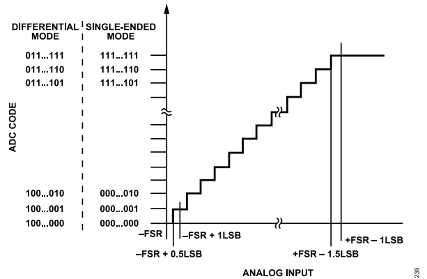
Figure 39. ADC Ideal Transfer Function
