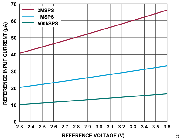
Figure 24. Reference Input Current vs. Reference Voltage
