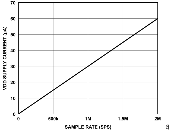
Figure 23. Reference Input Current vs. Sample Rate
