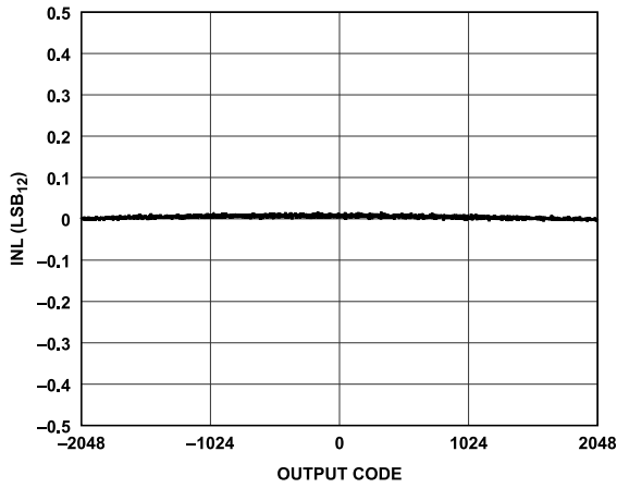
Figure 11. INL vs. Output Code
