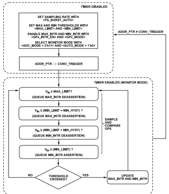
Figure 56. Monitor Mode Flowchart
