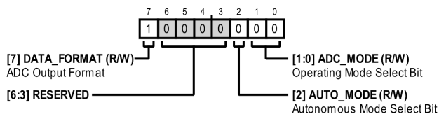
Figure 108. Address: 0x21, Reset: 0x80, Name: ADC_MODES
