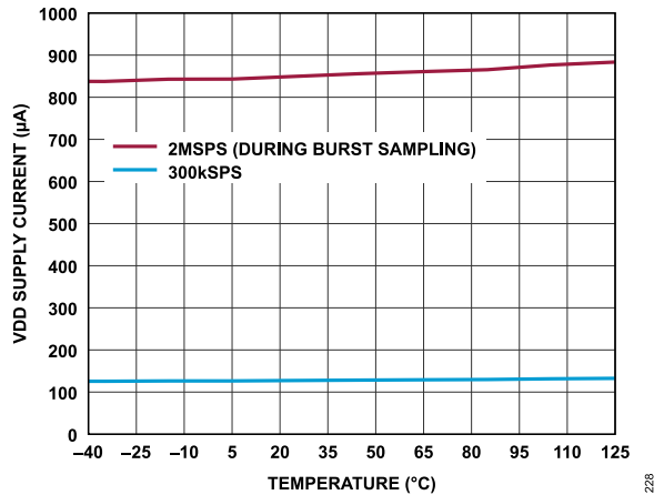
Figure 28. VDD Supply Current vs. Temperature
