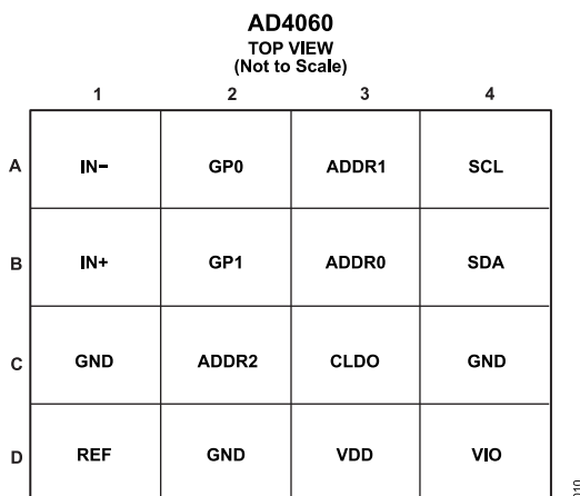
Figure 10. AD4060 WLCSP Pin Configuration
