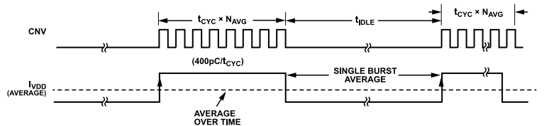
Figure 92. I_{DD} vs. Burst Conversions in Burst Averaging Mode
