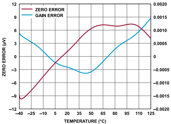
Figure 13. Zero Error and Gain Error vs. Temperature
