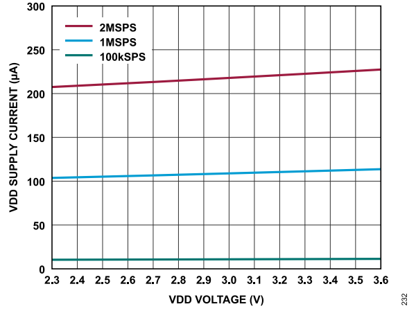
Figure 32. VDD Supply Current vs. VDD Voltage (Autonomous Modes)
