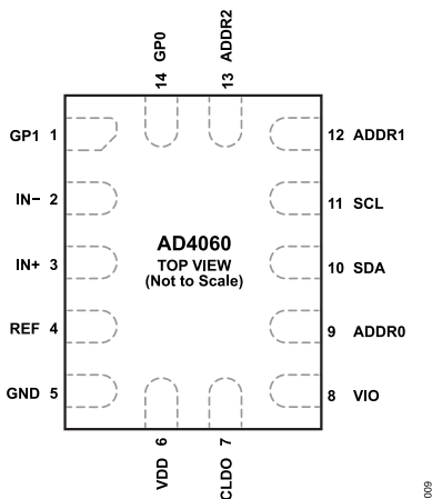
Figure 9. AD4060 LFCSP Pin Configuration
