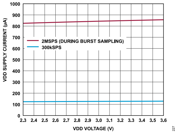
Figure 27. VDD Supply Current vs. VDD Voltage
