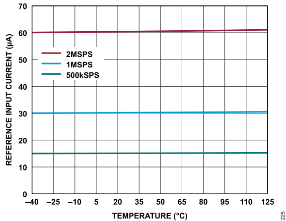
Figure 25. Reference Input Current vs. Temperature
