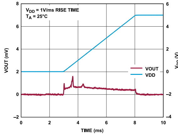
Figure 29. Power-On Reset to Tri-State Output
