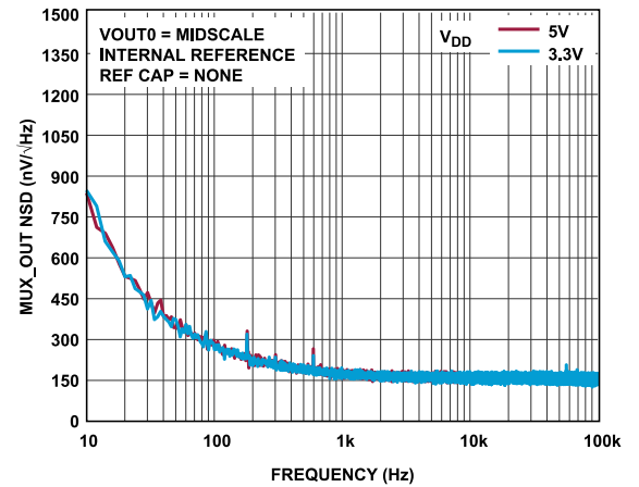
Figure 53. MUX_OUT NSD
