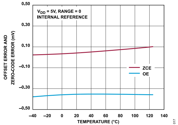
Figure 18. Offset Error and Zero-Code Error vs. Temperature
