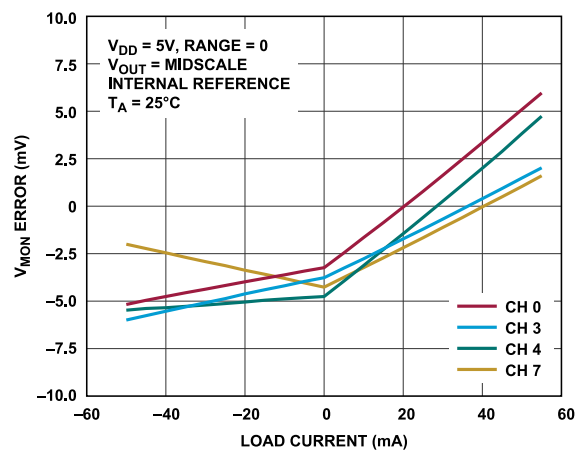
Figure 48. MUX_OUT V_{MON} Error vs. Output Current
