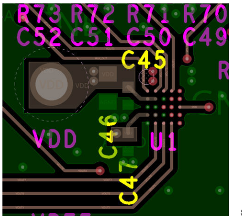
Figure 73. Evaluation Board Layout
