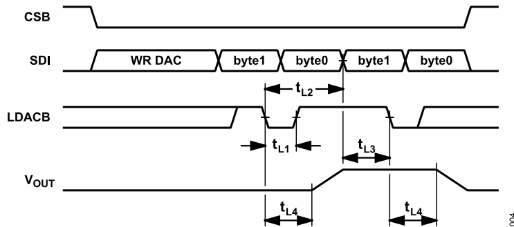
Figure 4. LDAC Timing
