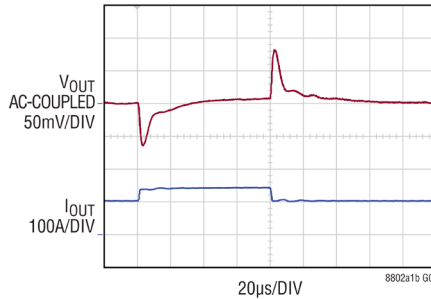
FIGURE 10 CIRCUIT V IN = 54V, V OUT = 3.3V, f SW = 813kHz C OUT = 680μF × 10 POSCAP + 100μF × 8 CERAMIC REG FE01h = 20, REG FE02h = 226, REG FE03h = 180, REG FE04h = 70
