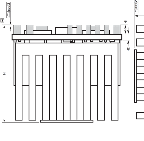
22-Terminal Printed Circuit Assembly [PCA] 22mm x 24mm x 22mm (PC-22-1)
