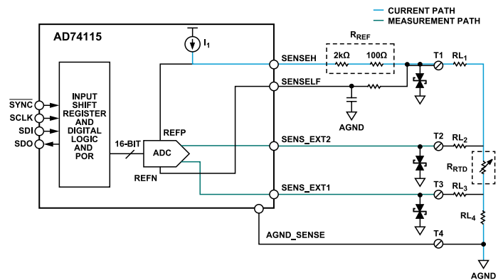
Figure 38. 4-Wire RTD Measurement Configuration
