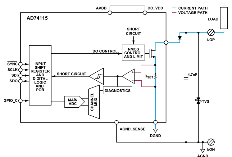
Figure 47. Digital Output Sinking Mode with the Internal FET
