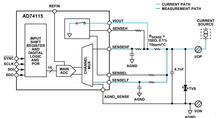
Figure 33. Current Input, Externally Powered Mode Configuration
