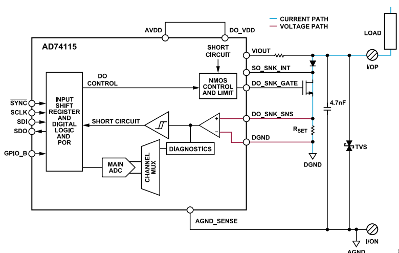
Figure 54. Configuration for Digital Output Sinking with FET Leakage Compensation
