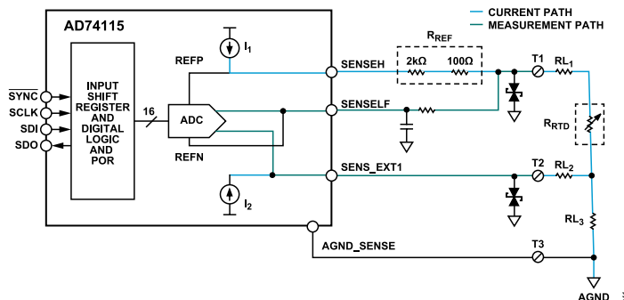
Figure 37. 3-Wire RTD Measurement Configuration
