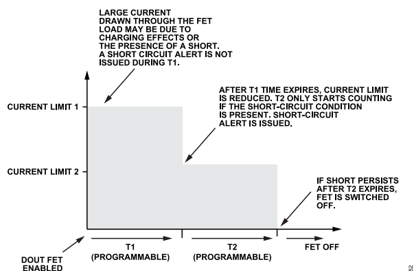
Figure 48. Digital Output Programmable Short-Circuit Control
