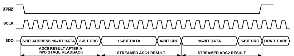
Figure 56. Burst Read Mode SDO Contents
