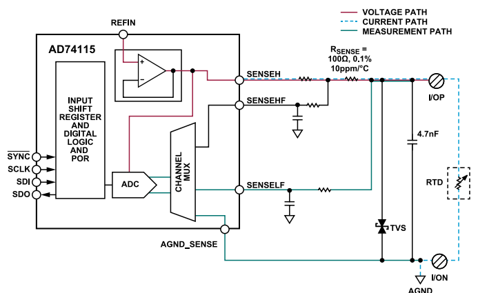
Figure 36. Resistance Measurement Configuration
