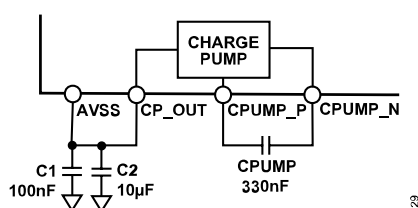
Figure 29. Charge Pump Configuration
