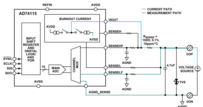
Figure 32. Voltage Input Mode Configuration
