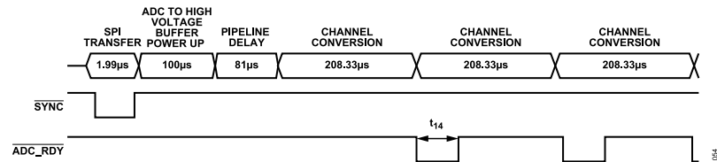
Figure 49. Single Measurement, Continuous Conversions Timing Diagram
