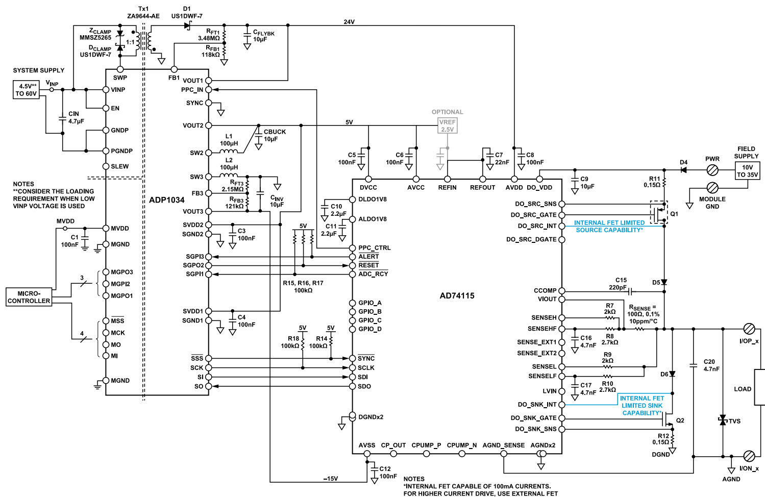
Figure 59. AD74115 and ADP1034 System Level Diagram
