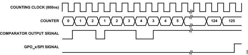
Figure 40. Digital Input Debounce Mode 0 Timing Example
