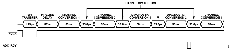
Figure 50. Multiple Measurements, Continuous Conversions Timing Diagram
