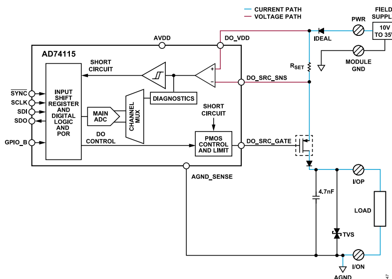
Figure 43. Digital Outputs Sourcing with External FET
