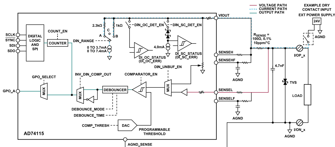
Figure 39. Digital Input Logic Mode Configuration
