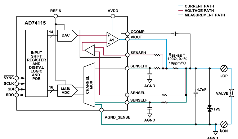
Figure 31. Current Output Mode Configuration
