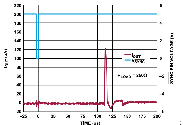
Figure 9. I_{OUT} and \overline{SYNC} Pin Voltage ( V_{\overline{SYNC}} ) vs. Time on Current Output Enable
