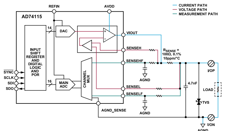
Figure 34. Current Input, Loop Powered Mode Configuration
