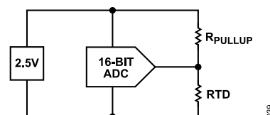
Figure 35. RTD Bias Circuit
