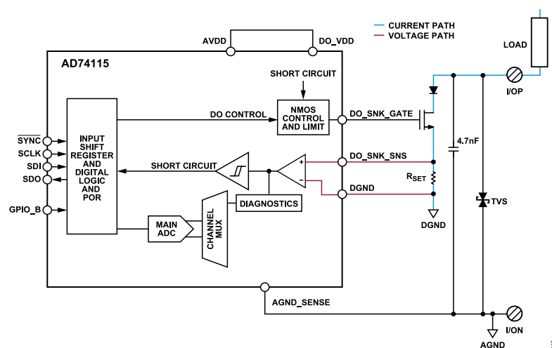
Figure 44. Digital Output Sinking with External FET
