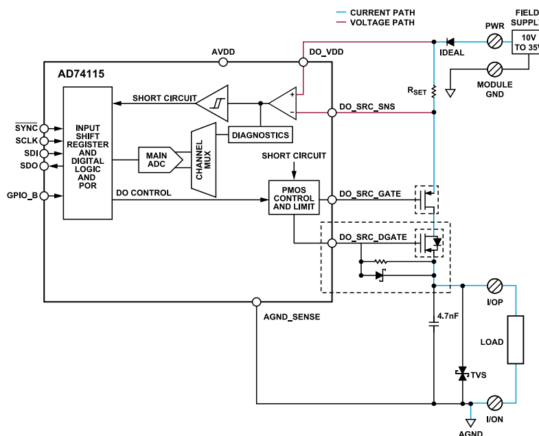
Figure 45. Smart Diode Configuration for Current Sourcing with an External FET
