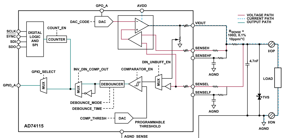
Figure 42. Digital Input, Loop Powered Configuration Mode
