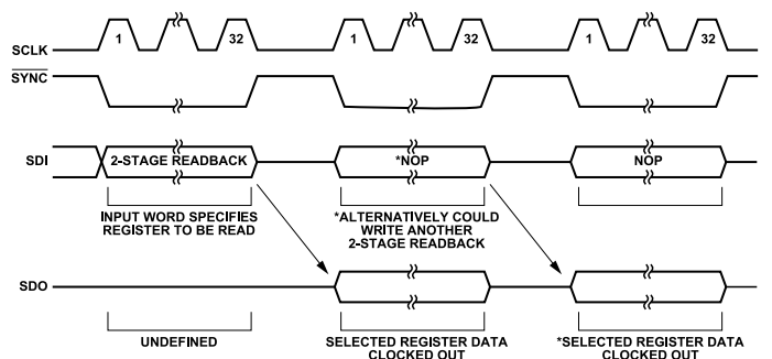
Figure 55. 2-Stage Readback Timing Diagram
