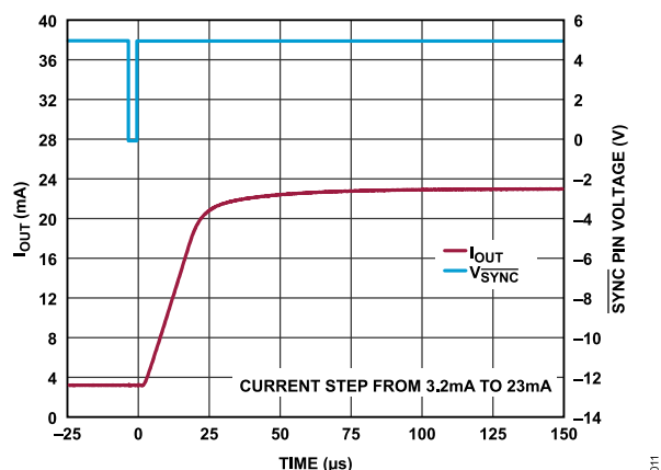
Figure 10. I_{OUT} and \overline{SYNC} Pin Voltage ( V_{\overline{SYNC}} ) vs. Time
