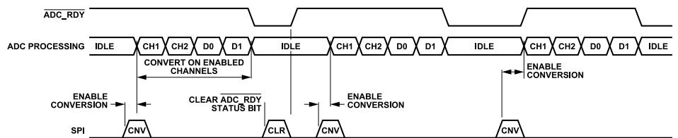
Figure 51. \overline{\text{ADC\_RDY}} Functionality in Single Conversion Mode
