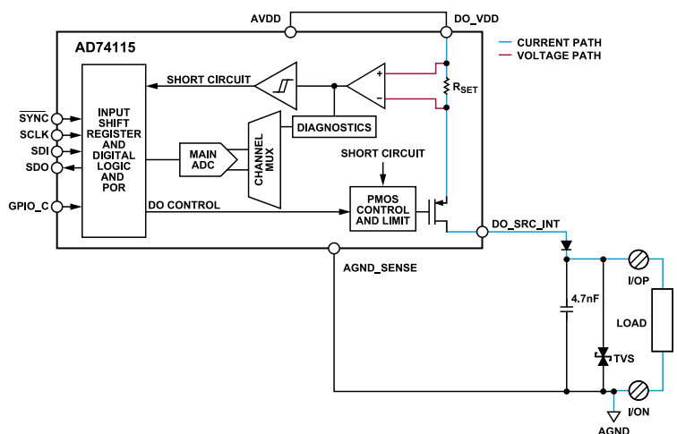
Figure 46. Digital Output Sourcing Mode with the Internal FET
