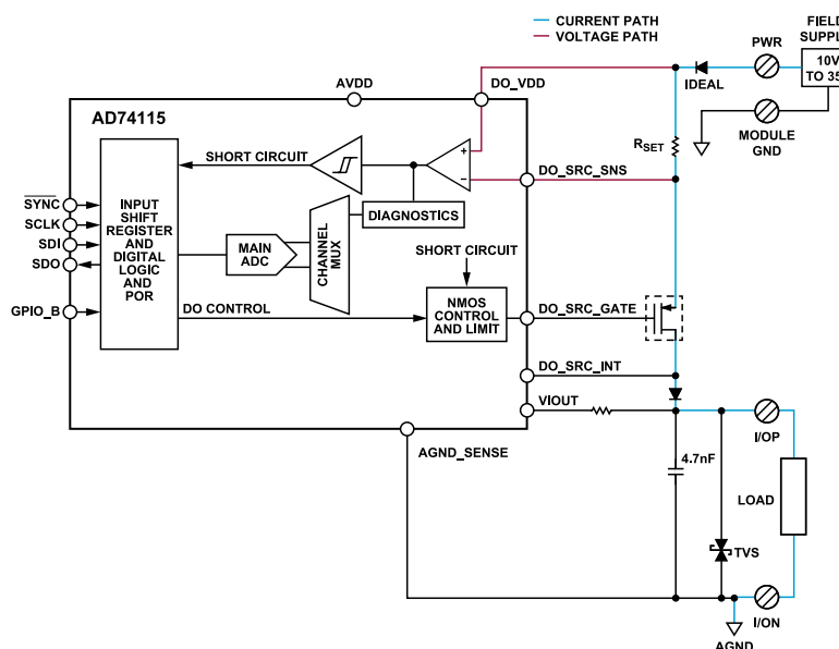
Figure 53. Configuration for Digital Output Sourcing with FET Leakage Compensation
