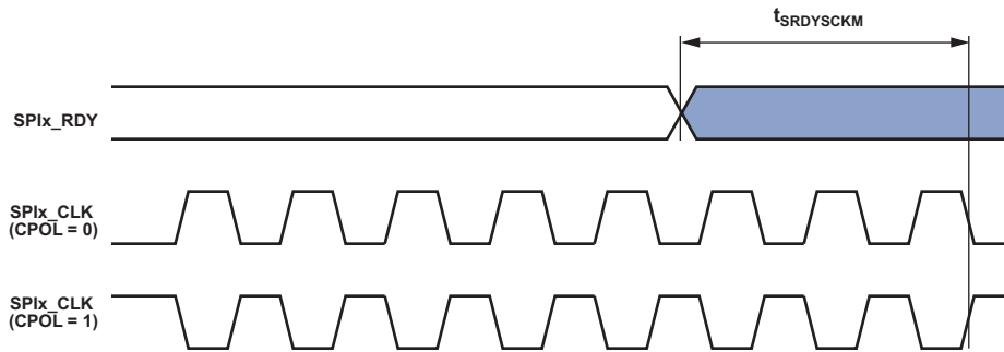
Figure 20. SPI x _RDY Setup Before SPI x _CLK
