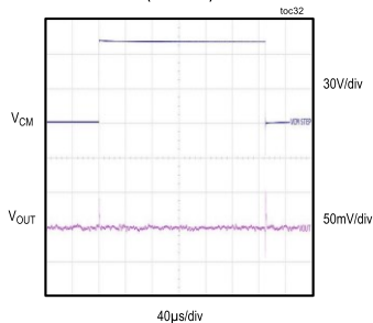
COMMON-MODE VOLTAGE STEP (0 TO 70V)
