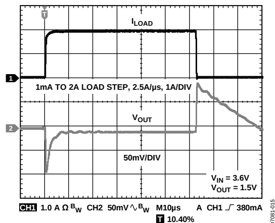
图15. 负载瞬态响应( C_{\text{IN}} = 4.7\text{ }\mu\text{F} , C_{\text{OUT}} = 4.7\text{ }\mu\text{F} )
