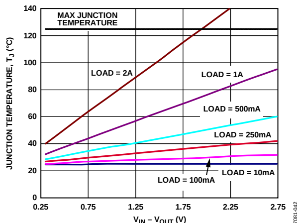
图44. 1000 mm 2 PCB覆铜, T_B = 25^\circ\text{C} , LFCSP
