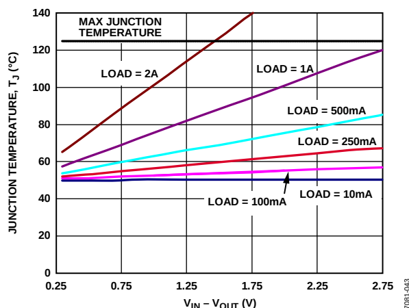
图45. 1000 mm 2 PCB覆铜, T_B = 50^\circ\text{C} , LFCSP
