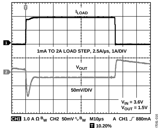
图16. 负载瞬态响应( C_{\text{IN}} = 22\text{ }\mu\text{F} , C_{\text{OUT}} = 22\text{ }\mu\text{F} )
