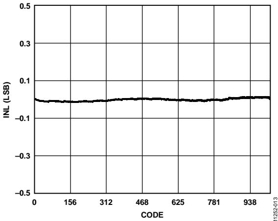
图12. 积分非线性(INL)
